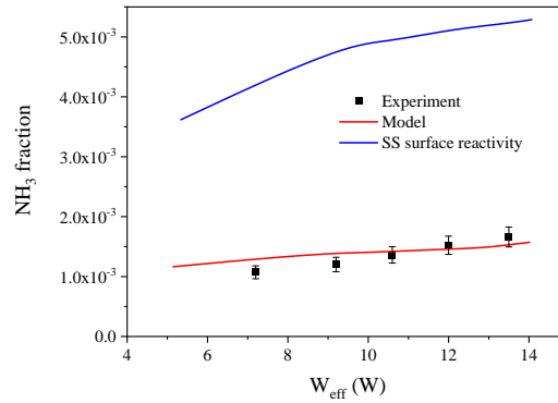
Figure 11. Simulations (curves) and measurements (points) of the \text{NH}_3 fraction, as a function of the power coupled, for the same conditions as in Figure 10. Simulations used the wall loss probabilities provided in Table A1 (red line) or the values for a stainless-steel surface proposed in [47] (blue line).
