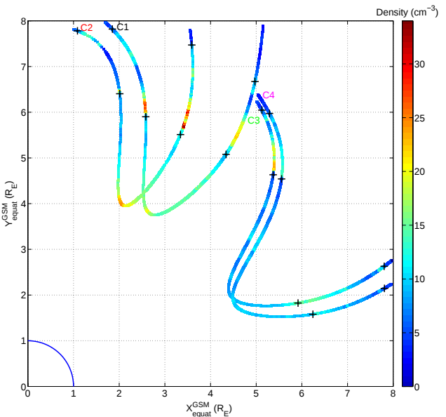
Fig. 5. Electron density plotted along the trajectories of C1, C2, C3 and C4 projected along the magnetic field lines onto the equatorial plane in a co-rotating geocentric solar magnetospheric (GSM) frame of reference (chosen such that C4 was at 15:30 MLT at 18:00 UT), during the plasmasphere pass on 18 July 2005. The density is plotted with the color scale on the right. The crosses show the times of the plume crossings T_{inner} and T_{outer} indicated in Table 1.
