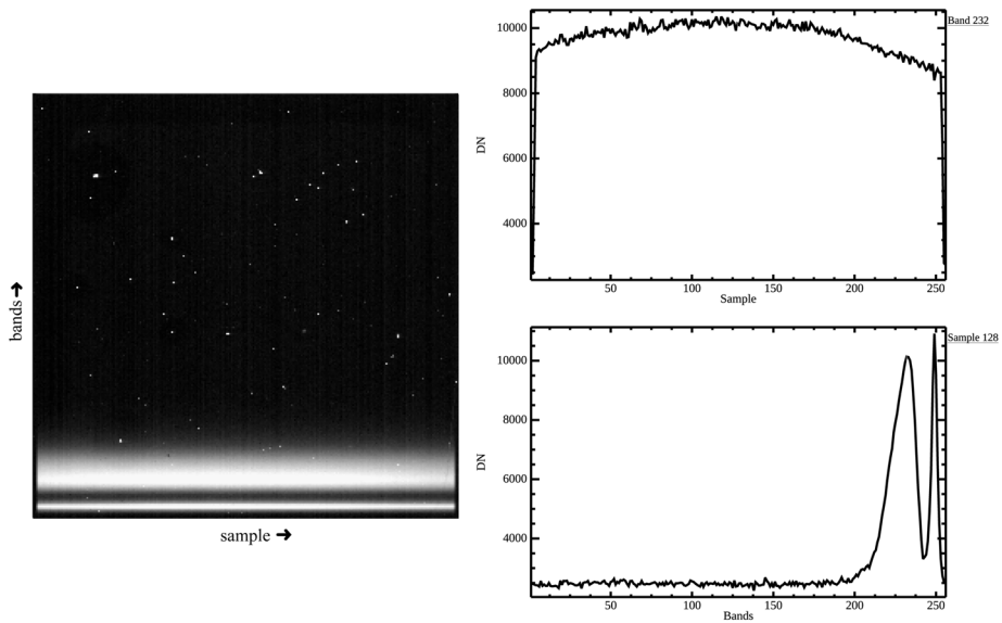
Fig. 38 The VIHI internal calibration LED source signal measured during commissioning: the signal on the detector frame (left, spectral information along the vertical direction and spatial information along the horizontal direction) and the spatial variability across the FoV (top right) and the spectrum (bottom right) from 400 nm (band 255) to 2000 nm (band 0)
