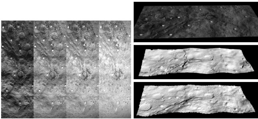
Fig. 22 The effect of four different illumination conditions for the anorthosite sample (left), with incidence angles of 10^\circ , 30^\circ , 50^\circ , and 70^\circ from left to right. The image obtained by one STC channel of the anorthosite target (top right), the photogrammetric DTM (middle right), and the DTM generated by the laser scanner (bottom right)
