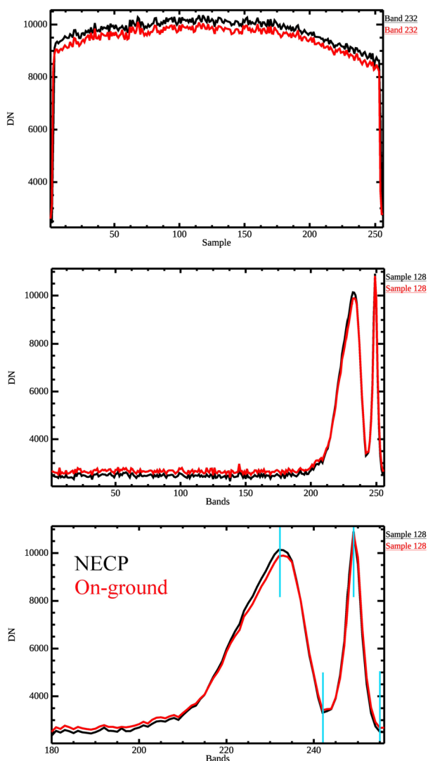
Fig. 39 Comparison between the VIHI internal calibration LED source signal measured during commissioning (black lines) and in on-ground tests (red lines). Spatial variability across the FoV (top) and the spectrum (middle) from 400 nm (band 255) to 2000 nm (band 0), as well as a spectral profile zoom showing the emission peaks of the LED as compared to the ground measurements (bottom)
