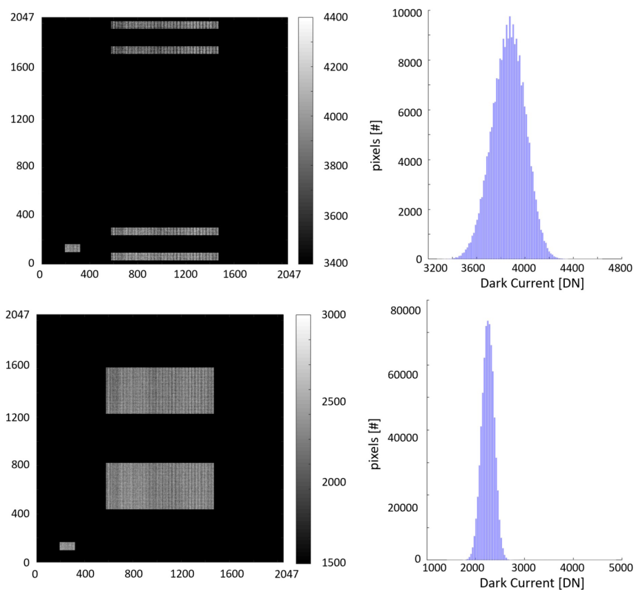
Fig. 35 Two examples of acquisition for STC during the NECP: the global mapping mode (top) and the color mode (bottom). The STC detector is shown on the left and the dark signal distribution on the right. In both cases, the histogram has a width around 800 DN corresponding to a foreseen standard deviation of 135 DN
