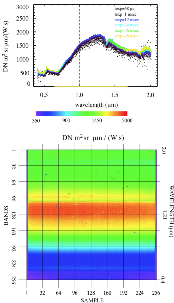
Fig. 27 The VIHI responsivity at sample = 128 (top) for integration times between 68 \mu s and 48 ms and the VIHI responsivity array (bottom) as derived for the integration time t = 10 ms. From Filacchione et al. (2017)
