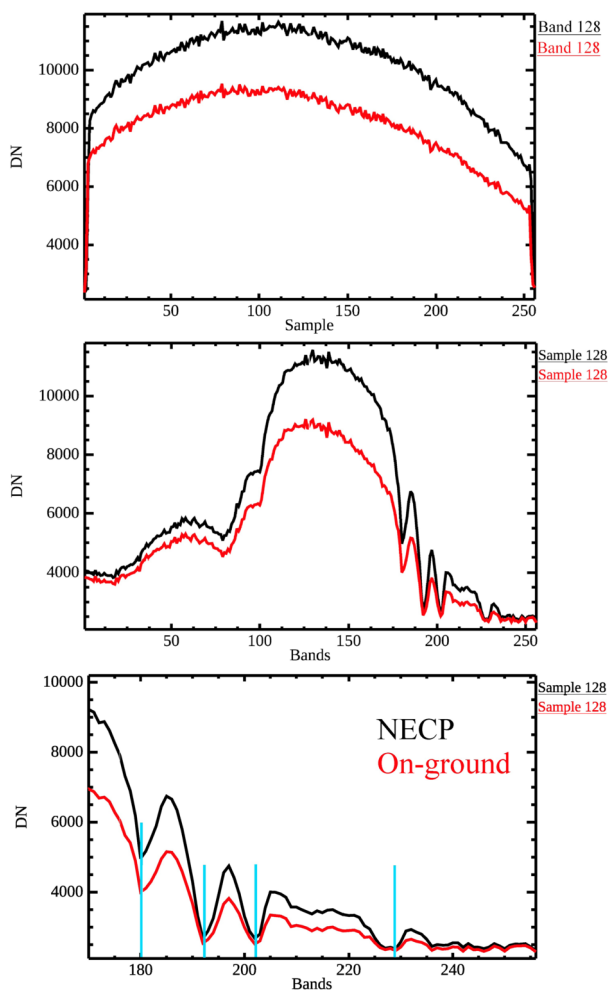
Fig. 37 The VIHI spectral response verification. The comparisons between the NECP tests (top and middle, black lines) and the on-ground ones (red lines). The two profiles show spatial variability (top) across the FoV and the spectrum (central), from 400 nm (band 255) to 2000 nm (band 0). A spectral profile zoom above the constant position of the Didymium filter absorption bands is also shown before and after launch (bottom)
