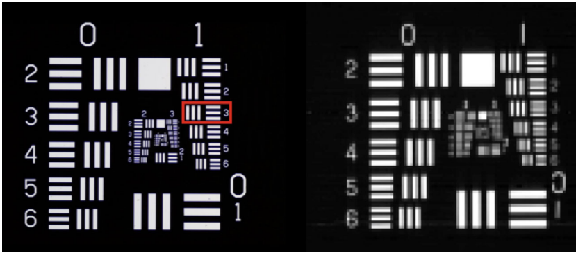
Fig. 25 USAF mask 1951 reference image (left). The pattern G = 1 , E = 3 indicated by the red box corresponds to the VIHI theoretical frequency f_{Nyquist} = 2.52 lines/mm. VIHI image of the mask (right) at wavelength \lambda = 590 nm. The VIHI slit (sample direction) is oriented towards the vertical axis and the image is acquired in time by scanning at one IFoV step along the horizontal axis. From Filacchione et al. (2017)
