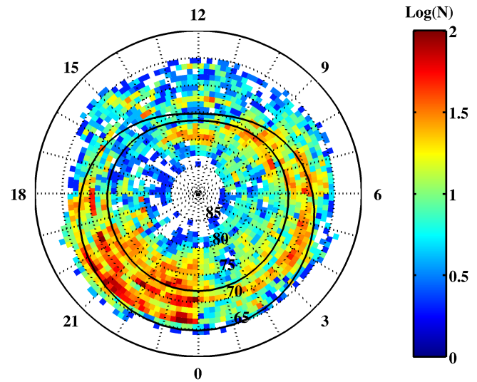
Fig. 1. Spatial distribution of the occurrence of radar echoes in our database, in MLT/ \Delta (Invariant Magnetic Latitude) AACGM coordinates. The occurrence is colour-coded on a logarithmic scale. The boundaries of the auroral oval, defined by Holzworth and Meng (1975) for a moderate geomagnetic activity ( 3 < K_p < 4^- ) are overlaid.
