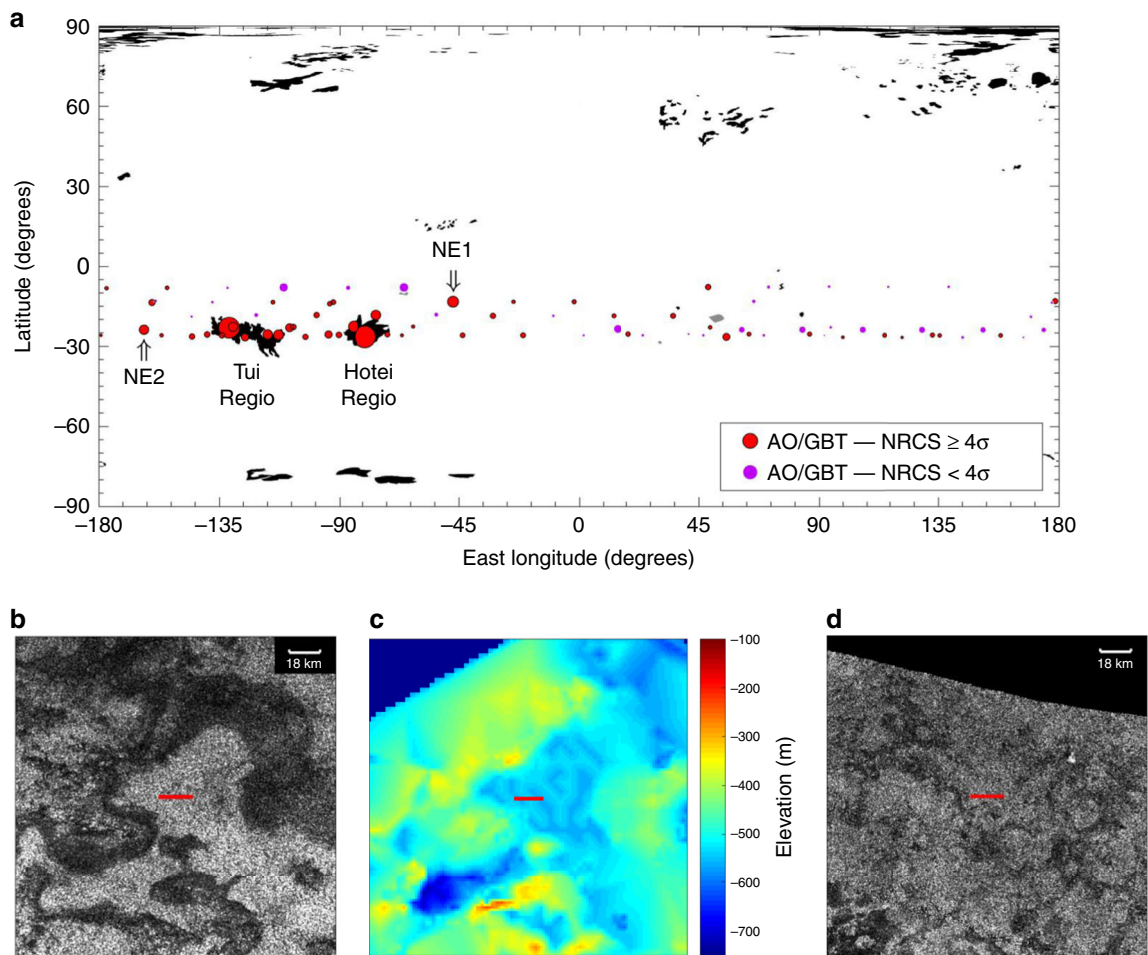
Fig. 4 Hotei and Tui Regions. a Black areas are Titan's 5- \mu m-bright regions as mapped in MacKenzie et al. 24 . Hotei and Tui Regions are the 5- \mu m-bright regions at \approx 80^\circ W, 25^\circ S and \approx 120^\circ W, 25^\circ S. AO/GBT observations are plotted as in Fig. 2. Hotei and Tui Regions are the main source of the AO/GBT anomalously specular reflections. Two noteworthy exceptions to the strong correlation of anomalously specular AO/GBT observations to Hotei/Tui are labeled NE1 and NE2 and discussed in the Discussion section. b The 18-km subradar track (red line) of the highest maximum-NRCS (and most specular in Black et al. 2 ) AO/GBT observation, located in Hotei Region (largest red dot in Hotei Region in a ). c The stereo topography of the same area 37 . The AO/GBT reflection is from a bright area that is morphologically similar to paleolakes 25 ( b ) and is topographically low ( c ). d The 18-km subradar track (red line) of the second highest maximum-NRCS (and second most specular in Black et al. 2 ) AO/GBT observation, located in Tui Region (largest red dot in Tui Region in a ). The AO/GBT reflection is again from a bright area that is morphologically similar to the comparably specular location in Hotei Region and paleolakes. Stereo topography does not cover this track.
