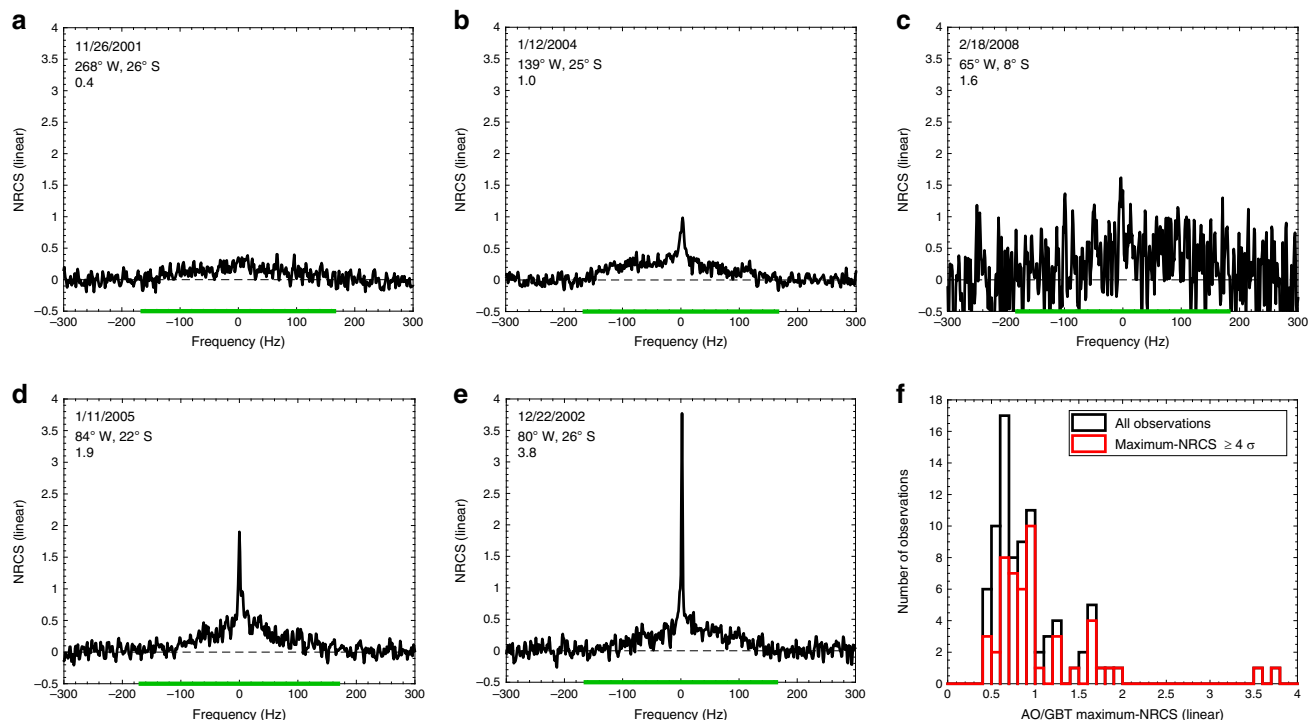
Fig. 1 Arecibo Observatory and Green Bank Telescope observations of Saturn's moon Titan. a–e Example AO/GBT echo spectra of Titan in the opposite circular polarization channel, adapted from Black et al. 2 . The observation date, subradar location on Titan, and maximum-NRCS are in the panel legends. The width of the echo from Titan is indicated by the green line on the x-axis; data beyond the green line are indicative of the noise. All AO/GBT spectra from Titan have a broad, diffuse component with an NRCS of approximately zero at the limits of the echo (endpoints of the green line on the x-axis) that increases toward the center. The NRCS of the central Doppler bin varies drastically between the spectra. Observations with anomalously high peaks (e.g., d and e ) are the AO/GBT anomalously specular radar reflections. c Example demonstrating that the maximum-NRCS of some observations may be affected by noise. f Histograms of the maximum-NRCS of AO/GBT observations of Titan reported in Black et al. 2 . The black histogram includes all 83 observations and the red histogram includes only observations where the maximum-NRCS is \geq 4 times the standard deviation of the noise ( \sigma ), to distinguish between observations with a high maximum-NRCS that may be due to greater noise and those that are confidently anomalous. Two observations have a maximum-NRCS \geq 3.5 and are clearly separate from the distribution and thus anomalously specular. Another group of observations, with 1.5 \approx maximum-NRCS \leq 2 , is also separate from most observations; these observations are also anomalously specular, albeit less so than the two observations with maximum-NRCS \geq 3.5 .
