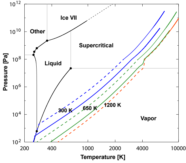
FIG. 1.— Pressure and temperature profiles of hydrospheres of 1 and 15 M_{\oplus} supercritical ocean planets fully constituted of water with equilibrium temperatures of 300, 650, and 1200 K superimposed onto the water phase diagram. Colored solid and dashed curves correspond to 1 and 15 M_{\oplus} planets, respectively. The black dashed line delimits a hypothetical transition between the supercritical phase and high pressure ice (see text). Dashed lines change to solid lines when the interior model takes over from the atmosphere model. The 1 M_{\oplus} case with an equilibrium temperature of 1200 K is removed because its atmosphere is hydrostatically unstable (see Fig. 2).
