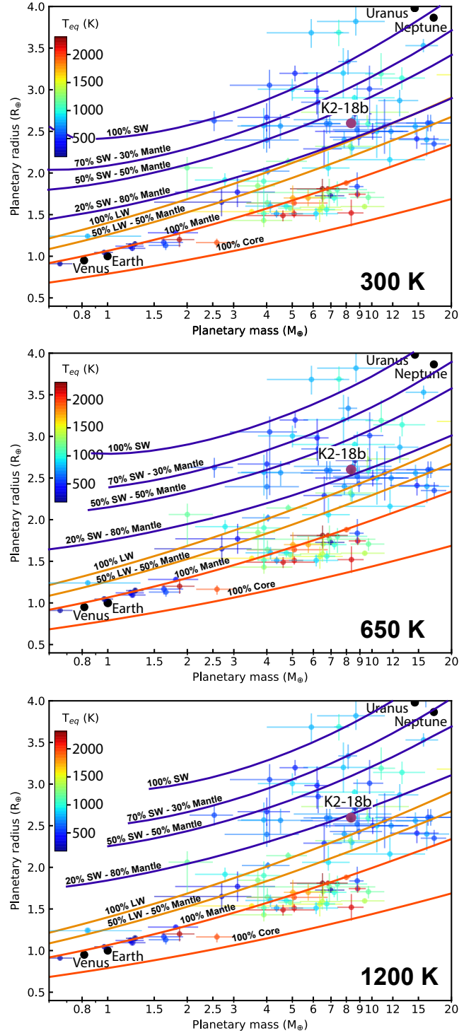
FIG. 2.— Mass-radius diagrams determined for exoplanets with masses in the 0.6–20 M_{\oplus} range, and equilibrium temperatures of 300 K, 650 K, and 1200 K. Mass-radius curves are calculated for several planetary compositions: 100% core and 100% mantle (red curves), liquid water (LW) hydrosphere (brown curves) and supercritical water (SW) hydrosphere (blue curves) topping mantle-like composition interiors. Planetary data are taken from the NASA exoplanet archive and updated to 20th July 2019. Hydrostatically unstable atmospheres (defined when the altitude at 0.1 Pa tends towards infinity) around the hotter and smaller planets are excluded from the mass-radius relationships.
