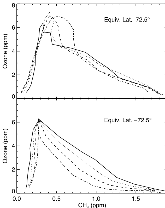
Figure 2. Similar to Figure 1 but for the polar regions in winter and spring. Methane-ozone relation at (top) 72.5°N and (bottom) -72.5°N. In Figure 2 (top), the solid line shows data for January, the dotted line shows data for February, the dashed line shows data for March, and the dash-dotted line shows data for April. In Figure 2 (bottom), the solid line shows data for June, the dotted line shows data for July, the dashed lines show data for August, and dash-dotted line shows data for September.
