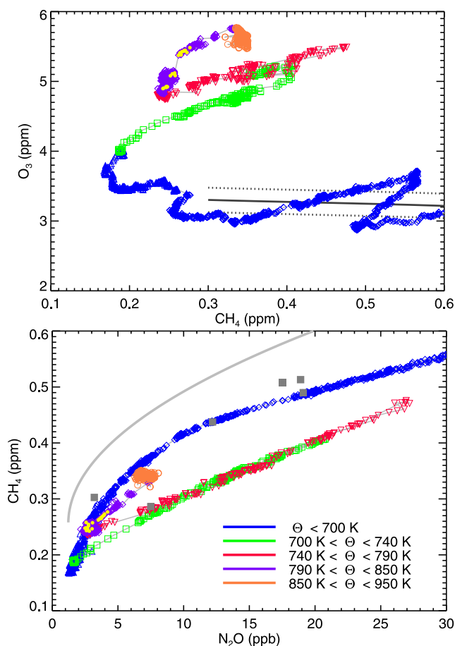
Figure 4. (top) Ozone-methane and (bottom) methane- N_2O relation from the SPIRALE measurements on 21 January 2003. The measurements are color coded according to altitude as in Figure 3 (color legend in Figure 4, bottom). Air masses that are most strongly influenced by mesospheric air (CO ranging between 570 and 584 ppb) are marked by solid yellow circles. Gray squares in Figure 4 (bottom) show the BONBON measurements on 6 March 2003 that are not influenced by mesospheric air. The gray solid line in Figure 4 (bottom) indicates the methane- N_2O relation for midlatitudes reported by Michelsen et al. [1998] adjusted to 2003 conditions by increasing N_2O by 2.3% and CH_4 by 3.2%. The black solid line in Figure 4 (top) shows an early vortex reference deduced from MkIV measurements on 16 December 2002 [ Tilmes , 2004], and dotted lines show the uncertainty of the reference.
