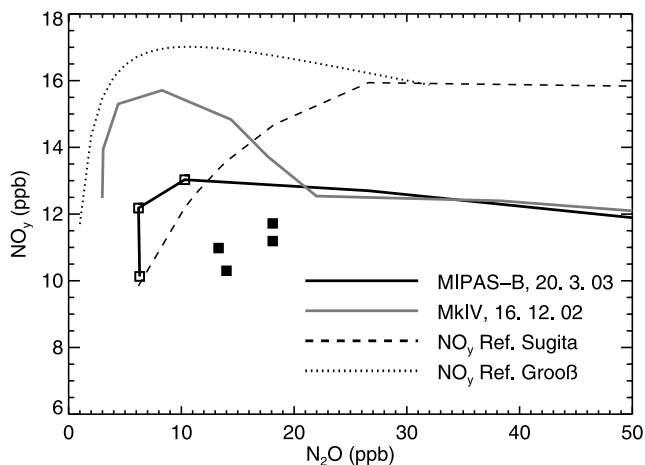
Figure 5. Relation of NO_y and N_2O (thick black line and squares) from the MIPAS-B measurements on 20 March 2003 in the polar vortex. Open squares indicate measurements (at 21–23 km) taken in mesospheric air according to Engel et al. [2006]; here the samples between 24 and 27 km (solid squares) are identified as of mesospheric origin (see text); the thick black line shows the measurements below 24 km. Also shown are NO_y - N_2O from the MkIV measurement on 16 December 2002 (thick gray line), the NO_y - N_2O reference for midlatitude conditions based on atmospheric trace molecule spectroscopy (ATMOS) measurements reported by Sugita et al. [1998] (dashed black line), and the NO_y - N_2O reference deduced for winter 2002/2003 by GrooB et al. [2005] (dotted line).
