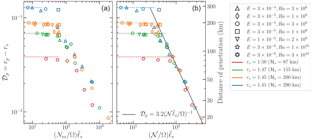
Figure 2. Distance of penetration of the convective flow \mathcal{D}_p (eq. 17) as a function of (N_m/\Omega)\bar{\ell}_s (left-hand panel) and as a function of (N/\Omega)\bar{\ell}_s (right-hand panel). The colour of the symbols correspond to the thickness of the stratified layer \mathcal{H}_s , while the shape correspond to different (E, Ra) combination of parameters listed in Table A1. In each panel, the coloured dashed lines correspond to the maximum extent of the penetration, that is \mathcal{D}_p = \mathcal{H}_s . The solid black line in panel (b) corresponds to a best fit for the models with (N/\Omega)\bar{\ell}_s > 80 .
