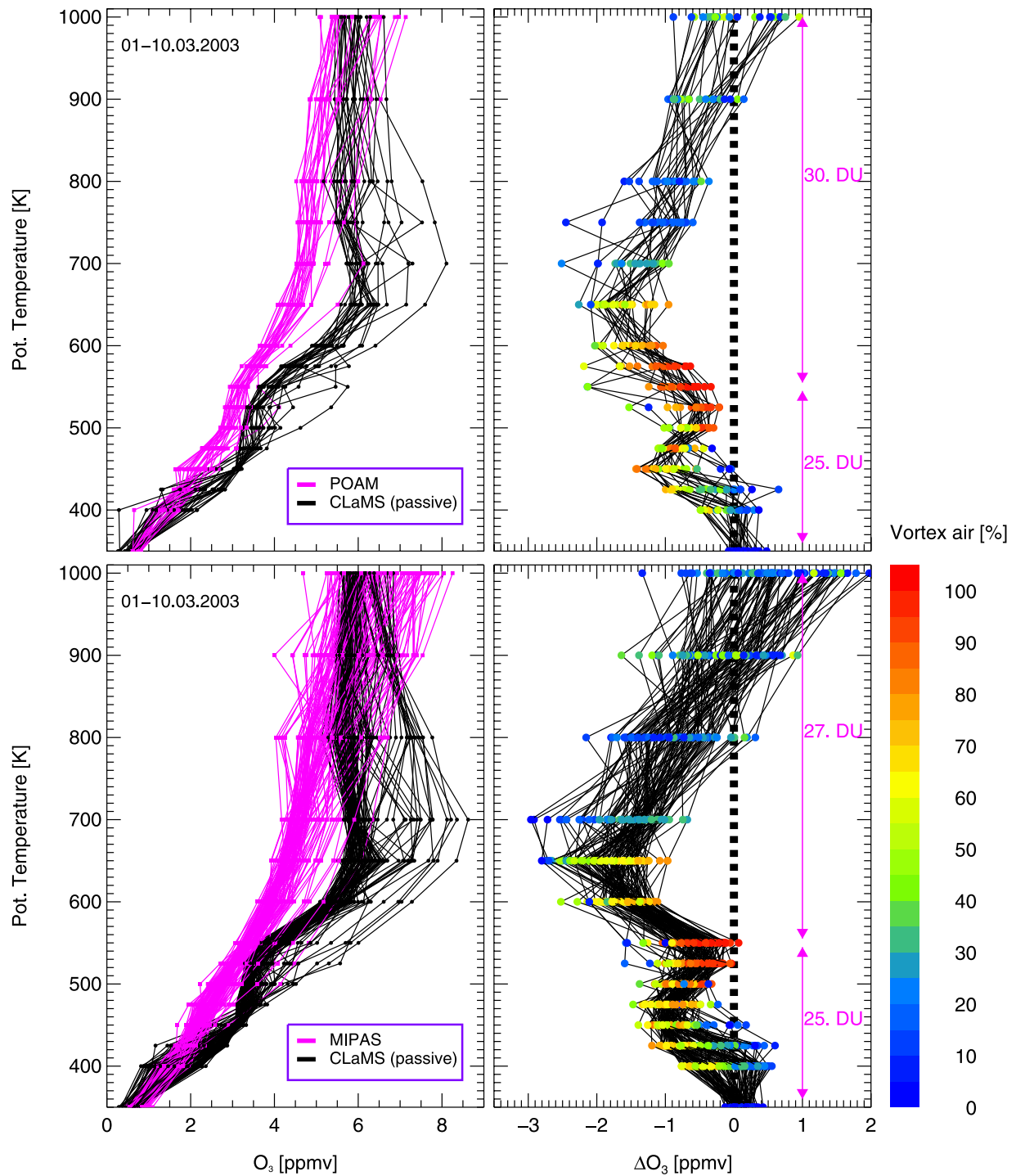
Figure 1. (left) O_3 profiles observed (pink) by (top) POAM and (bottom) MIPAS versus passive O_3 transported by CLaMS (black) between 1 and 10 March and poleward of 65^\circ\text{N} equivalent latitude (calculated at \theta = 450\text{ K} ). (right) Corresponding O_3 loss ( \Delta O_3 ), i.e., the difference between the observed and simulated profiles. Each air parcel sampled along the profile (bold circles) was colored by the percentage of the pure vortex air calculated with CLaMS (i.e., red means air masses within a well-isolated vortex). The pink arrows denote the column O_3 loss integrated between 350\text{--}550\text{ K} and 550\text{--}1000\text{ K} which, as shown in this paper, can be attributed to halogen and \text{NO}_x chemistry, respectively.
