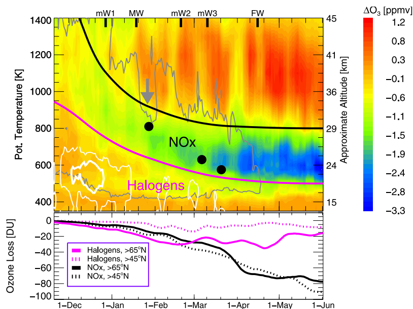
Figure 2. (top) Accumulated O 3 loss ( \Delta O_3 ) between 17 November 2002 and 1 June 2003 and averaged poleward of 65°N equivalent latitude (calculated at \theta = 450 K). \Delta O_3 is derived from the difference between the satellite observations (POAM) and simulated passive O 3 (CLaMS). A well-isolated vortex exists within the gray line. As a consequence of the major warming (MW) in January, an increase of the vortex permeability (gray arrow) leads to a strong intrusion of subtropical, O 3 -rich air into the polar region. The black dots denote places where balloons sampled mesospheric air. The thick pink line approximates the upper boundary of the region where PSCs were observed (thin and thick white lines correspond to the possible PSC area of 1 and 10 \times 10^6 km 2 , respectively [Tilmes et al. , 2003]). The thick black line approximately separates the region of O 3 loss from the region of O 3 production. (bottom) Corresponding column O 3 loss (solid lines) calculated below the thick pink line (halogen-induced within the vortex) and between the thick black and pink lines (NO x -induced). The dotted lines result when our calculations are extended over a region poleward of 45°N equivalent latitude (MIPAS).
