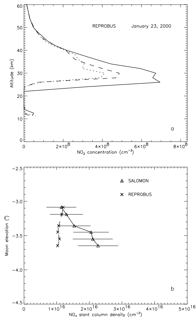
Figure 6. (a) NO 2 vertical profiles computed by the 3-D CTM Reprobis at locations 67 N, 24 E (full line), 70 N, 35 E (dotted line) and 71 N, 38 E (dashed line) on 23 January 2000 at 1700 UT. The balloon altitude is approximately 27 km. The location 67 N, 24 E is the mean of the locations of the entry point of the line of sights for Moon elevation between -3^{\circ} and -3.7^{\circ} at 25 km. The location 70 N, 35 E is the mean of the location of the exit points at level between 25 and 35 km for Moon elevation -3^{\circ} . The location 71 N, 38 E is the mean of the locations of the exit points at levels between 25 and 35 km for Moon elevation -3.7^{\circ} . The three profiles show that the horizontal homogeneity hypothesis is not strictly true along the lines of sights. (b) Measured slant columns densities as a function of Moon elevation (triangle with error bars and full line) and computed slant column densities using Reprobis simulations and a 3-D geometry (crosses and dashed line).
