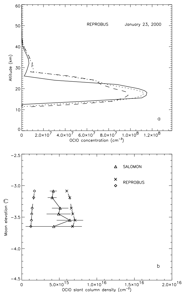
Figure 7. (a) Same as Figure 6a for OCIO. (b) Same as Figure 6b for OCIO. Also shown the slant columns densities computed using Reprobis simulations and a 3-D geometry if OCIO concentration is arbitrarily fixed to zero below 18 km (diamond and dashed line).
