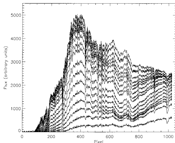
Fig. 6. Raw spectra recorded during the occultation (cosmic rays have been removed).
