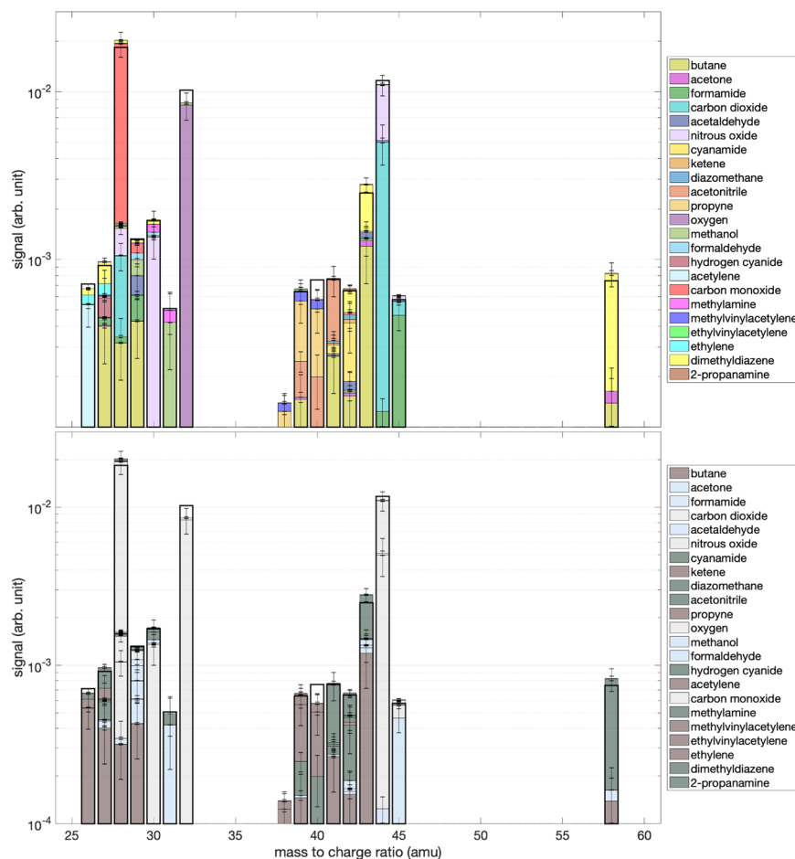
Figure 2. (upper panel) Decomposition of the mass spectrum shown in Fig. 1 using the Monte Carlo approach of Gautier et al. 64 . The experimental mass spectrum used for the decomposition is indicated by the black bold lines. The coloured bars indicate the contribution of each molecule. (lower panel) The coloured bars indicate the contribution of different families of chemical compounds: pollutants derived from water photolysis (grey), oxygenates (blue), hydrocarbons (brown) and nitrogen species (green).
