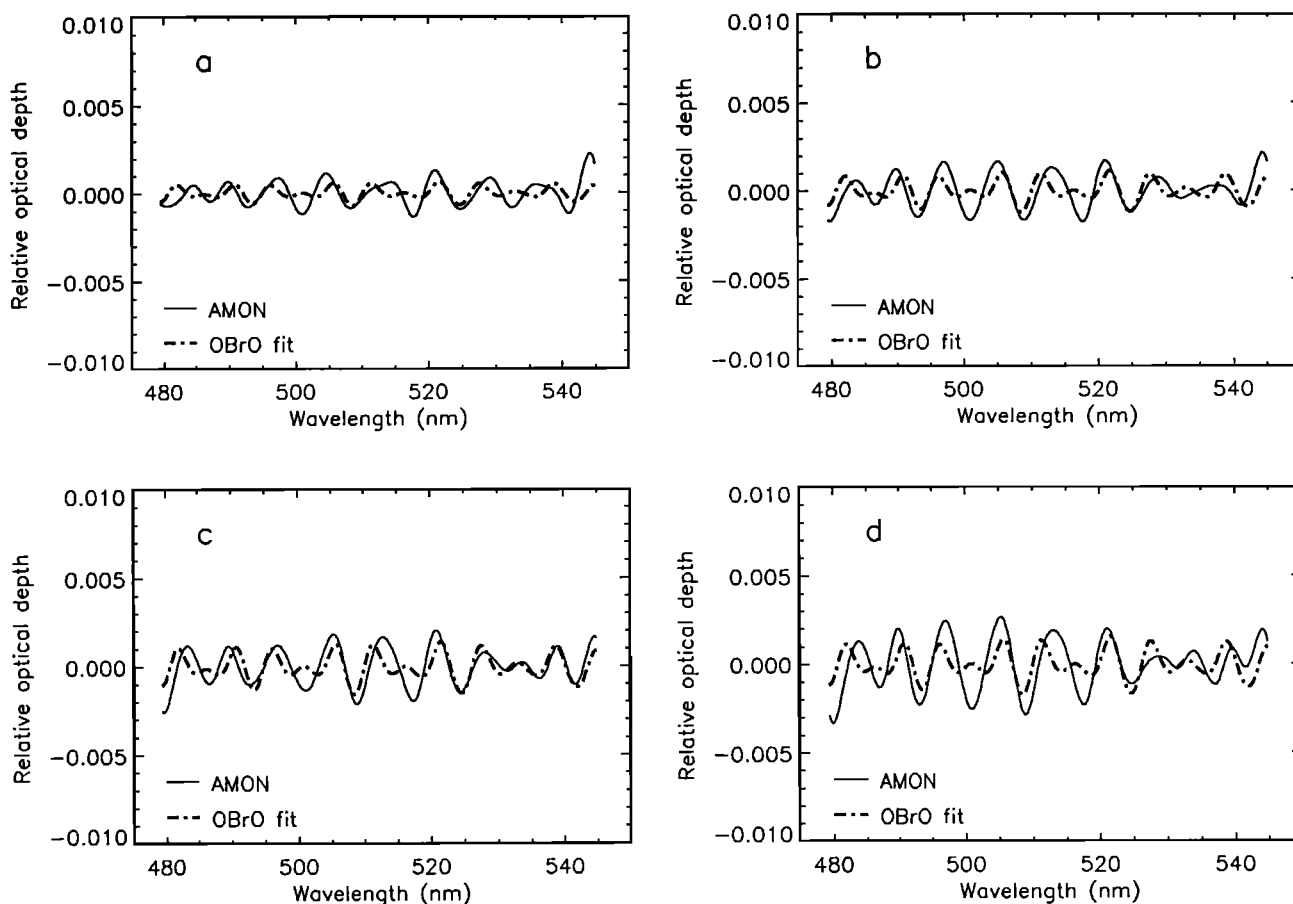
Figure 10. Spectra for the midlatitude flight at Aire sur l'Adour (France) on March, 24, 1994. The star elevation was (a) -1.7^\circ , (b) -2.0^\circ , (c), -2.3^\circ degree, and (d) -2.8^\circ . Because of the poor quality reference spectrum, the best signal-to-noise ratio is only around 3.
