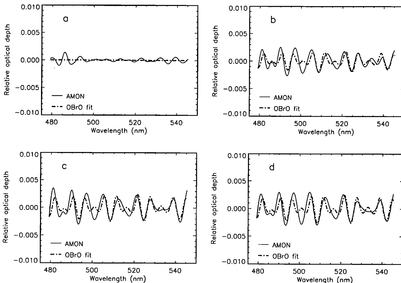
Figure 9. Spectra for the midlatitude flight at Aire sur l'Adour (France) on October, 16, 1993. The star elevation was (a) +1.5^\circ , (b) -3.3^\circ , (c) -3.5^\circ , and (d) -3.8^\circ . The first spectrum, obtained at maximum transmission, corresponds to noise. The signal-to-noise ratio for the three other spectra is 4.2, 4.8, and 4.8, respectively.
