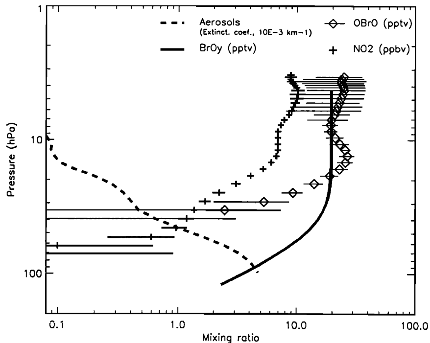
Figure 13. OBrO vertical distribution and comparison with vertical distribution of NO 2 , the extinction coefficient of aerosol (averaged on the 350 - 700 nm spectral domain), and total bromine species (BrOy) predicted by models, for the midlatitude flight on October 16, 1993. The OBrO cross sections are assumed to have a maximum of 1.5 \times 10^{-17} \text{ cm}^{-2} .
