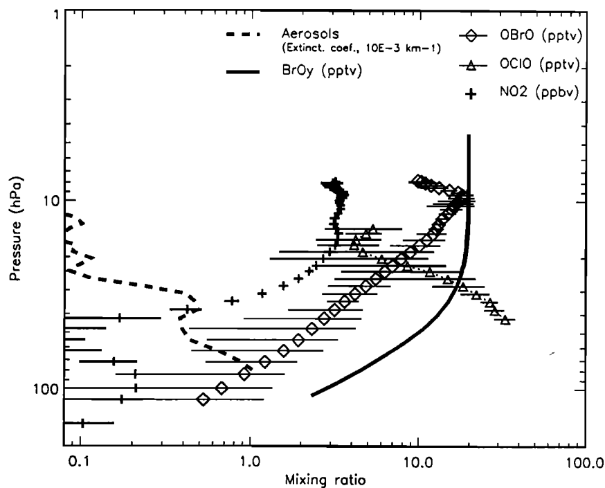
Figure 14. OBrO vertical distribution and comparison with vertical distribution of NO 2 , OClO, the extinction coefficient of aerosol (averaged on the 350 - 700 nm spectral domain), and BrOy predicted by models, for the flight inside the polar vortex on February 26, 1997.
