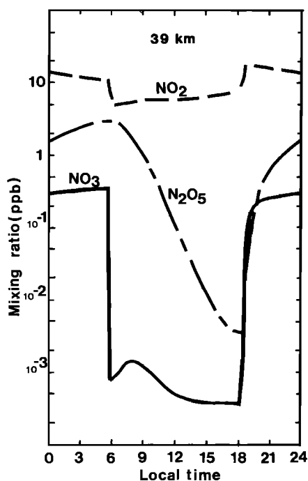
Fig. 1. Diurnal variations of the mixing ratio of NO 2 , N 2 O 5 , and NO 3 , computed with the zero-dimensional model (see text) for September 24, 1985, at 39 km.
