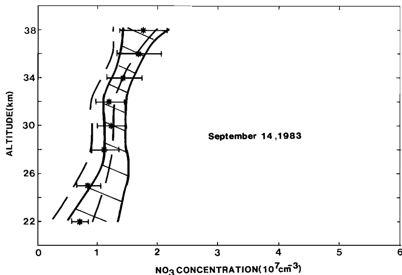
Fig. 6. Same as Figure 3, except for September 14, 1983, at 0330 LT.
