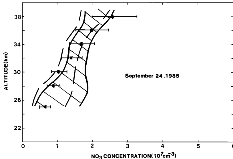
Fig. 7. Same as Figure 3, except for September 24, 1985, at 0315 LT.
