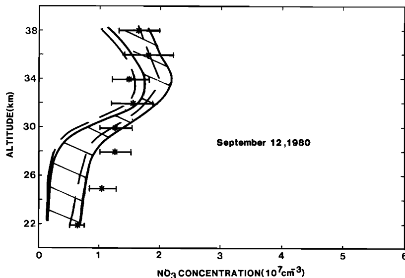
Fig. 3. Measurements of the NO 3 concentration including uncertainties as a function of the altitude [after Naudet et al. , this issue], indicated by the hatched area bounded by solid curves, and the results of the theoretical calculations, indicated by asterisks with errors bars (see text) for September 12, 1980, at 0150 LT. Also shown are the measurements corrected by taking into account the dependence on the temperature of the |NO 3 | absorption cross section (see text), indicated by the area bounded by dashed curves.
