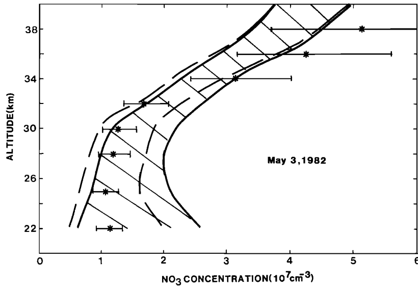
Fig. 5. Same as Figure 3, except for May 3, 1982, at 0330 LT.
