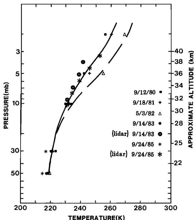
Fig. 2. Mean temperatures derived from the NMC data (see text) for the nights of September 11–12, 1980, September 18–19, 1981, May 2–3, 1982, September 13–14, 1983, and September 23–24, 1985, and measured temperature by lidar at l'Observatoire de Haute Provence on the nights of September 13–14, 1983, and September 23–24, 1985, as a function of the pressure P or the approximate altitude h . Also shown are the standard zonal mean temperatures for September (solid curve) and May (dashed curve). The approximate altitudes are computed by assuming the standard zonal mean temperatures for May or September. Note that although the temperatures are very different above 10 mbar, the approximate altitudes are very close for these two months (the differences are smaller than 200 m).
