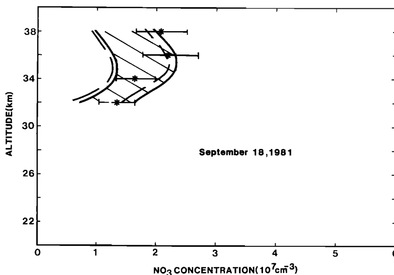
Fig. 4. Same as Figure 3, except for September 18, 1981, at 2140 LT.
