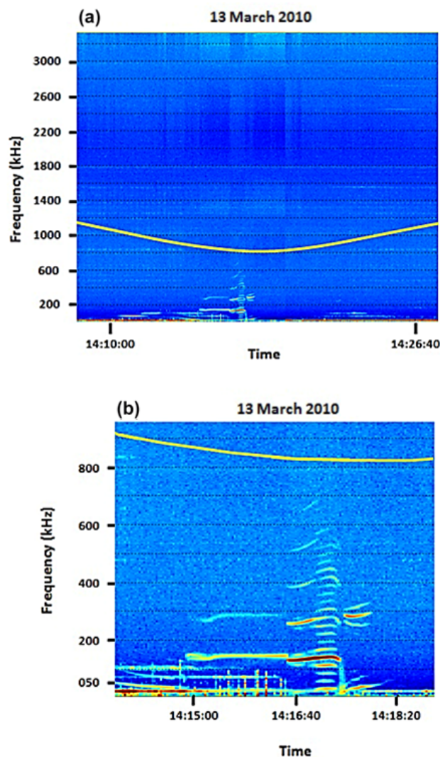
Figure 2. Like in Fig. 1 for an event recorded by DEMETER on 13 March 2010.
