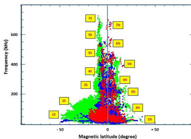
Figure 6. Overlapping of the three power levels displayed in Fig. 5. The spectral pattern is a “Christmas tree” with a “trunk” along the magnetic equatorial plane. We have indicated by numbers the main parts of the spectral pattern for the Southern Hemisphere and Northern Hemisphere. Table 1 lists the observational parameters associated with the investigated events.
