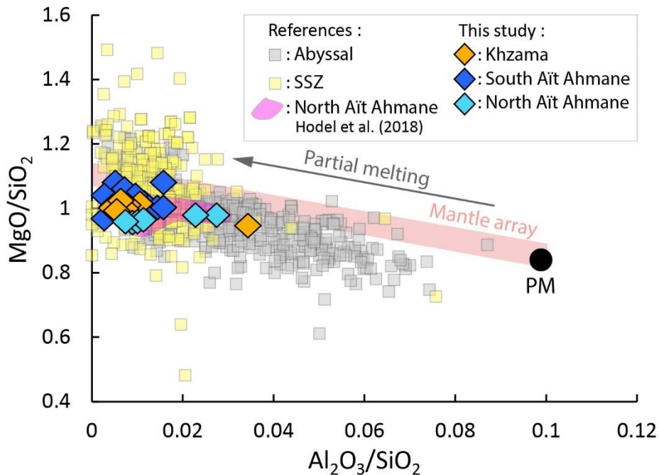
Figure 9: MgO/SiO 2 vs. Al 2 O 3 /SiO 2 ratios for the Khzama and Ait Ahmane (South and North) serpentinites. The pink domain corresponds to the North Ait Ahmane variously hydrothermalized serpentinites of the Hodel et al. (2018) study. Data for abyssal peridotites are from Snow and Dick (1995), Casey (1997), Niu (2004), Paulick et al. (2006), Godard et al. (2008), Augustin et al. (2012), Boschi et al. (2013), Andreani et al. (2014), Chen et al. (2015). Data for SSZ (Supra Subduction Zone) peridotites are from Ishii et al. (1992), Parkinson and Pearce (1998), Pearce et al. (2000), Savov et al. (2005, 2007), Marchesi et al. (2006, 2009) Kodolányi et al. (2012). Mantle array is from Jagoutz et al. (1979) and Hart and Zindler (1986). Primitive mantle values are from McDonough and Sun (1995).
