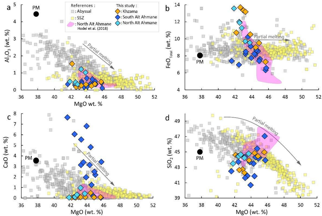
Figure 10: Bulk-rock major oxides contents vs. MgO content (wt%) diagrams for the Khzama and Aït Ahmane (South and North) serpentinites. Element concentrations are recalculated on a LOI-free basis. (a) Al 2 O 3 vs. MgO; (b) FeO vs. MgO, (c) CaO vs. MgO and (d) SiO 2 vs. MgO contents. The pink domain corresponds to the North Aït Ahmane variously hydrothermalized serpentinites of the Hodel et al. (2018) study. Data for abyssal peridotites are from Snow and Dick (1995), Casey (1997), Niu (2004), Paulick et al. (2006), Godard et al. (2008), Augustin et al. (2012), Boschi et al. (2013), Andreani et al. (2014), Chen et al. (2015). Data for SSZ peridotites are from Ishii et al. (1992), Parkinson and Pearce (1998), Pearce et al. (2000), Savov et al. (2005, 2007), Marchesi et al. (2006, 2009), Kodolányi et al. (2012). Primitive Mantle (PM) values are from McDonough and Sun (1995).
