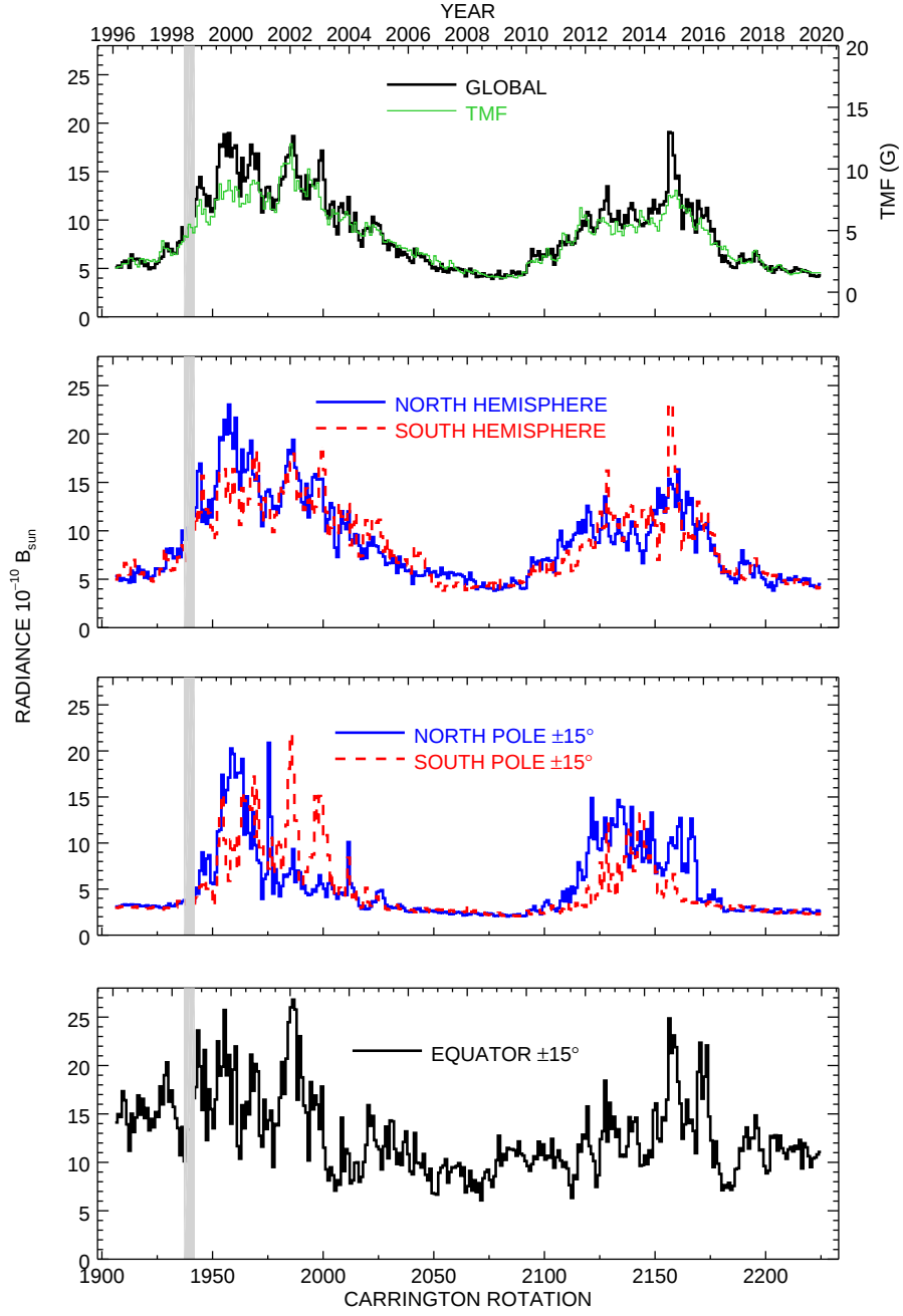
Figure 29. Monthly averaged profiles extracted from the multi-annual synoptic map of the radiance of the K-corona at 2.7R_\odot , globally, in the two hemispheres, and in polar and equatorial sectors.
