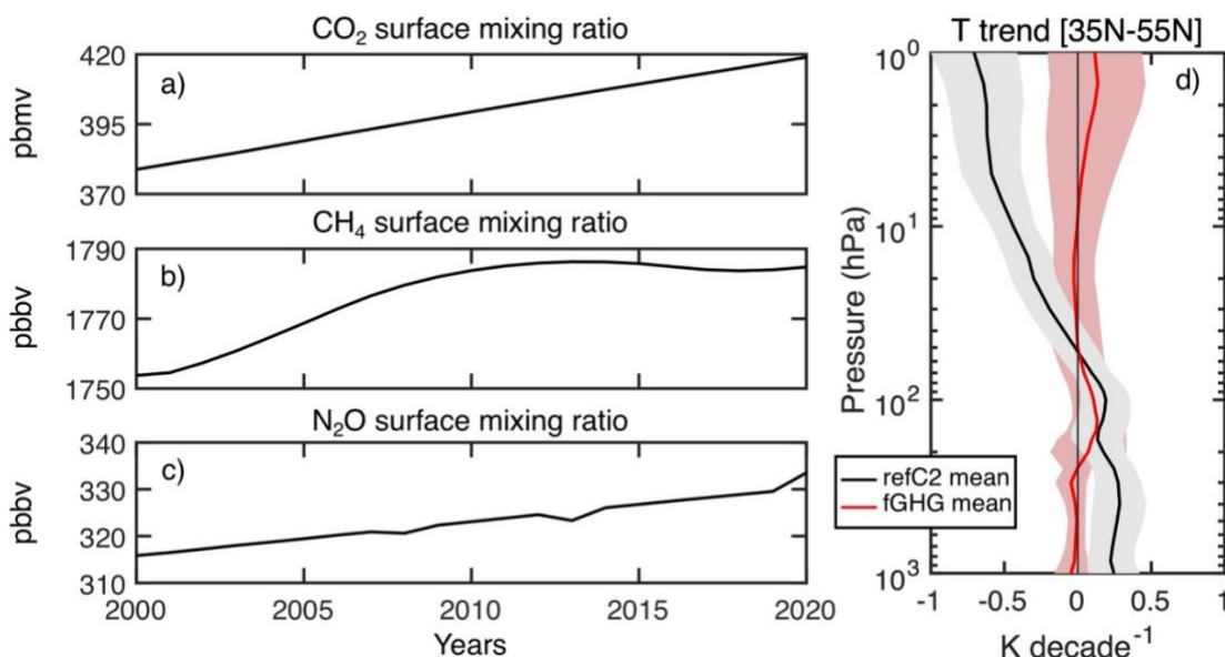
Fig. 7. Time series (2000–2020) of surface mixing ratios of CO 2 (a), CH 4 (b) and N 2 O (c); values are those used as prescribed boundary conditions for the CCM1 RefC2 numerical experiments (Eyring et al., 2013). Panel (d): vertical profiles of northern mid-latitude trends (35N–55N) of temperature (K/decade) averaged over all available models for refC2 (black line) and fGHG (red line). The corresponding shadings represent \pm 1 \sigma of the ensemble of models. The profiles for the single models are reported in Fig. S2.
