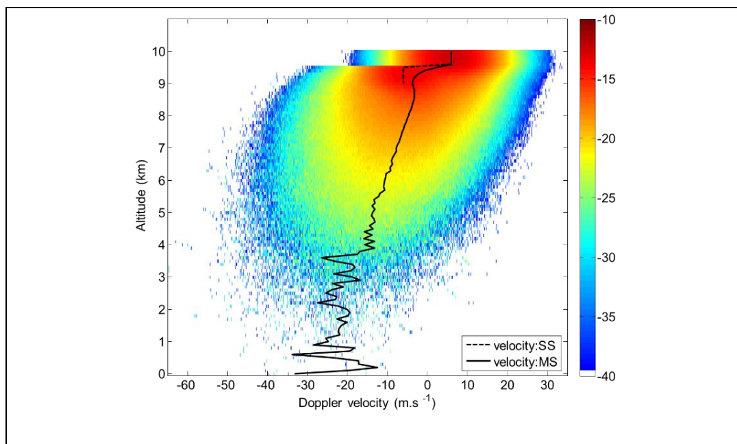
Figure 10: Vertical profiles of MS radar Doppler spectrum (logarithm of the spectra density (in \text{m}^{-1}.\text{sr}^{-1}.\text{(m.s}^{-1})^{-1} )) in CPR/EarthCARE configuration simulated by McRALI-FR. The MS Doppler velocity (black line) and SS (black dotted line) vertical profiles of Doppler velocity are superimposed. The homogeneous cloud layer base altitude is 9 km, its geometrical thickness is 1 km. The vertical velocity is set to 6 \text{ m.s}^{-1} (downdraft) and to -6 \text{ m.s}^{-1} (updraft) in the upper and the lower part of the cloud layer, respectively. Optical depth is 3.
