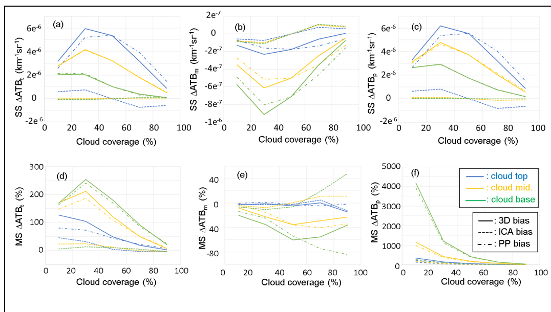
Figure 15: ICA (dashed), PP (dotted dashed) and 3D (full line) biases under single scattering (SS) regime on (a) total ATB, (b) molecular ATB and (c) particulate ATB as a function of cloud coverage (%) inside the lidar receiver FOV, computed at cloud top (9.8 km, blue curves), in the middle of the cloud (9.5 km; yellow curves) and at cloud base (9.2 km; green curves). (d), (e) and (f) same as (a), (b) and (c) but for relative bias and MS regime. Cloud optical depth is 3.
