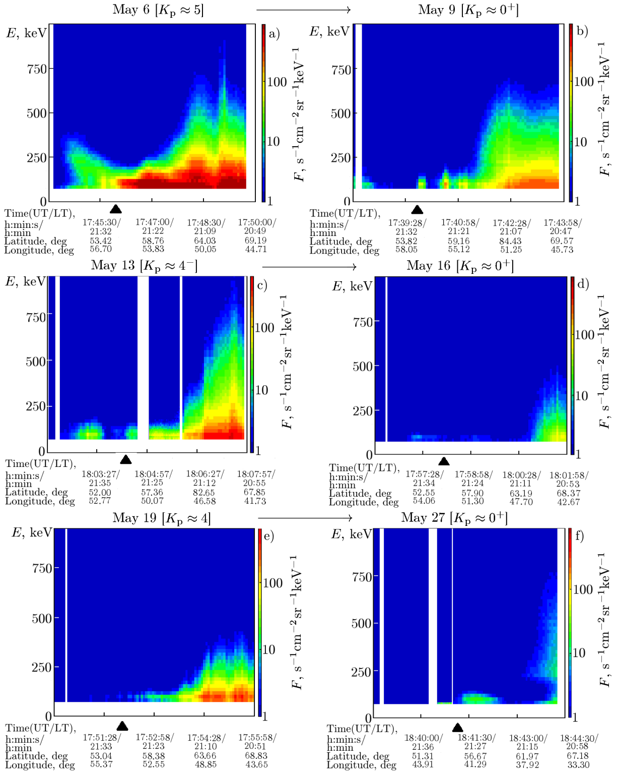
Fig. 1. Spectral and spatial characteristics of the natural precipitations of energetic electrons measured on May 6–27, 2006 under conditions of a strongly varying geomagnetic activity level day by day when the DEMETER spacecraft passed above an idle Sura facility. Hereafter, the coordinates of the center of the perturbed magnetic flux tube are marked by a black triangle under the abscissa axis.
