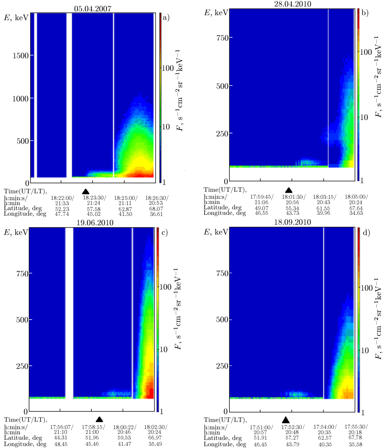
Fig. 2. Examples of the sessions in which the precipitations that could certainly be qualified as artificial (sessions 7, 15, 18, and 20 on panels a , b , c , and d , respectively) were not detected during the Sura operation.
