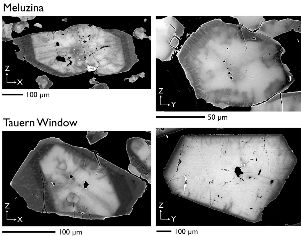
Fig. 6. Chemical zonation patterns parallel and normal to lineation in garnets from the Meluzina and Tauern sections. Left: XZ-sections, Right hand figures: YZ-sections. The YZ-sections show approximately the same thickness of growth rims around the cores in all directions.
