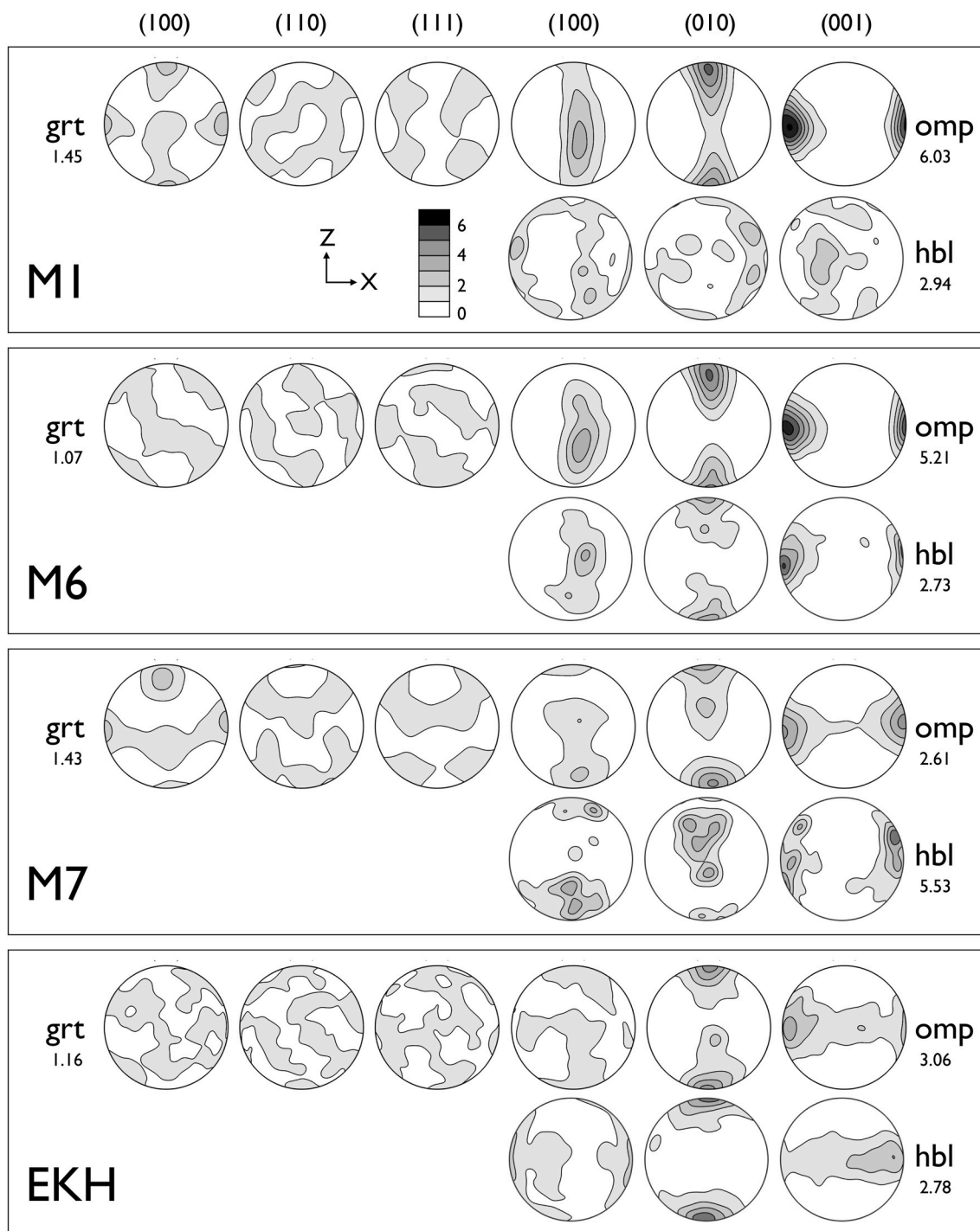
Fig. 10. Crystallographic preferred orientation (CPO) of garnet, omphacite, and hornblende from the Bohemian massif (M1, M6 and M7) and the Tauern Window (EKH) eclogites. Left: pole figures of (100), (110) and (111) of garnet; right, pole figures of (100), (010) and (001) of omphacite (above) and hornblende (below). Contours are multiples of the uniform distribution. J-indices are indicated below the mineral name.
