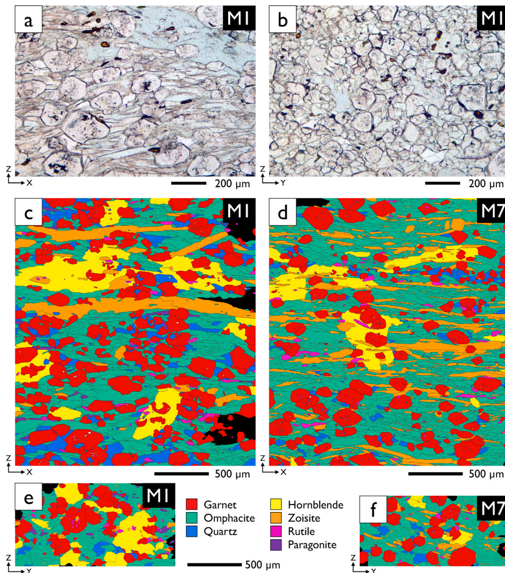
Fig. 1. Microstructures of the Bohemian Massif eclogites. (a) & (b) Light micrographs of M1 parallel and normal to lineation. (c)–(f) Phase maps derived from EBSD and BSE images, parallel and normal to lineation for M1 and M7.
