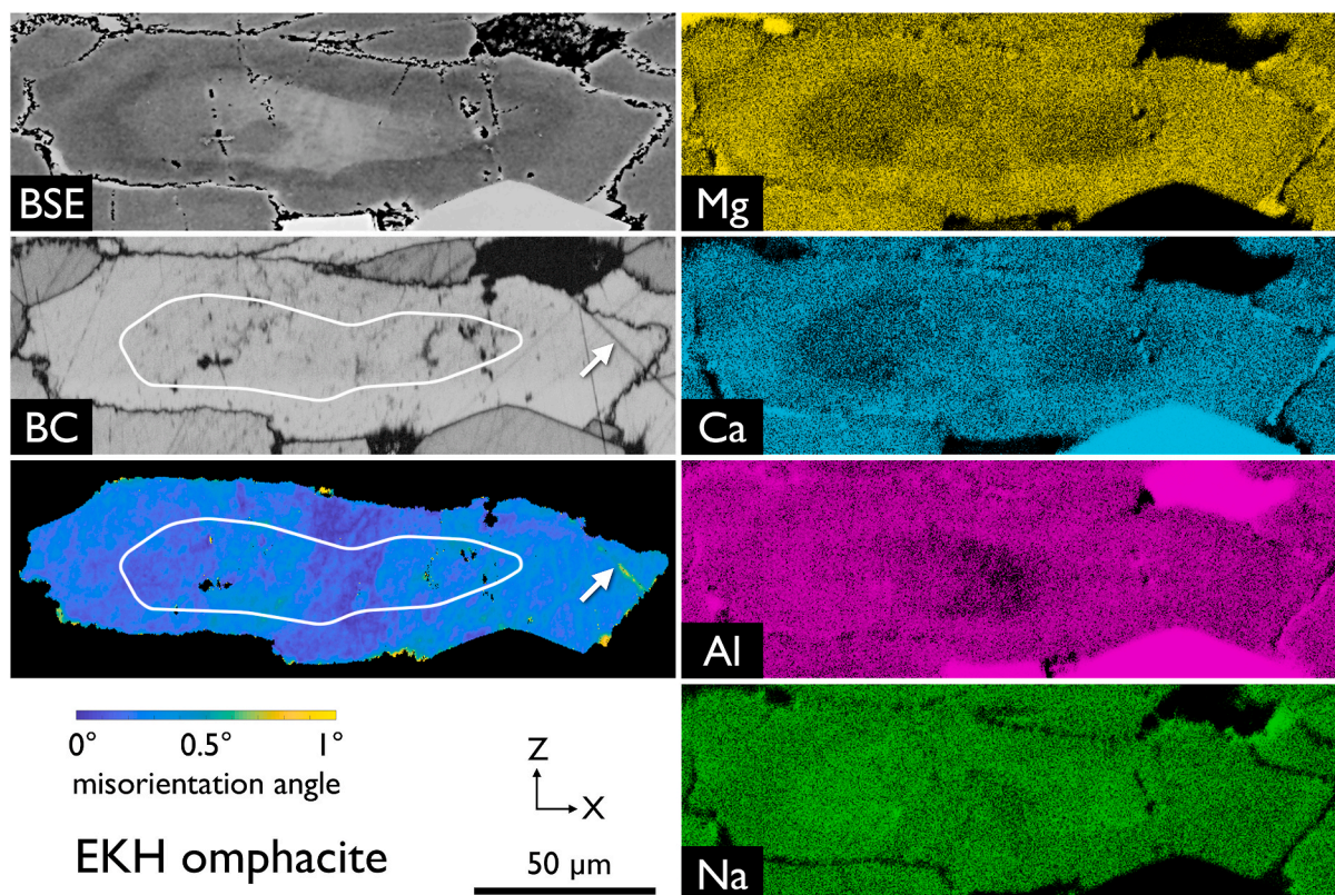
Fig. 9. Omphacite zonation from a Tauern Window eclogite. Left: Back scatter contrast image (BSE), Band contrast (BC) and misorientation map (showing angles of \text{mis2mean} ) of an omphacite grain from sample EKH with boundary of zonation superposed. Note that misorientation angles are extremely small ( <1^\circ ). Note also that misorientation boundaries may be induced by scratches (compare with BC, white arrows), but do not coincide with zonation boundaries. Right: Element maps (Mg = yellow, Ca = turquoise, Al = purple, Na = green). Note that the zonation is widest parallel to the stretching direction X and continuous on faces normal to the shortening direction Z. (For interpretation of the references to color in this figure legend, the reader is referred to the Web version of this article)
