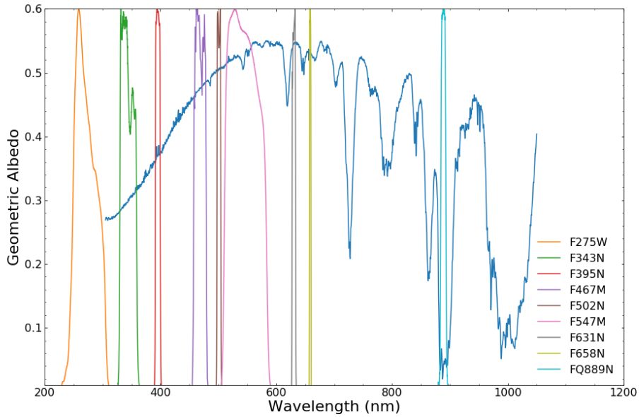
Figure 2. HST/WFC3 filters used in this work together with the geometric albedo spectrum of Jupiter obtained by Karkoschka (1998). Transmissivity of the filters are scaled to the same maximum only for representation purposes.
