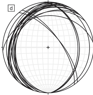
Upper Eocene - Oligocene Mansi Gale Group Layering/bedding (near Shangalon; n = 21 )
