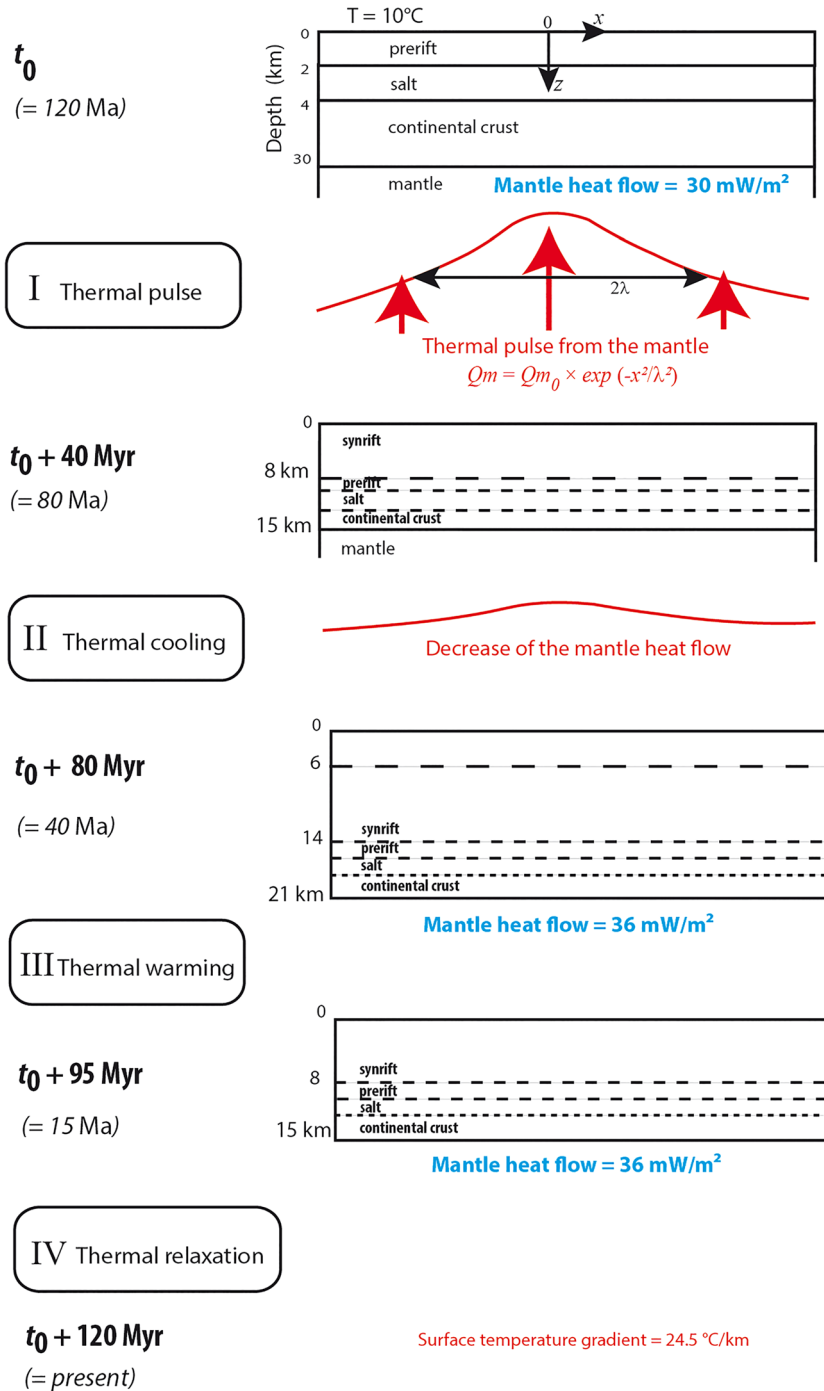
Figure 10. Conceptual model of the four stages of thermal events since 120 Ma of the Mauléon basin. Lithologies are shown but are not accounted for in thermal properties (see text). The final value of mantle heat flow ( 36 \text{ mW/m}^2 ) accounts for present-day surface temperature gradients.
