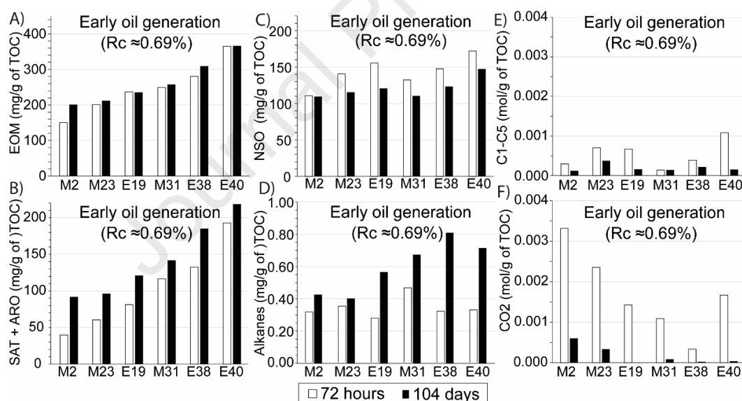
32 33 Fig. 7. Comparison of A) extractible organic matter (EOM), B) saturated (SAT), aromatic (ARO) 34 hydrocarbons, C) NSO, D) alkanes (hopanes, steranes, n-alkanes, branched alkanes, isoprenoids and 35 alkylcycloalkanes), E) C 1 -C 5 gaseous hydrocarbons and F) CO 2 concentrations in the early oil 36 generation stage after 104 days and 72 hours of thermal maturation. The division of hydrocarbons 37 generation stages is based on Rc values, Rock Eval parameters, biomarker ratios and Fig.2.
