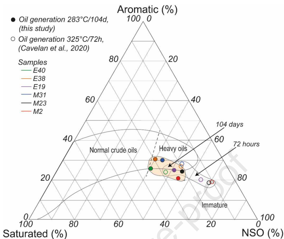
Fig. 4. Comparison of the relative proportion of saturated, aromatic hydrocarbons and NSO during oil generation ( R_c of ca. 0.70%) after 104 days (filled symbols) and 72 hours (open symbols) of thermal maturation. Data of normal crude-oil from Tissot and Welte, (1984).
