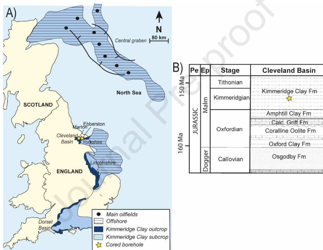
Fig. 1. A) Kimmeridge clay formation across England and North Sea; location of the studies boreholes (modified from Gallois, 2004). B) Simplified stratigraphic column of the Cleveland Basin (modified from Powell, 2010).
