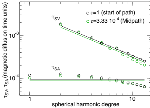
Figure 2. Secular variation and acceleration timescales \tau_{SV}(\ell) , \tau_{SA}(\ell) as functions of the spherical harmonic degree \ell , in the start-of-path and Midpath model. Solid lines represent the best fits of the form \tau_{SV}(\ell) = \tau_{SV}^1/\ell and \tau_{SA}(\ell) = \tau_{SA}^0 , with the master timescales \tau_{SV}^1 , \tau_{SA}^0 reported in Table 2.
