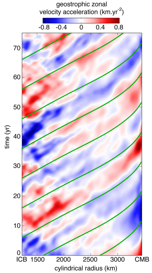
Figure 10. Time-cylindrical radius plot of the time derivative \partial v_g / \partial t of the geostrophic velocity (eq. 13) outside the tangent cylinder in the Midpath model. Green lines represent the theoretical propagation tracks of torsional waves at the Alfvén speed c_A(s, t) (eq. 15).
