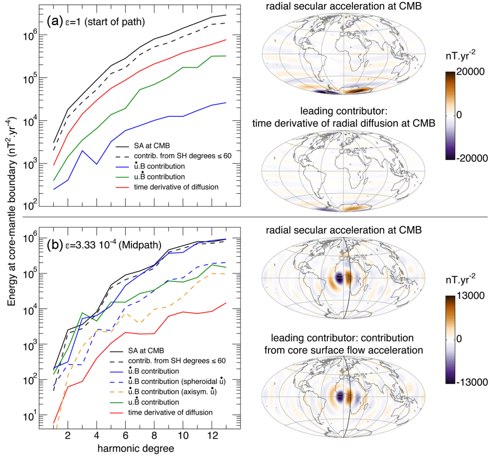
Figure 8. Left: core–mantle boundary spatial SA energy spectra up to spherical harmonic degree 13, at pulse times marked by arrows in Fig. 3(d) for the start-of-path (a) and Midpath (b) models. See Fig. 7 for the definitions of the presented contributions. Here, the contribution from the interaction of the spheroidal part of \partial\mathbf{u}/\partial t with \mathbf{B} is additionally reported (dashed blue line). Right: hammer projections of the radial SA at the core–mantle boundary (orange is outwards), and the leading contribution to this SA. The black curves in (b) delineate the longitude selected for analysis of the pulse event in Section 3.3.
