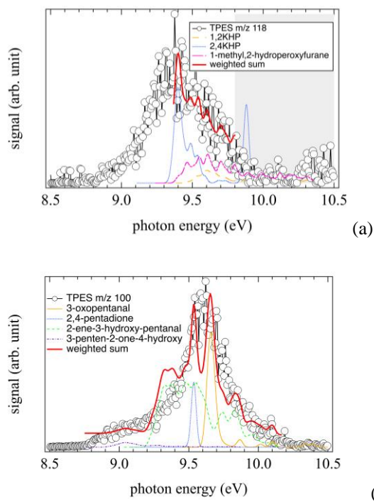
Figure 2: Comparison between the measured (under the conditions of Fig. 1) TPES spectra for m/z 118 (a) and 100 (b), and theoretically calculated PES based on the compounds listed in Table 1.
