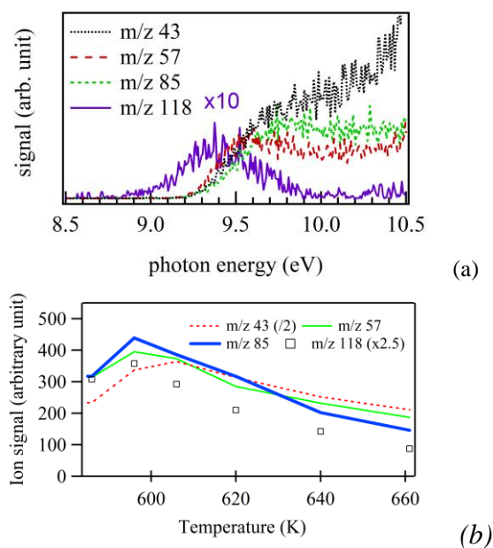
Figure 3: M/z 118, 85, 57 and 43 (under the conditions of Fig. 1): (a) TPES and (b) ion signal at 10.5 eV as a function on temperature (numbers in the graphs indicate factors by which the signal are multiplied/divided).
