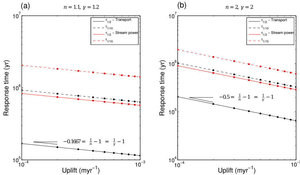
Figure 13. Log–log plot of response time for different slope exponents and uplift rates to a change to a precipitation rate from an initial value of \alpha_0 = 1 to \alpha_1 = 0.5 \text{ m yr}^{-1} ; \tau_{1/2} is the time for the sediment flux to recover by half of the magnitude change in sediment flux and \tau_{1/10} is the time for the sediment flux to recover by 90%. (a) Response time for the transport model (Eq. 8) and stream power model (Eq. 12) when the slope exponent \gamma = 1.2 and n = 1.2 , respectively. A linear trend is found with a gradient of -1.667 . (b) Response time for the transport model and stream power model when the slope exponent \gamma = 2 and n = 2 , respectively. A linear trend is found with a gradient of -0.5 .
