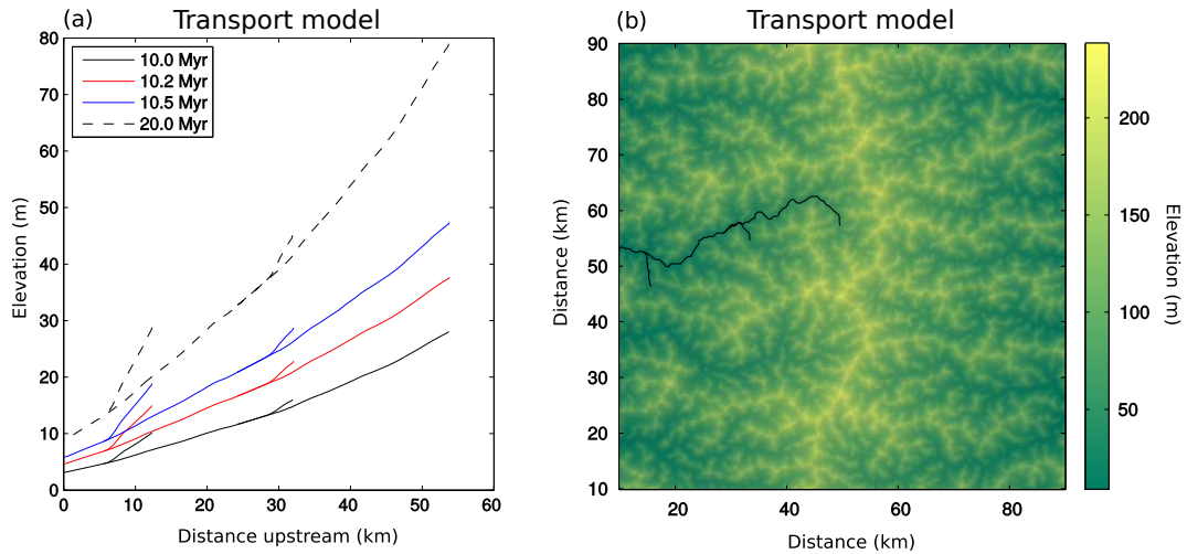
Figure 7. Transport model evolution due to a reduction in precipitation. (a) Selected river-long profile response to a change in precipitation. The black line is the profile just before a factor of 2 reduction in precipitation. The red and blue lines are 200 and 500 kyr after the reduction in precipitation. The dashed black line is the steady-state profile. (b) Trunk stream used for the analysis with the steady-state elevation.
