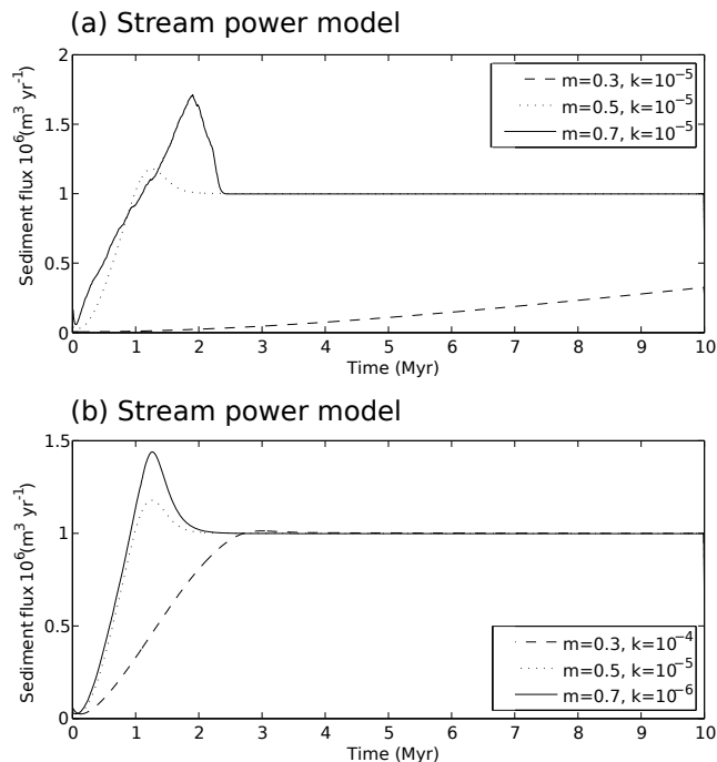
Figure 4. Sediment flux out of the model domain for the stream power models in which (a) m = 0.3, 0.5, and 0.7 and k = 10^{-5} (m^2 yr^{-1})^{1-m} ; (b) m = 0.3, 0.5, and 0.7 and k = 10^{-4}, 10^{-5}, and 10^{-6} m^{-1} (m^2 yr^{-1})^{1-m} .
