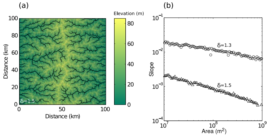
Figure 3. (a) Steady-state topography after 10 Myr for the transport model in which \delta = 1.5 and c = 10^{-4} (m^2 yr^{-1})^{1-\delta} . (b) Slope–area relationship for the transport model for \delta = 1.3 and \delta = 1.5 .
