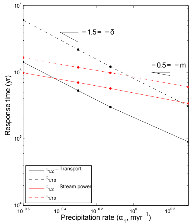
Figure 10. Log-log plot of response time to a change to a precipitation rate of \alpha_1 from an initial value of \alpha_0 = 1 \text{ myr}^{-1} when the model domain is 100 by 100 km (see Table 2); \tau_{1/2} is the time for the sediment flux to recover by half of the magnitude change in sediment flux and \tau_{1/10} is the time for the sediment flux to recover by 90%.
