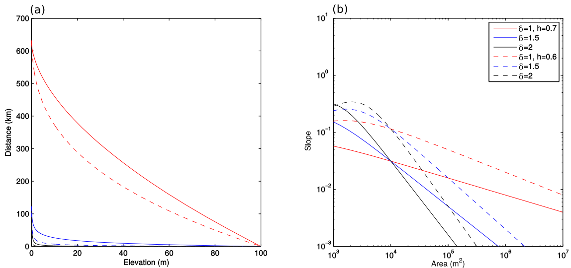
Figure A2. (a) Steady-state elevation and (b) slope–area relationship for the numerical solution to 1-D sediment transport (Eq. 8) for which the area, a , is taken to be related to distance x by a = x^p , where p = 1/h and h is the Hack exponent. Red lines are for the case in which n = 1 , blue lines for n = 1.5 , and black lines for n = 2 . Solid lines are for h = 0.7 . Dashed lines are for h = 0.6 .
