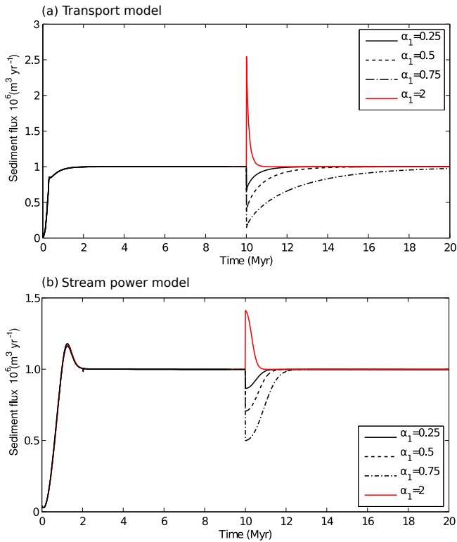
Figure 9. (a) Response of the transport model to a change in precipitation rate. Equation (6) is solved for \delta = 1.5 and c = 1 \times 10^{-4} (\text{m}^2 \text{yr}^{-1})^{1-\delta} . The precipitation rate is initially \alpha_0 = 1 \text{ myr}^{-1} and changes to \alpha_1 = 0.25, 0.5, 0.75, or 2 \text{ myr}^{-1} after 10 Myr. (b) Response of the stream power model to a change in precipitation rate. Equation (6) is solved for m = 0.5 and k = 1 \times 10^{-5} \text{ m}^{-1} (\text{m}^2 \text{yr}^{-1})^{1-m} . The precipitation rate is initially \alpha_0 = 1 \text{ myr}^{-1} and changes to \alpha_1 = 0.25, 0.5, 0.75, or 2 \text{ myr}^{-1} after 10 Myr.
