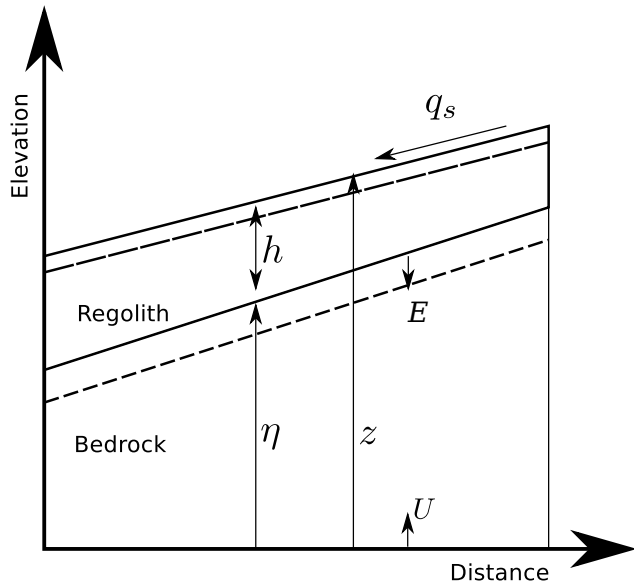
Figure 1. Diagram showing the conservation of mass within a 2-D domain where mass enters the system through uplift, U (units of \text{m s}^{-1} ), and exists as sediment transported, q_s ( \text{m}^2 \text{s}^{-1} ), out of the domain. E ( \text{m s}^{-1} ) is the rate of production of regolith, h (m) is the thickness of regolith, \eta (m) is the bedrock elevation, and z (m) is the total elevation.
