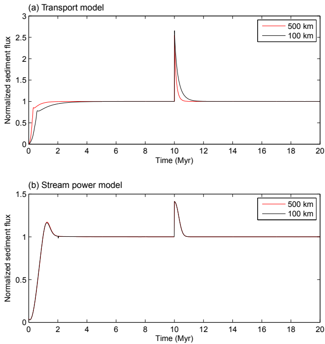
Figure 11. (a) Response of the transport model to a change in precipitation rate for two different model dimensions, 100 by 100 km and 500 by 500 km. Equation (6) is solved for \delta = 1.5 and c = 1 \times 10^{-4} (\text{m}^2 \text{yr}^{-1})^{1-\delta} . The precipitation rate is initially \alpha_0 = 1 \text{ m yr}^{-1} and changes to \alpha_1 = 2 \text{ m yr}^{-1} after 10 Myr. (b) Response of the stream power model to a change in precipitation rate for two different model dimensions, 100 by 100 km and 500 by 500 km. Equation (6) is solved for m = 0.5 and k = 1 \times 10^{-5} \text{ m}^{-1} (\text{m}^2 \text{yr}^{-1})^{1-m} . The precipitation rate is initially \alpha_0 = 1 \text{ m yr}^{-1} and changes to \alpha_1 = 2 \text{ m yr}^{-1} after 10 Myr.
