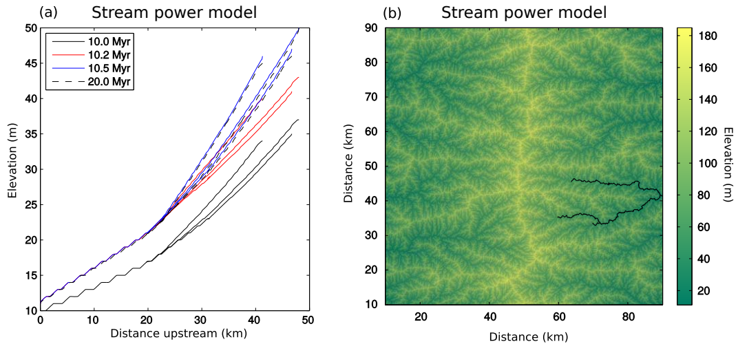
Figure 8. Stream power model evolution due to a reduction in precipitation. (a) Selected river-long profile response to a change in precipitation. The black line is the profile just before a factor of 2 reduction in precipitation. The red and blue lines are 200 and 500 kyr after the reduction in precipitation. The dashed black line is the steady-state profile. (b) Trunk stream used for the analysis with the steady-state elevation.
