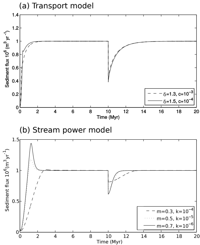
Figure 6. Response of the transport and stream power model to a reduction in precipitation rate. (a) Sediment flux for the transport model for a step reduction in precipitation from 1 to 0.5 \text{ m yr}^{-1} after 10 Myr. Two models are plotted in which \delta = 1.3 and 1.5 , \kappa = 10^{-2} , and c = 10^{-3} and 10^{-4} (\text{m}^2 \text{ yr}^{-1})^{1-\delta} . (b) Sediment flux for the stream power model for a step reduction in precipitation from \alpha_0 = 1 to \alpha_1 = 0.5 \text{ m yr}^{-1} after 10 Myr. Three models are plotted in which m = 0.3, 0.5 , and 0.7 and k = 10^{-4}, 10^{-5} , and 10^{-6} \text{ m}^{-1} (\text{m}^2 \text{ yr}^{-1})^{1-m} .
