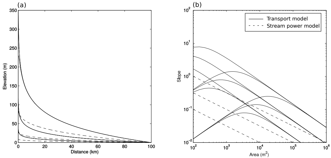
Figure A1. (a) Steady-state profiles of elevation against down-system length and (b) the slope of the profile plotted against the drainage area assuming that area a = x^p , where p = 1/h = \sqrt{2} and h is the Hack exponent. Dashed lines are for the stream power law (Eq. 12) with m = 0.5 and k = 10^{-4} , 10^{-3.5} , and 10^{-3} . The solid lines are for the transport model (Eq. 8 with n = \sqrt{2} , \kappa = 10^{-3} , 1 , and 10^3 \text{ m}^2 \text{ yr}^{-1} and c = 10^{-6} , 10^{-5.5} , and 10^{-5} ).
