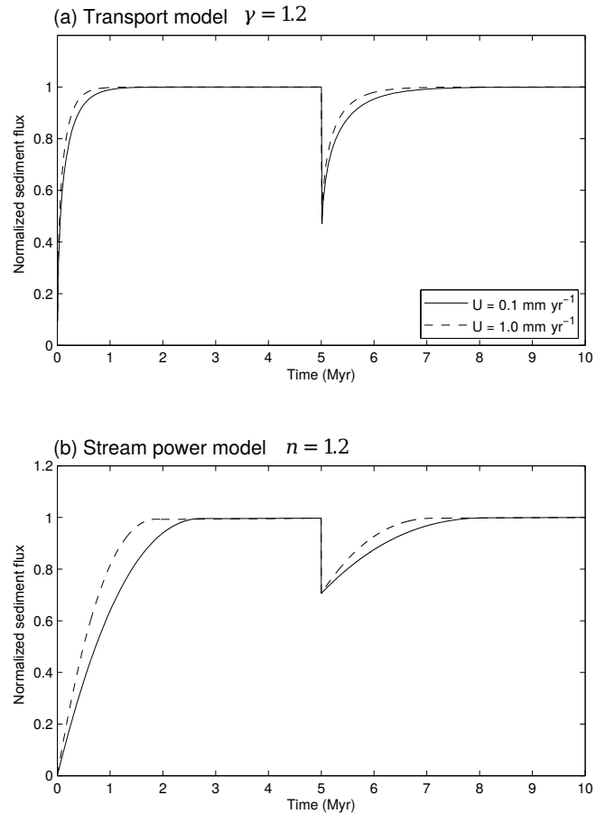
Figure 12. (a) Response of the transport model to a change in precipitation rate for two values of uplift, 0.1 and 1.0 \text{mm yr}^{-1} . Equation (8) is solved for \gamma = 1.2 , \delta = 1.5 , p = 1.1 , and c = 5 \times 10^{-5} (\text{m}^2 \text{yr}^{-1})^{1-\delta} . The precipitation rate is initially \alpha_0 = 1 \text{ m yr}^{-1} and changes to \alpha_1 = 0.5 . (b) Response of the stream power model to a change in precipitation rate for two values of uplift, 0.1 and 1.0 \text{mm yr}^{-1} . Equation (12) is solved for n = 1.2 , m = 0.5 , p = 1.1 , and k = 1 \times 10^{-4} \text{ m}^{-1} (\text{m}^2 \text{yr}^{-1})^{1-m} . The precipitation rate is initially \alpha_0 = 1 \text{ m yr}^{-1} and changes to \alpha_1 = 0.5 after 5 Myr.
