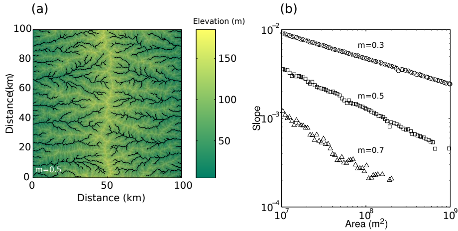
Figure 5. (a) Steady-state topography after 10 Myr for the transport model in which m = 0.5 and k = 10^{-5} \text{ m}^{-1} (\text{m}^2 \text{ yr}^{-1})^{1-m} . (b) Slope–area relationship for the transport model for m = 0.3, 0.5 , and 0.7 .
