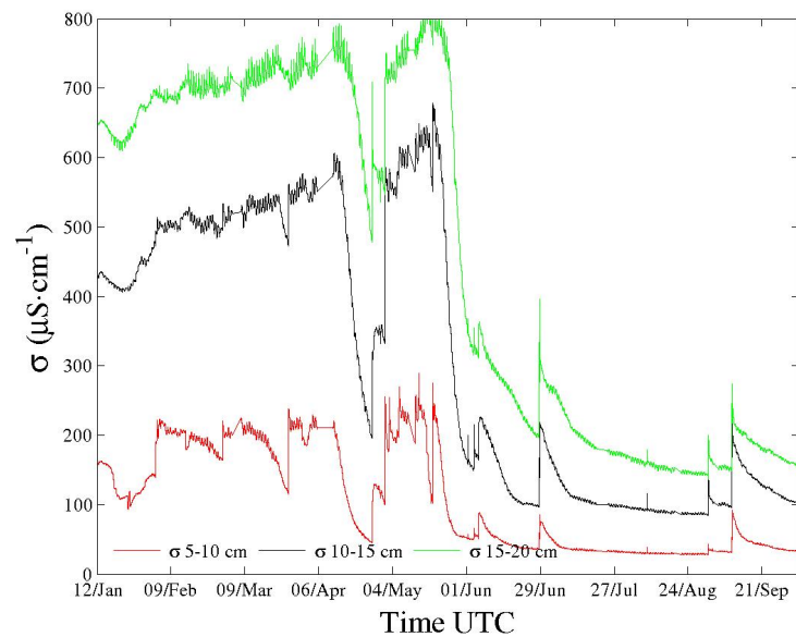
Figure 3. Time series over nine months of a three-channel sensor located in a remote catchment of the French Southern Alps—one point every 10 min. Minor interruptions due to power supply. Soil conductivity profile in \mu\text{S}\cdot\text{cm}^{-1} .
