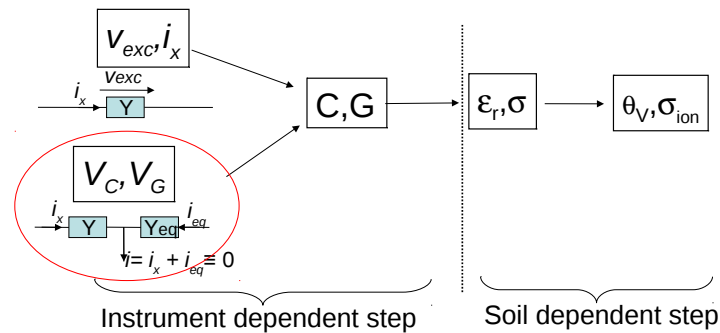
Figure 1. Successive steps of conversion from raw sensor output, direct voltages V_G and V_C in the case of a self-balanced bridge or alternating current i_x and voltage v_{exc} for a method based on Ohm's law, to quantities of interest, soil water content \theta_v and its salinity \sigma_{ion} . Quantities G and C are, respectively, the capacitance and the conductance of the electrodes embedded in the soil, while \epsilon_r and \sigma are soil apparent electric permittivity and conductivity.
