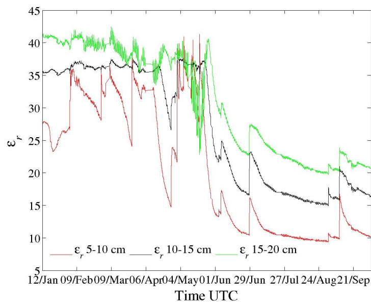
Figure 4. Soil real permittivity profile (see Figure 3).
