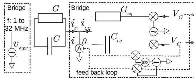
Figure 2. Schematic diagram of a self-balanced bridge. The current i_x flowing through the admittance to be measured, Y = G + jC2\pi f , under the voltage v_{exc} of an on-board oscillator at frequency f , is balanced by the current i_{eq} generated by the bridge. i_{eq} is adjusted to i_x owing to the direct voltages V_G and V_C provided by a feedback loop. At equilibrium, they are proportional to i_x and therefore Y . Synchronous detectors and modulators permit the conversion between alternating and direct voltages using v_{exc} as the alternating reference. Conductance G_{eq} and capacitance C_{eq} give bridge sensitivity and are fixed by passive components.
