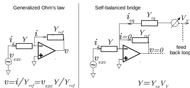
Figure 5. Two techniques in alternating current to measure an unknown admittance Y with a trans-impedance—or current-to-voltage converter—in the circuit input: one based on Ohm’s law (left hand part), the other based on the balanced bridge (right hand part). When the bridge is balanced, trans-impedance output v is zero (as i_x \equiv -i_{eq} ). The automatic adjustment to reach this state, in form of a direct voltage V_Y , is used as the sensor signal. In the Ohm’s law case, v is one of the sensor signals, along with the excitation v_{exc} .
