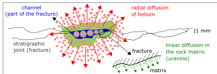
Figure 2. Schematic explanation of the different behavior of helium and uranine. At the small scale sampled by uranine, matrix diffusion is locally perpendicular to the surface and behaves effectively like the parallel plate model. At the larger scale sampled by helium, the presence of macroscopic channels leads to radial diffusion in the matrix, captured by the channel model.
