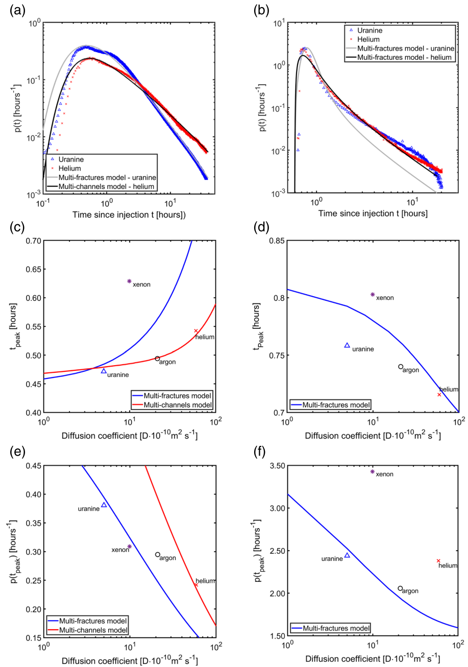
Figure 3. Modeling of the (a) convergent and (b) push-pull experiment for uranine and helium. Peak times of the (c) convergent and (d) push-pull configuration, and peak values in RTD for (e) convergent and (f) push-pull configuration in the parameter adjustment. Tracers are listed in the legend by ascending diffusion coefficient (Table 1).
