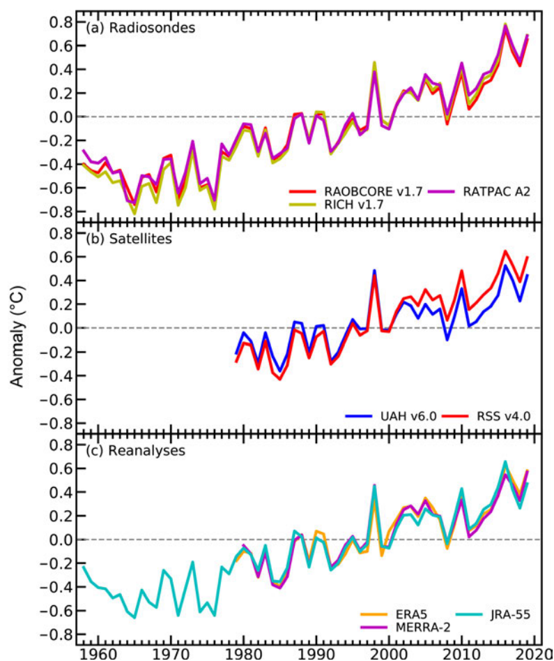
Fig. 2.7. Time series of global annual temperature anomalies (°C) for the lower troposphere from (a) radiosondes, (b) satellite microwave emissions, and (c) reanalyses.
