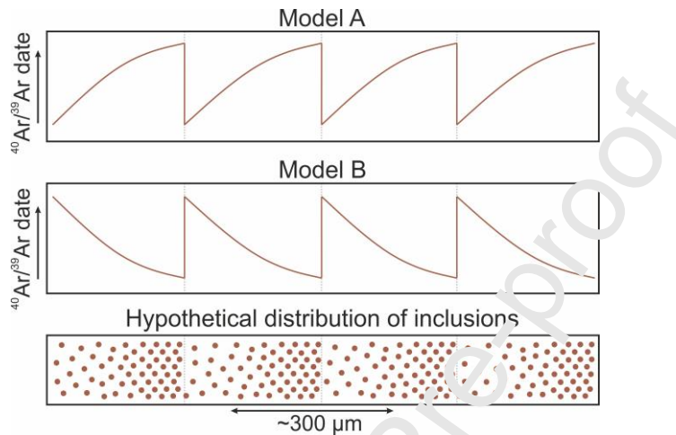
Fig. 10. Hypothetical relationships between the intra-grain ^{40}\text{Ar}/^{39}\text{Ar} date variation and the abundance of inclusions.
