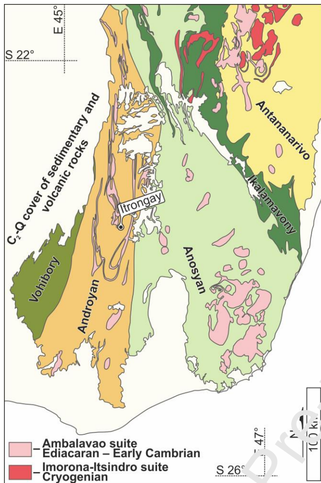
Fig. 1. Geological terrane map showing the relationships between the Vohibory, Androyan, Anosyan, Ikalamaivony and Antananarivo domains in the south of Madagascar (adopted from Roig et al., 2012). Ambalavao and Imorona-Itsindro suites are suites of largely metamorphosed intrusive rocks. The label “Itrongay” shows the location of the \sim 5 \times 20 km field of “pegmatites dites d’Itrongay” from the maps of Savornin (1932; 1933). We sampled near the southwestern boundary of this field (see in section 4.1 for details).
