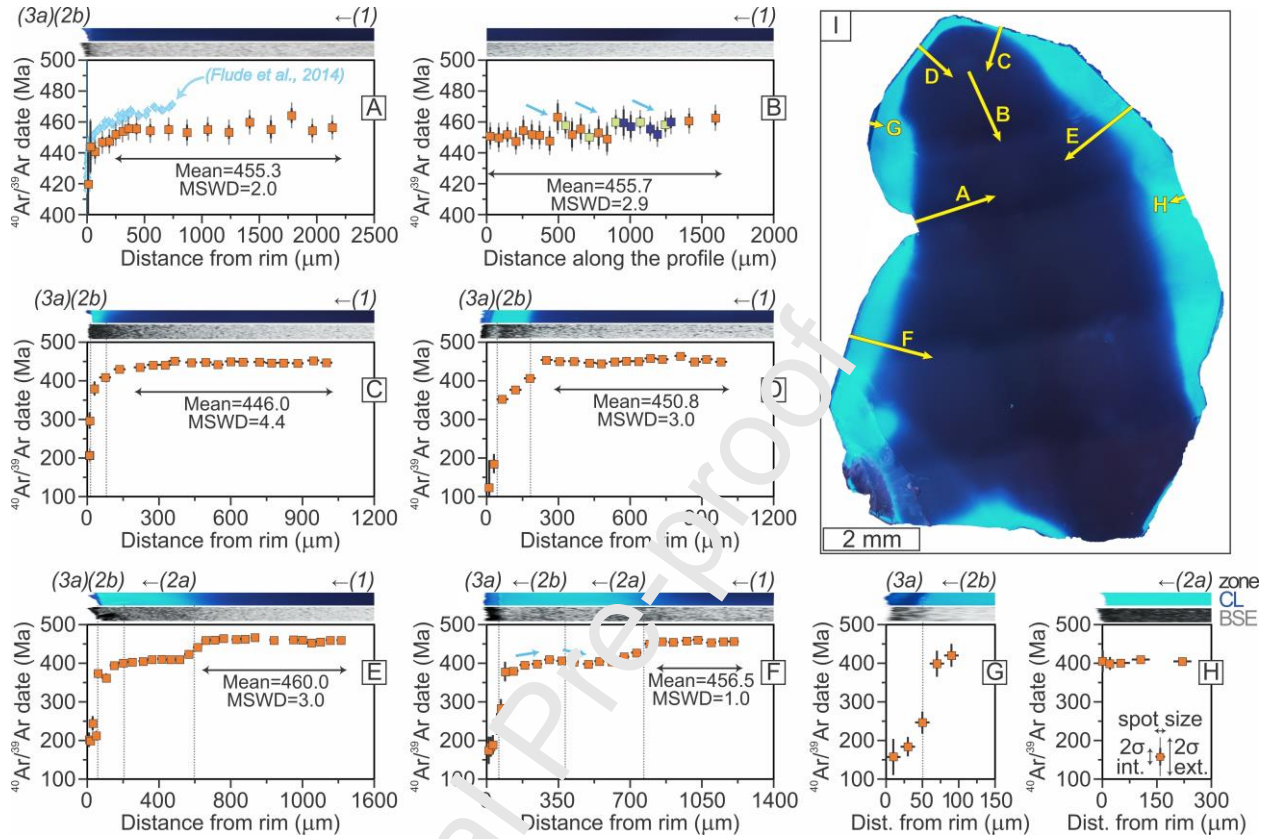
Fig. 5. In situ ^{40}\text{Ar}/^{39}\text{Ar} date profiles and their locations within the studied crystal of Itongay feldspar. A-H: plots showing the variations of in situ ^{40}\text{Ar}/^{39}\text{Ar} dates along the profiles. Strip profiles above the date plots show the variations of BSE and CL signals. These were used to locate the boundaries between the zones, which are shown with grey dotted lines and are labelled above the plots. Blue markers in Fig. 5A show the composite in situ ^{40}\text{Ar}/^{39}\text{Ar} date profile from (Flude et al., 2014). Their dates were recalculated using the decay constants of (Steiger and Jäger, 1977), which changed these dates by <0.1 Ma. Blue arrows in Figs. 5B and 5F indicate notable segments of the date profiles where the dates consistently increase or decrease with increasing distance from the rim of the crystal. The colour coded dates shown in Fig. 5B were obtained in a sequential order of light green, then orange, then deep blue, revealing their reproducibility. Weighted means and MSWD values shown in Figs. 5A-5E were calculated for intervals that are indicated with double headed arrows, internal uncertainties were used in
