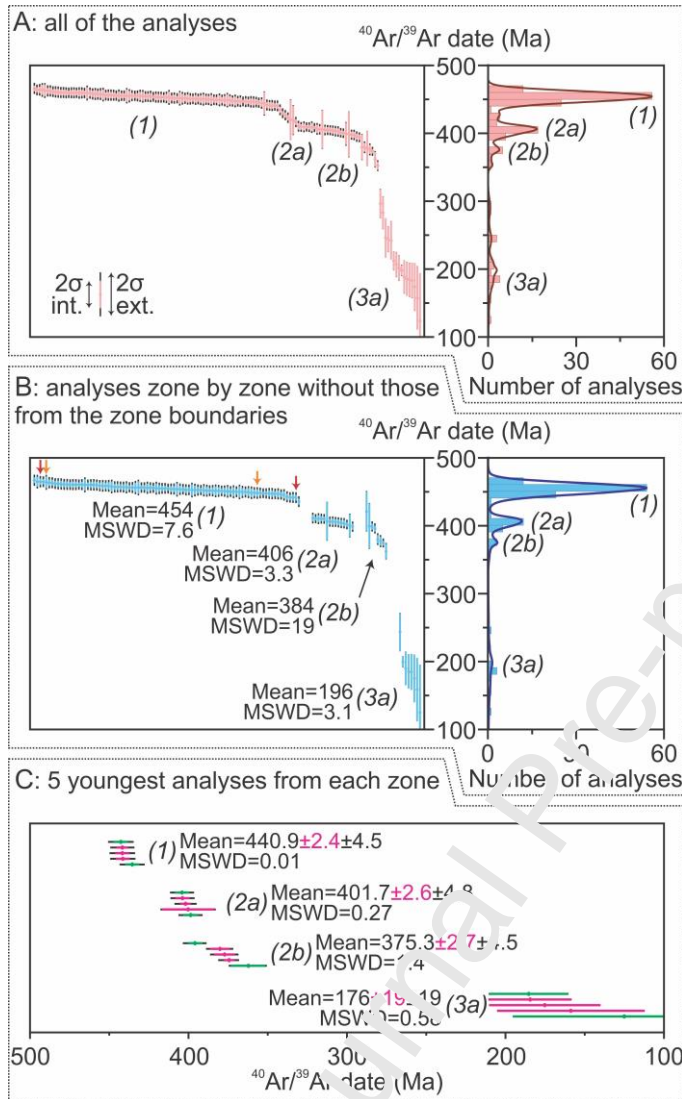
Fig. 6. A comparison of all of the in situ ^{40}\text{Ar}/^{39}\text{Ar} dates obtained in this work. A: all dates plotted in descending order along with a histogram and probability density function. B: dates from each (sub)zone plotted in descending order along with a histogram and probability density function. Weighted means were calculated for each of the (sub)zones. We have omitted dates that were obtained from the boundaries between the (sub)zones or proximal to these boundaries, as constrained using CL and BSE images, and these are also not included in the calculations of the weighted means. Brown and orange arrows show the youngest and the oldest dates in profiles A and B, respectively. C: the five youngest dates from each of the (sub)zones
