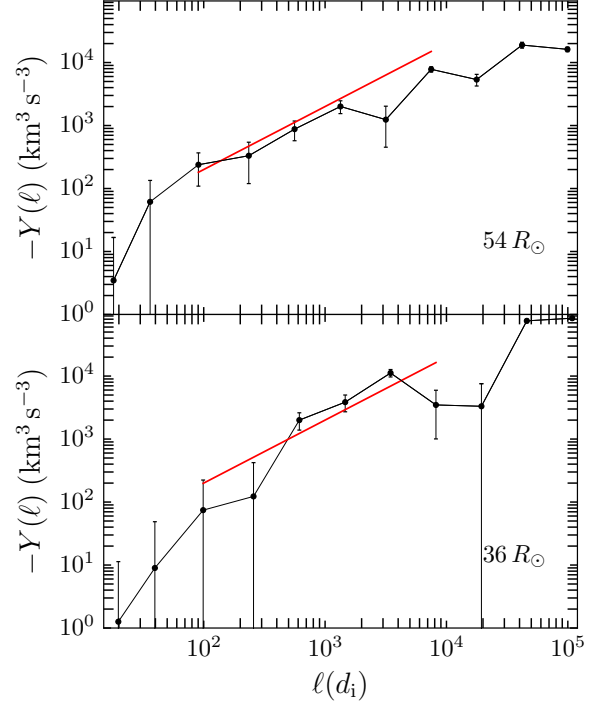
Figure 2. The scaling behavior of the third-order structure function as a function of the (Taylor shifted) length scale in units of ion-inertial length for two different periods we examined. Top: interval 02 on 2018 October 31, from 08:00:00 to 16:00:00 UTC; R = 54 R_{\odot} , Bottom: interval 20, near the Perihelion, 2018 November 06, from 08:00:00 to 16:00:00 UTC; R = 36 R_{\odot} . The thick red lines correspond to linear scaling laws for reference. The error bars are calculated by \sigma/\sqrt{m} , where \sigma is the standard deviation and m is the number of points used to calculate the mean.
