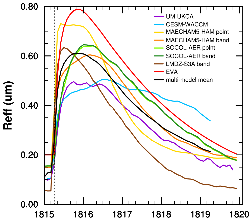
Figure 3: Global stratospheric mean effective radius ( R_{eff} ) time series. Vertical dotted line marks date of injection of SO_2 . The calculation of R_{eff} is weighted by surface aerosol density and gridcell volume, as explained in Appendix A.
