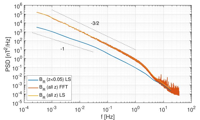
Figure 9. Power spectral density of the radial component B_R of the magnetic field for quiescent ( z < 0.05 ) and active (all z ) regimes. For the latter, we overplot the results obtained by using the Fast Fourier Transform (FFT) and the Lomb–Scargle (LS) method to confirm their good agreement.
