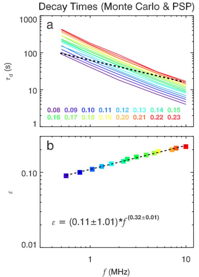
Figure 8. Comparison of Monte Carlo simulations and PSP observations. (a) Simulated decay times, \tau_d , as a function of the frequency for 16 levels of relative density fluctuations, \epsilon , in color. A dashed black line shows fitting results from PSP (Figure 6). (b) Relative density fluctuations, \epsilon , as a function of the frequency retrieved from intersections between Monte Carlo simulations and PSP observations. A dashed black line represents results of power-law fittings.
