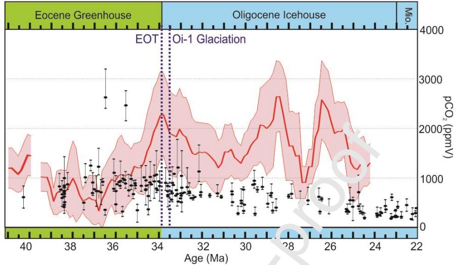
Fig. 3. Reconstructed CO_{2atm} using the standard soil paleobarometry approach. The CO_{2atm} values are reconstructed using R_s values of +0.0 \pm 130 \text{ gC/m}^2/\text{yr} (see text). Reconstructed CO_{2atm} values are close to CO_{2atm} data from marine proxies (black dots with error bars) during the 38-36 Ma window but climb above 1000 ppmV in the Oligocene, reaching values episodically up to 2500 ppmV, five times more than what is predicted by other proxies.
