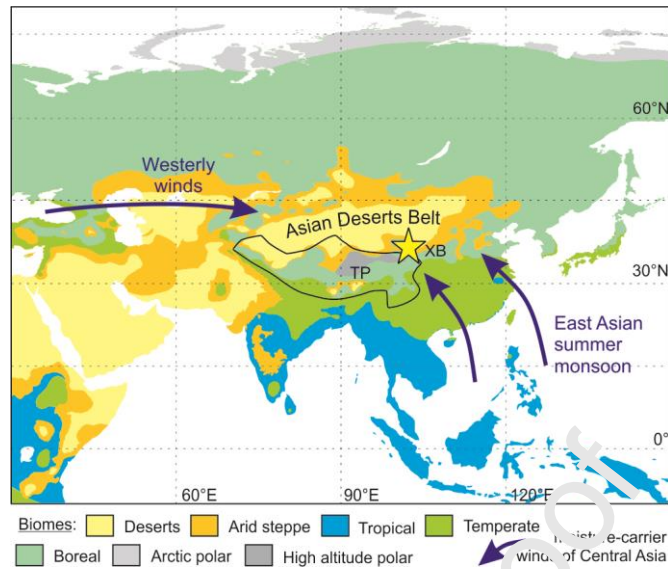
Fig. 1. Map of Asia and its different biomes (Peel et al., 2007), with location of the Xining Basin (XB) and Tibetan Plateau (TP, black line) and moisture-carrier wind directions feeding the Asian desert belts (blue arrows).
