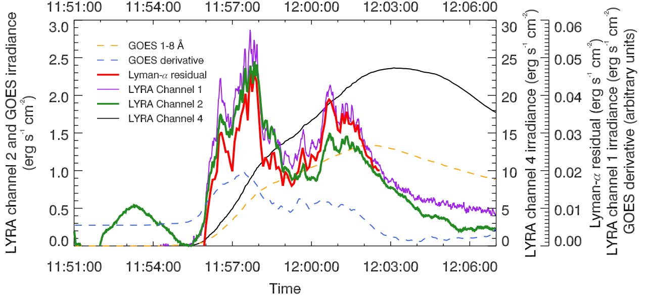
Figure 2. Solar irradiance during the X9.3 flare of 2017 September 6 (with the pre-flare irradiance subtracted), observed by GOES (orange line) and LYRA channels 1, 2 and 4 (respectively the purple, green, and black lines for E_1 , E_2 and E_4 ), as well as the Lyman- \alpha residual irradiance E'_1 (red line) extracted from E_1 . The LYRA data were rebinned to the cadence of 1 s. The time derivative of GOES 1–8 Å data is also shown (blue line) as a proxy of the non-thermal flare emission. Different scales were used for the various time series for the sake of clarity.
