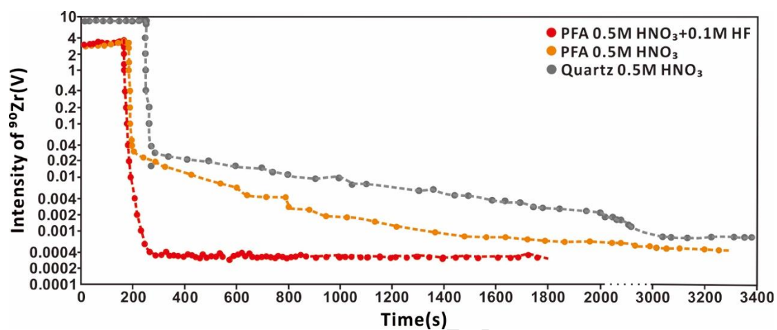
Figure 2 ^{90}\text{Zr} intensity as a function of time during washout of the 200ppb IPGP-Zr solution when using different acids and spray chambers. The difference of the intensity at the same concentration is due to PFA CSC has inferior sensitivity than quartz SIS.
