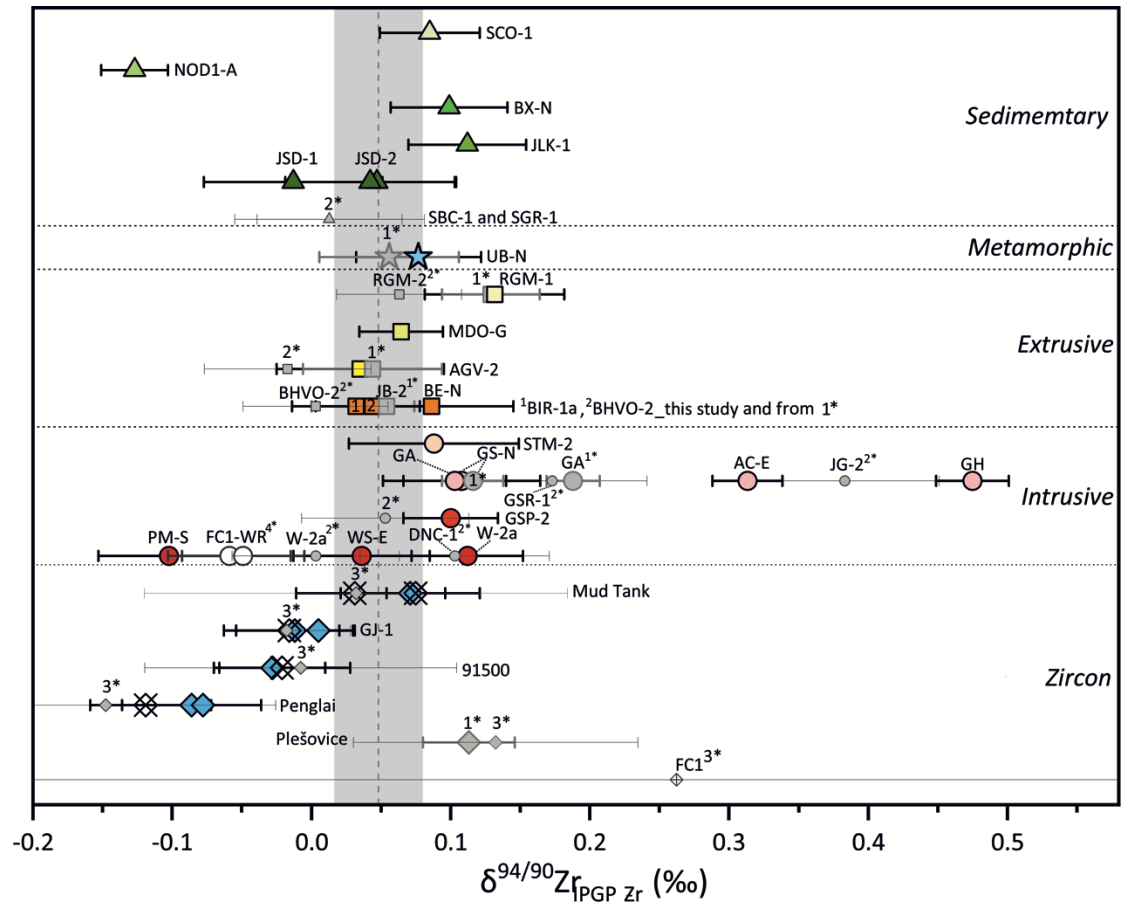
Figure 3 Zirconium isotopic compositions of whole rock and zircon reference materials. Error bars indicate 2SD uncertainties. Colorful symbols with black edge represent the data from this study, plus zircon symbols (diamonds) with cross representing unpurified zircons for distinction from their purified counterparts (diamonds with black edge). Literature data marked with * are from: 1. Inglis et al. (2018); 2. Feng et al. (2020); 3. Zhang et al. (2019); 4. Ibañez-Mejia and Tissot (2019). The gray band denotes \delta^{94/90}\text{Zr}_{\text{IPGP-Zr}} value of the upper mantle estimated by Inglis et al. (2019).
