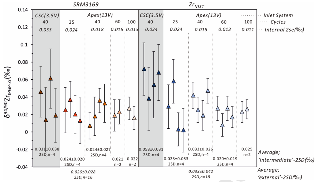
Figure 4 Zr isotope compositions of SRM3169 and NIST. CSC and Apex denote the two different inlet systems with brackets behind them including the signal on ^{90}\text{Zr}^+ . Error bars indicate 2se uncertainties within each block. Data can be found in Table S3.
