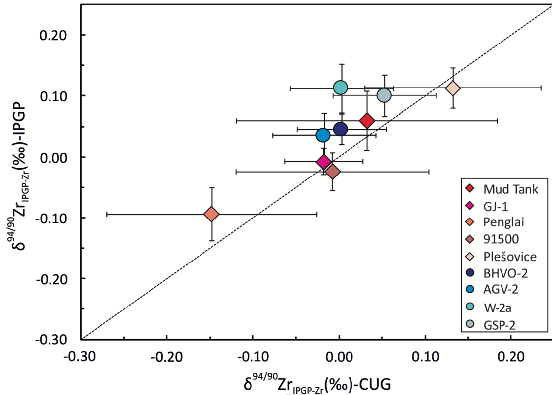
Figure 6 Interlaboratory comparison of Zr isotope compositions of zircons and RMs. The ordinate shows \delta^{94/90}\text{Zr}_{\text{IPGP-Zr}} measured on the MC-ICP-MS at the Institut de Physique du Globe de Paris (IPGP), among which the \delta^{94/90}\text{Zr}_{\text{IPGP-Zr}} value of zircon Plesovice is from Inglis et al. (2018) and others are reported in this study. The horizontal ordinate represents the data of zircon and RMs from Zhang et al. (2019) indicated by red-colored diamonds and Feng et al. (2019) denoted by blue-colored circles which were measured on LA-MC-P-MS and TIMS respectively (CUG denotes China University of Geosciences). The error bars indicate 2SD uncertainties.
