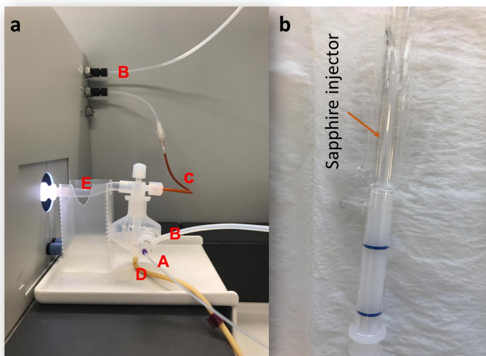
Figure 1 a. Savillex PFA cyclonic spray chamber (CSC) (no surface treatment, part number 820-01). Sample solutions are aspirated by sample gas (B) through the PFA-50 micro-flow nebulizer and assembled sample capillary (A). The make-up gas (C) improves the delivery of nebulizing sample solutions into the torch through the elbow connection (E). The waste droplets go down to the drain (D) at the bottom of the spray chamber. b. Thermo Injector Assembly with Sapphire Injector (1.8 mm ID, precleaned, 851-011-100708) in the torch.
