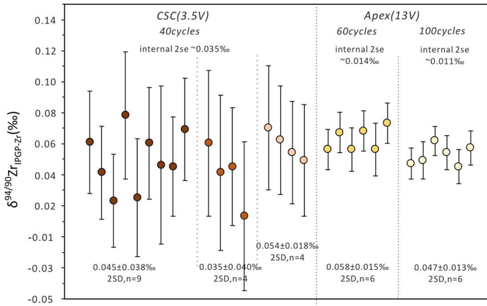
Figure 5 Zr isotope compositions of BHVO-2 analyzed at different conditions. Note that \delta^{94/90}\text{Zr}_{\text{IPGP}} values of BHVO-2 measured using CSC showed here are selected randomly from all the measurements because we just want to show the usual internal precision under this condition. Error bars indicate 2se uncertainties of every analysis. The data below the circles indicate the average values and their 2SD uncertainties of the measurements, n representing the number of replicates for one aliquot. Data can be found in Table S4
