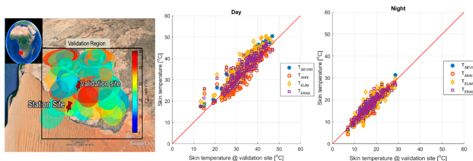
Figure 7. Comparison of IASI T_{\text{ANN}} , T_{\text{EUM}} , T_{\text{ERA5}} , and T_{\text{SEVIRI}} with ground observations at Gobabeb. Left: station and validation site locations with a one-month example of IASI-coincident observations; middle panel: T_{\text{ANN}} versus in situ T_{\text{skin}} during the day; and right panel: during the night for all coincident observations in 2016.
