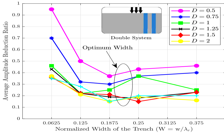
Figure 15: Influence of normalized barrier width on \bar{A}_r ( X = 0.5 )
