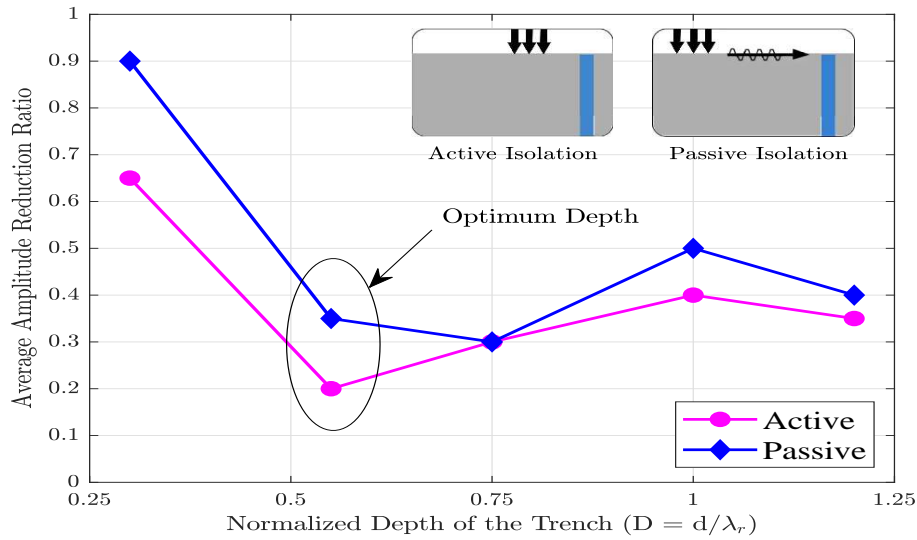
Figure 7: Influence of normalized barrier depth on \bar{A}_r ( X = 0.5 )
