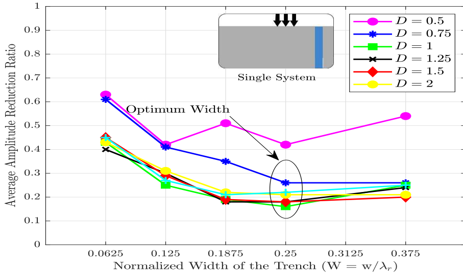
Figure 13: Influence of normalized barrier width on \bar{A}_r ( X = 0.5 )
