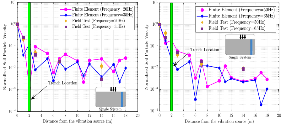
Figure 9: Validation of numerical modelling based on the result of field test, active isolation, (D=3m, W=0.25m, L=10m, X=2m)
