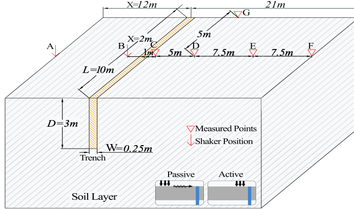
Figure 3: Measuring arrangement
