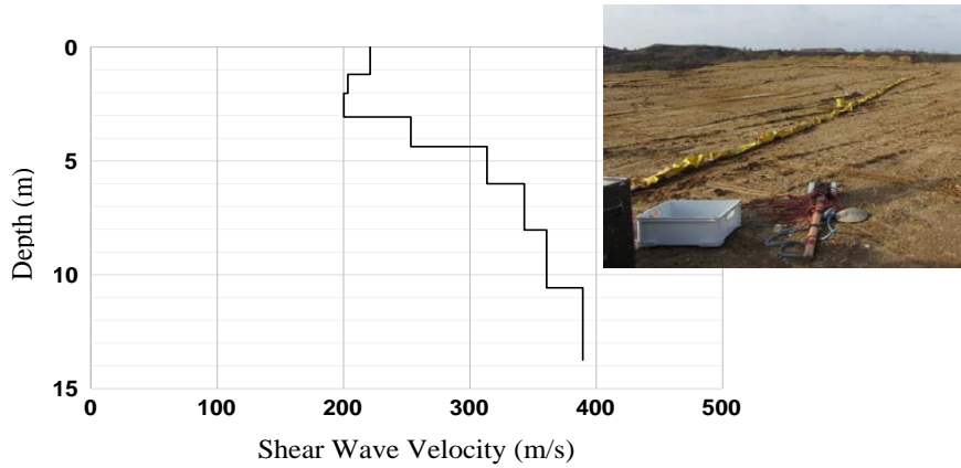
Figure 1: Shear wave velocity profile of the site
