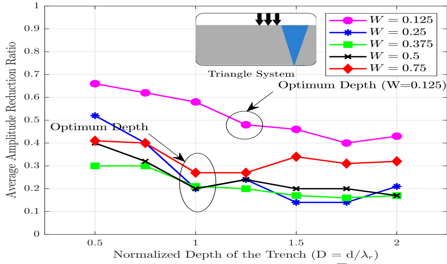
Figure 16: Influence of normalized barrier depth on \bar{A}_r ( X = 0.5 )
