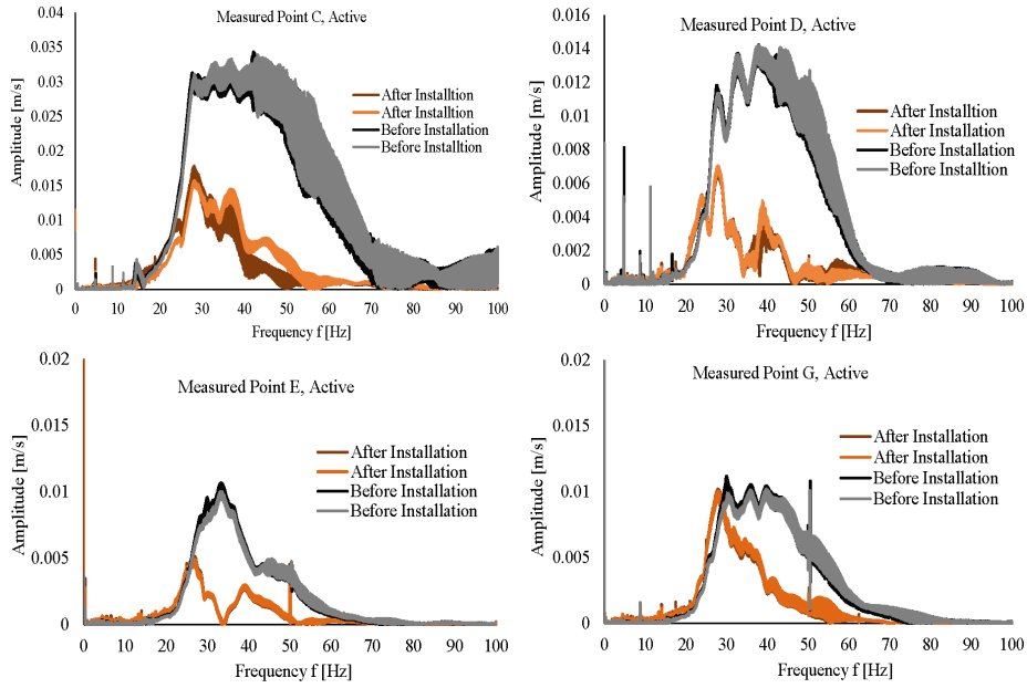
Figure 5: Representation in the frequency domain: Measuring points C, D, E, G (Active Isolation)
