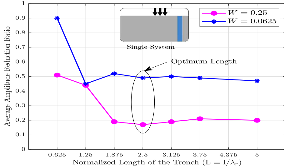
Figure 11: Influence of normalized barrier length on \bar{A}_r ( X = 1.25 , D = 1.25 )
