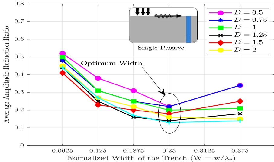
Figure 18: Influence of normalized barrier width on \bar{A}_r ( X = 3 )
