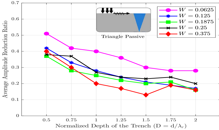
Figure 20: Influence of normalized barrier depth on \bar{A}_r ( X = 3 )
