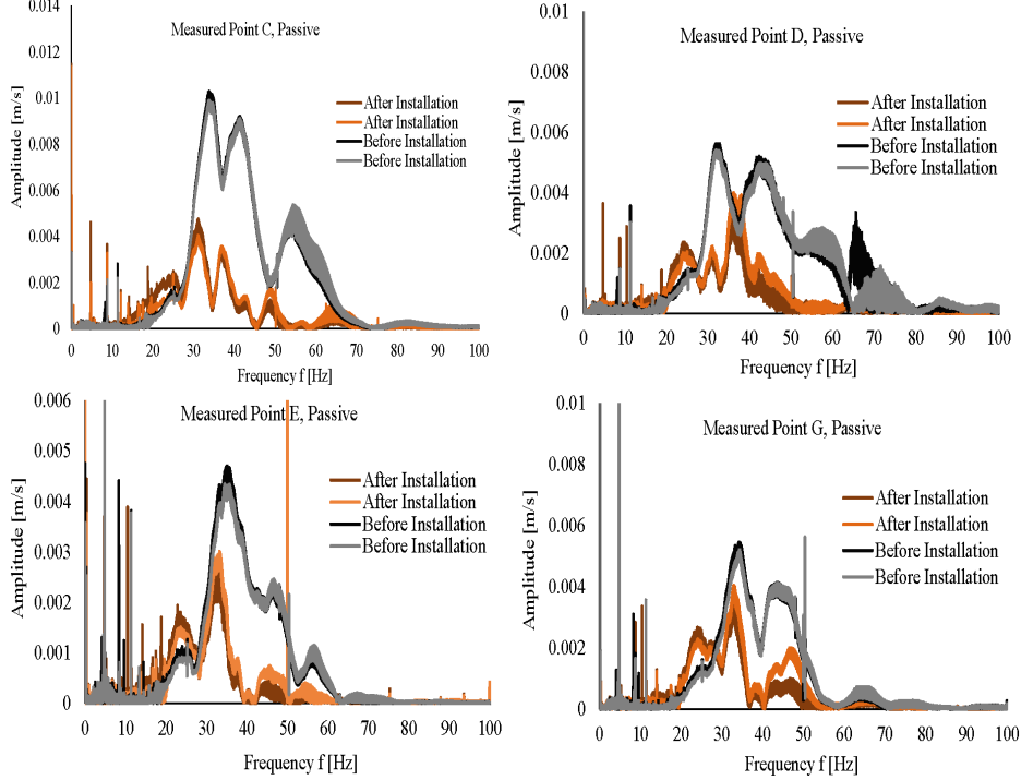
Figure 6: Representation in the frequency domain: Measuring points C, D, E, G (Passive Isolation)
