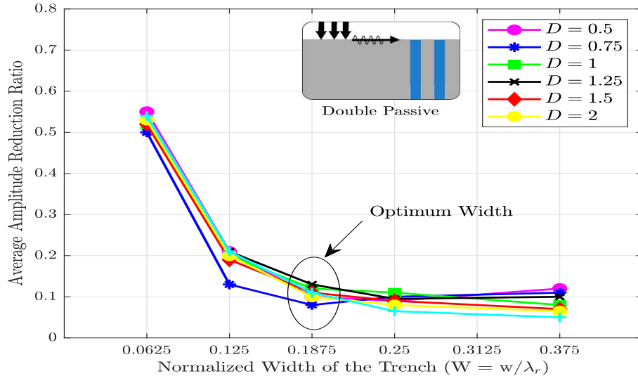
Figure 19: Influence of normalized barrier width on \bar{A}_r ( X = 3 )
