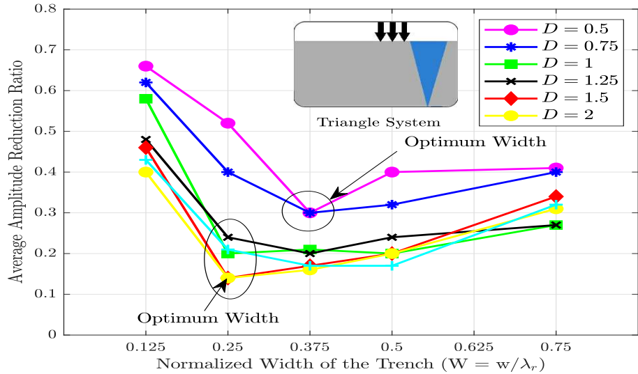
Figure 17: Influence of normalized barrier width on \bar{A}_r of EPS Geofoam wave barrier ( X = 0.5 )
