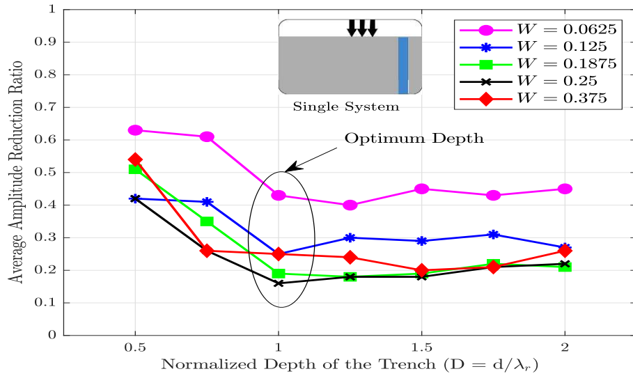
Figure 12: Influence of normalized barrier depth on \bar{A}_r ( X = 0.5 )
