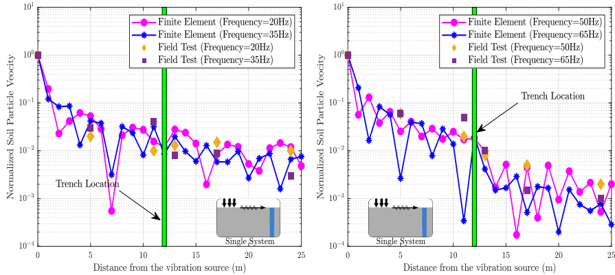
Figure 10: Validation of numerical modelling based on the result of field test, passive isolation (D=3m, W=0.25m, L=10m, X=12m)
