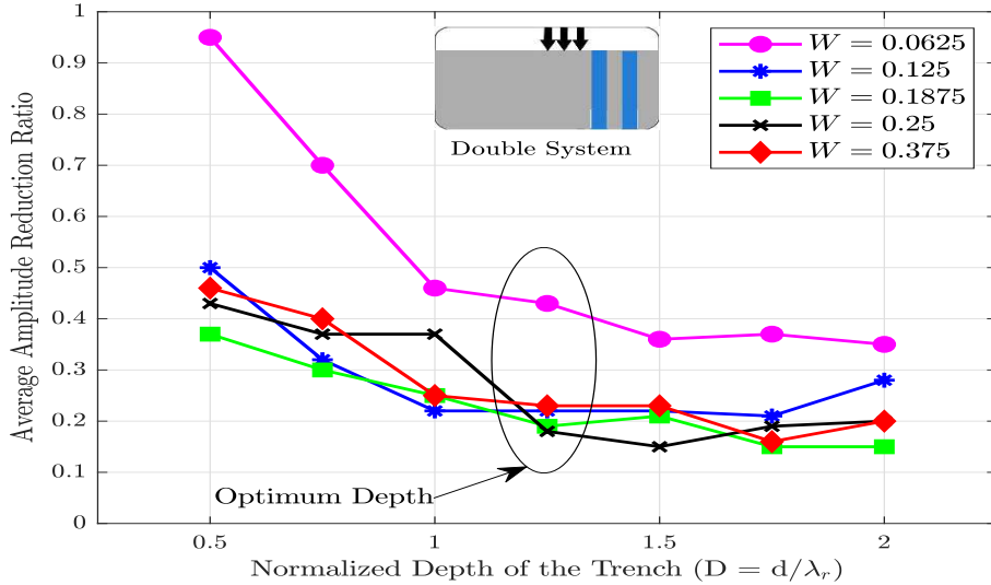
Figure 14: Influence of normalized barrier depth on \bar{A}_r ( X = 0.5 )
