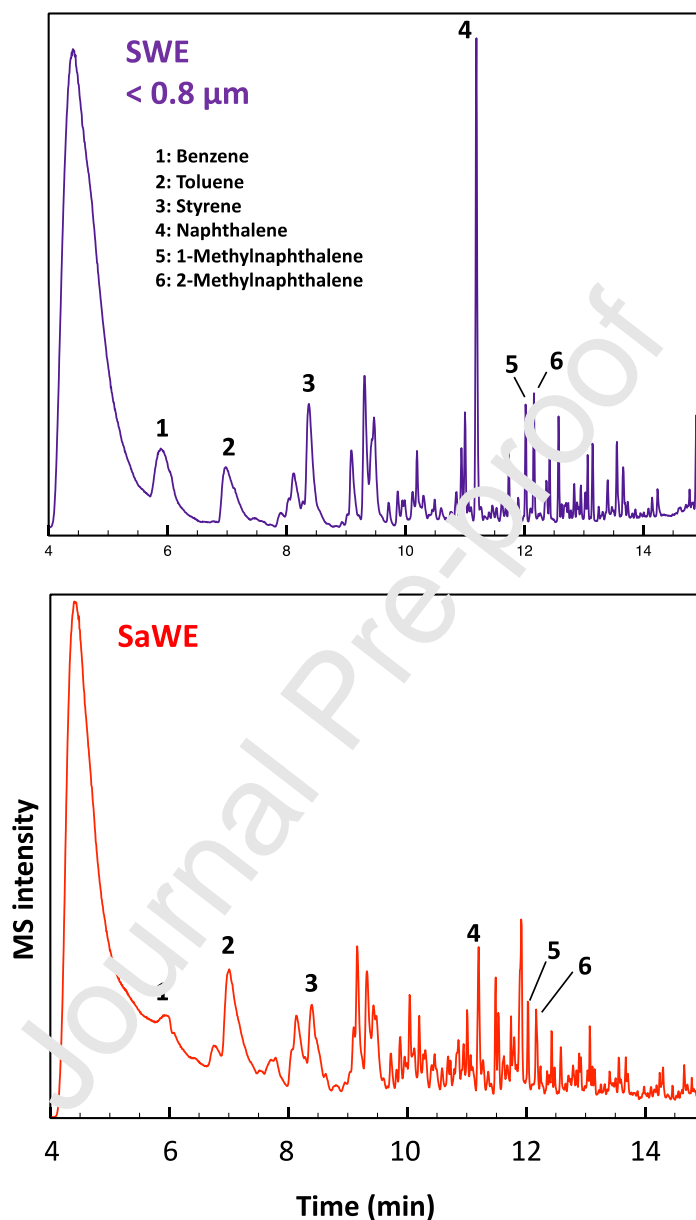
Figure 4. Total ion chromatogram obtained for the <0.8 μm fractions of the SWE and the Sargassum water extract (SaWE).
