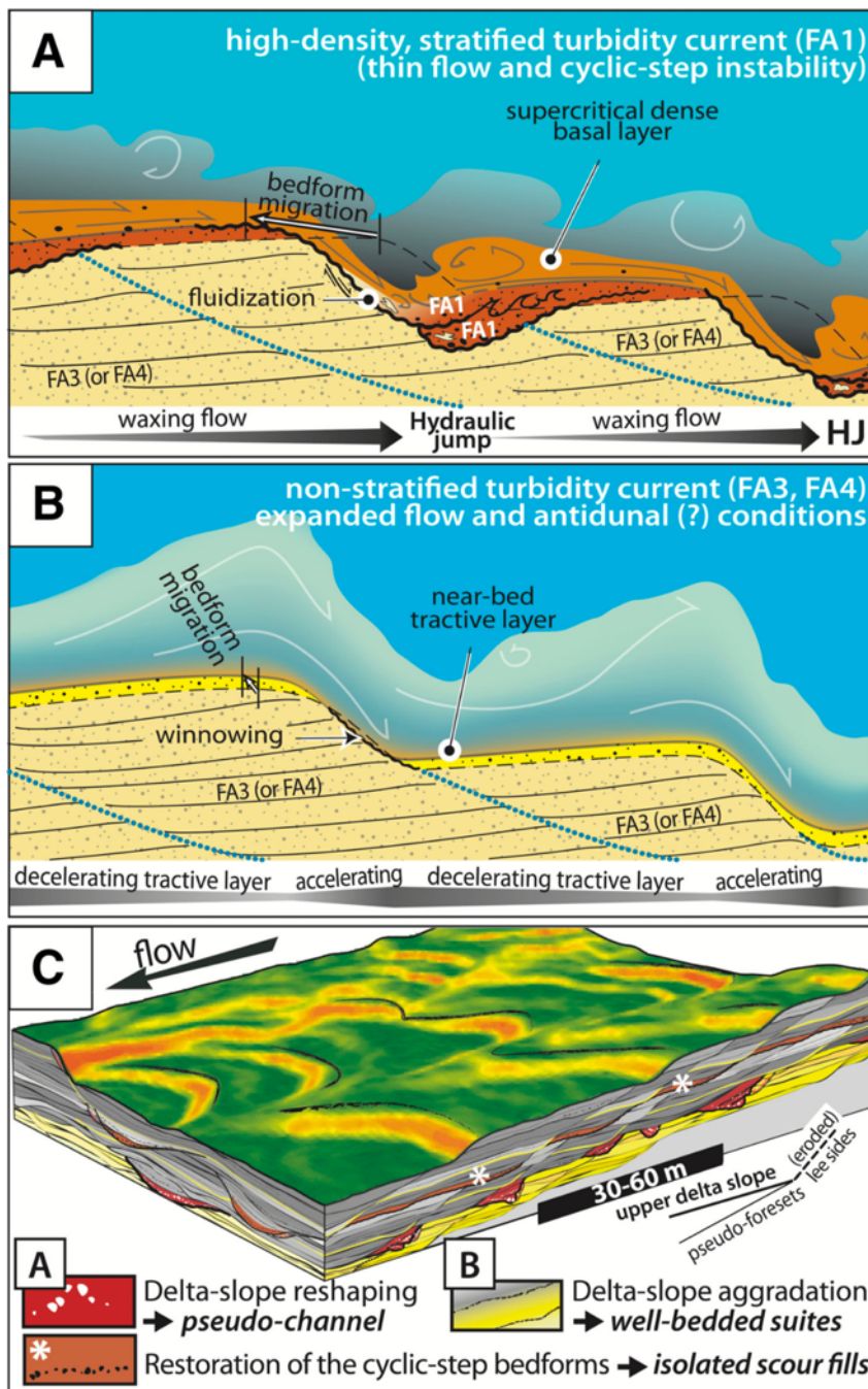
Fig. 15. The depositional signature of cyclic-step instabilities. (A) Cyclic steps, which lead to episodes of significant delta-slope reshaping, truncate earlier deposits (FA3 and FA4) and intervening pseudo-foresets (cf. Fig. 15B). They are interpreted to develop in association with the supercritical basal layer of dense (stratified) turbidity currents, here represented in orange. The depositional record of cyclic steps, constituting chiefly the infill of pseudo-channels, is interpreted as the result of “cyclic-step flow events”. Such events encompass a tract of flow conditions from the fully erosional cyclic steps that might have developed in an initial flow stage (not shown) up to late waning-flow conditions. They must include flow conditions corresponding to partially depositional cyclic steps sensu Slooman and Cartigny (2020) and to other transient flow stages such as antidunes (FA1 and FA2, respectively). (B) Successions of short-lived, expanded (non-stratified) turbidity currents, possibly under antidunal conditions, are suggested to explain the aggradation of top-cut-out turbidites forming well-bedded
