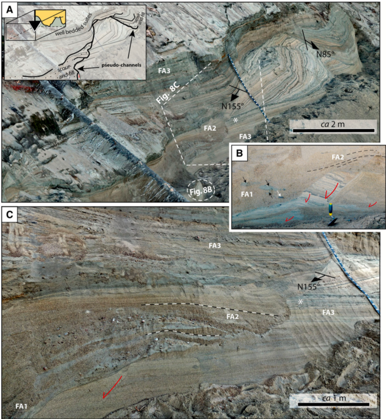
Fig. 8. Pseudo-channels and related deposits (see location in Fig. 5). (A) Oblique plan view drone image, palaeocurrent towards the observer; coarse brown sand prevails in pseudo-channel fills, while lighter sand characterizes the underlying truncated deposits (dip orientations of pseudo-channel margins are noted). (B) Structureless coarse sand containing pebbles (FA1, lower part; black arrows: rip-up mud clasts; white arrow: basement clast) and passing to faintly laminated (FA2, upper part, dashed lines). FA1 and FA2 deposits onlap translated sand masses (including bioturbation), the original position of which was found 2 m higher and 4 m upslope (white stars in A and C). These translated sand masses underline the erosion margin of the pseudo-channel (see also Fig. 5). (C) Coarse to pebbly sand that shows an assemblage of convex-up to undulating laminae (FA2). Dashed black-white lines highlight individual laminae that thicken upstreamward. Red arrows indicate small extensional faults.
