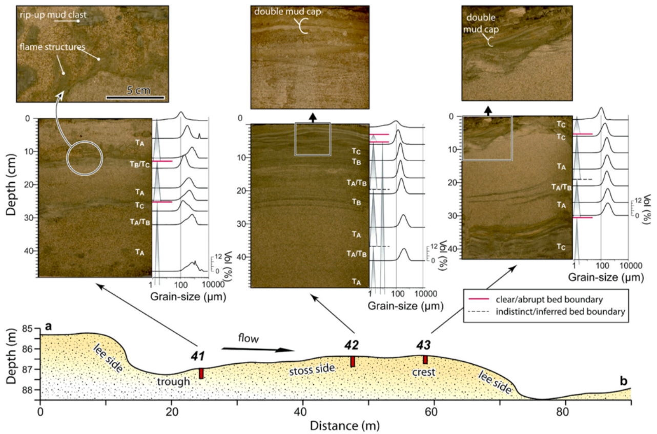
Fig. 14. Cross-sections —and close-up views— collected near the trough, on the middle stoss and on the crest of a single cyclic-step bedform illustrating the variation in sedimentary facies (location map in Fig. 13A; Southwind Fjord delta slope, Baffin Island). The trough consists of poorly-sorted gravel and sand with rip-up mud clasts while the stoss and crest consist of top-cut-out turbidites with T A , T B (T B-1 or T B-2 ) and T C subdivisions. Vertical and lateral grain-size distributions are given. The close-up view of sample 41 is from a cross-section distinct from the one that is illustrated here. To be compared with Figs 7C, 8B, 9 to 11 from the Portneuf-Forestville case study.
