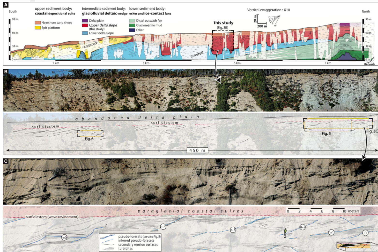
Fig. 3. Depositional architecture of the Portneuf-Forestville deltaic complex. (A) Interpreted depositional units, redrawn from Dietrich et al. (2017b). The case study is comprised within the upper delta-slope deposits (red colour) belonging to the intermediate sediment body. (B) Photomosaic of the study area (location in A) with locations of some other zoomed-in figures. (C) Orthophotomosaic of the northern segment of the study area, essentially showing a cyclic alternation of well-bedded suites and up to 6 pseudo-foresets (n to n+5; see Fig. 5 for a detailed description; no vertical exaggeration except for A).
