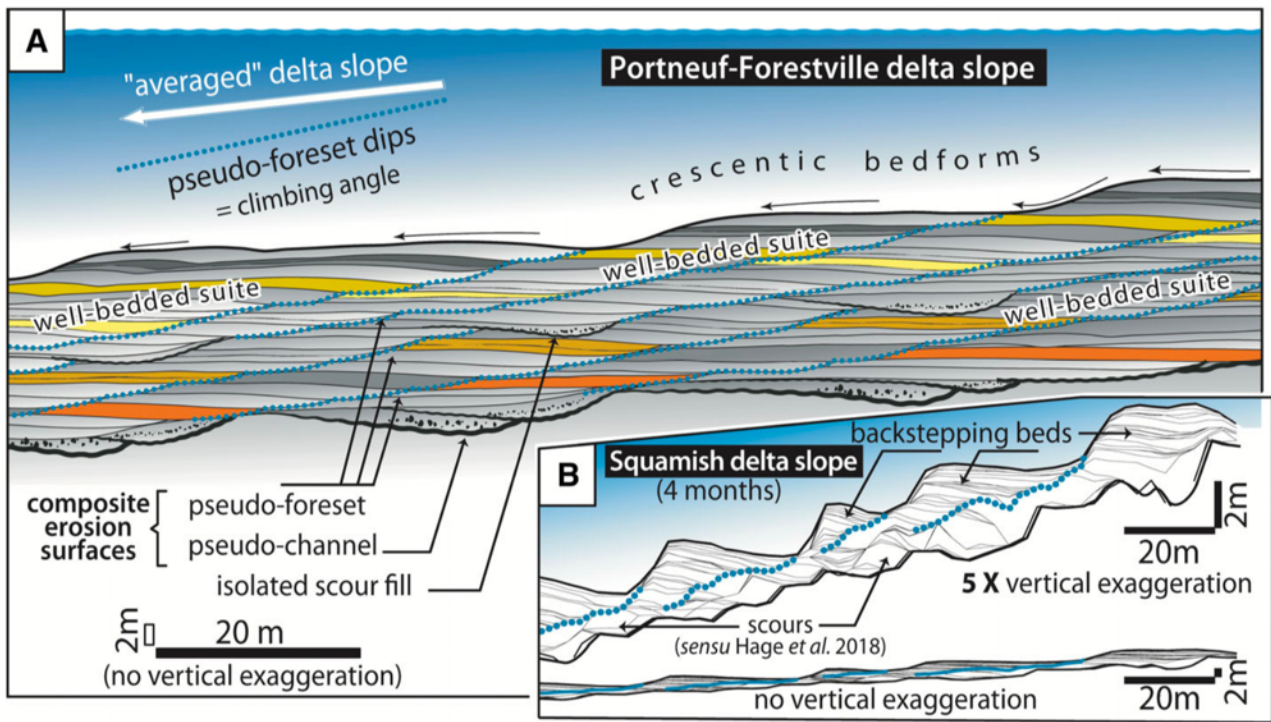
Fig. 12. Stratigraphic patterns in proglacial delta-slope sands involving cyclic steps. (A) Conceptual model showing the relation of well-bedded suites to aggrading, asymmetrical bedforms migrating upslope along the fossil upper delta slope of the Portneuf-Forestville complex. Grey horizons represent the layout of turbidites (laminae not shown), four of which have been coloured to highlight discontinuous, yet synchronous layers. Resulting well-bedded suites are interrupted by composite erosion surfaces in the sense of Slooman and Cartigny (2020), here referred to as pseudo-foresets (blue dotted lines) and representing retrogressive climbing planes showing ca 12° dips (10 to 20° in Fig. 3). The original, "averaged", delta slope, with significant lesser dips ( ca 6°), is poorly identifiable from this stratal pattern (see also grey dotted lines in Fig. 5). (B) For comparison, the stratigraphy reconstructed from a 4-month repeat swath bathymetry survey in the Squamish delta (redrawn from Hage et al. , 2018). Backstepping beds evidenced owing to vertical exaggeration are analogous to the here-described well-bedded suites (see Fig. 11). Pseudo-foreset geometries are here also identifiable (blue dotted lines). In both cases (A and B), pseudo-channel/scour infills prevail in the lower part of the succession.
