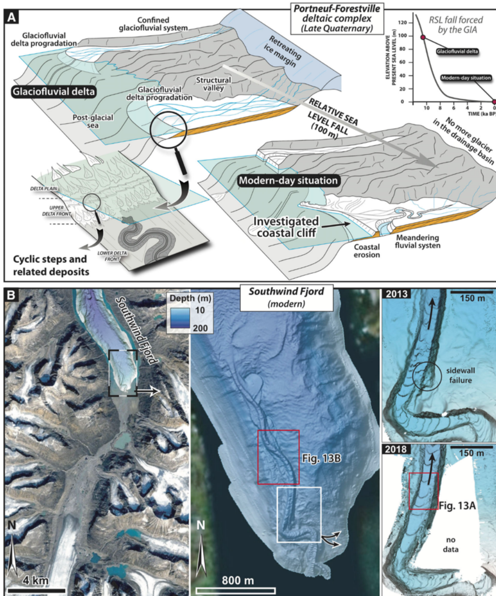
Fig. 2. Depositional settings (locations in Fig. 1). (A) 3D diagram illustrating the late Quaternary development of the Portneuf-Forestville deltaic complex (Québec North Shore; location in Fig. 1); the sediment wedge deposited in front of a retreating continental ice margin is currently uplifted owing to the glacio-isostatic adjustment. Largely dissected by present-day coastal erosion, it offers a 7 km long, up to 85 m high depositional transect including the here-studied delta-slope sands (Fig.3A; see also Dietrich et al. , 2017b, 2020). (B) The proglacial context of the Southwind Fjord (Cumberland Peninsula, SE Baffin Island) and detailed bathymetric maps (2013 and 2018, localized by the white box) of the Southwind Fjord delta slope. Red frames are locations related to Fig. 13A and B.
