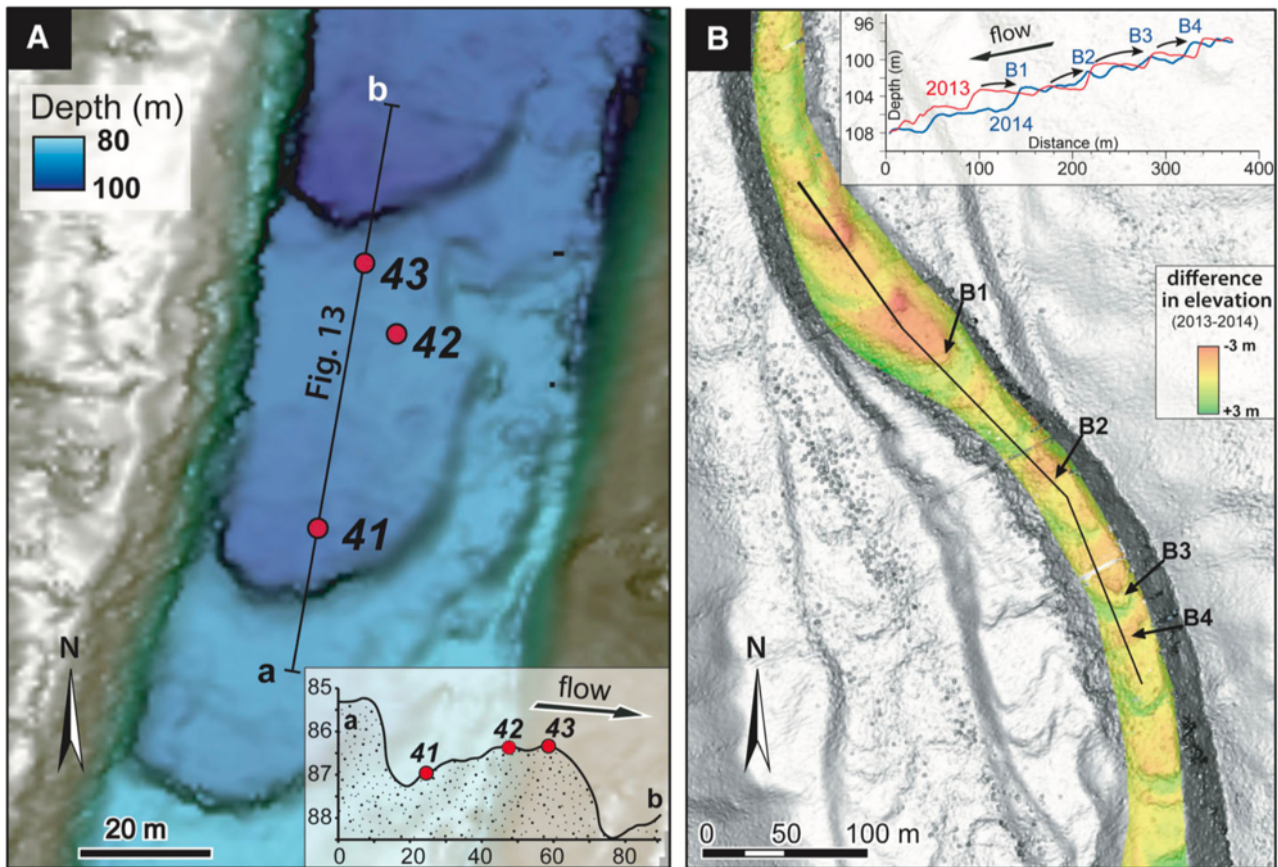
Fig. 13. Cyclic steps observed in a submarine channel of a modern turbiditic system (Southwind Fjord delta slope, Baffin Island). (A) Location of IKU grabs on a single cyclic step (location in Fig. 2B). (B) Difference in elevation between two surveys (2013 and 2014, location in Fig. 2B) in the lower part of the channel system illustrating erosion of the lee side and the deposition on the stoss side of four active bedforms labeled B1 to B4. This erosional/depositional pattern leads to the upslope migration of the crescentic bedforms, interpreted as cyclic steps.
