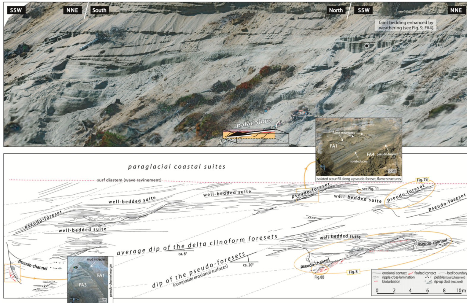
Fig. 5. Orthophotomosaic of a northern portion of the study area (see location in Fig. 3B) and its interpretation, differentiating the main bed boundaries and intervening erosion surfaces and showing relationships between pseudo-foresets, well-bedded suites and pseudo-channels. These deposits are truncated by a gravelly lag interpreted as a surf diastem reflecting forced regression (Dietrich et al. , 2017b). The low-angle and steeper grey dotted lines highlight the inferred “average” dip of the delta clinoform foreset and the dips of the pseudo-foresets, respectively. Insets show a pseudo-channel margin (lower left) and an isolated scour fill and associated cyclic-step deposits with sheared flame structures (upper right).
