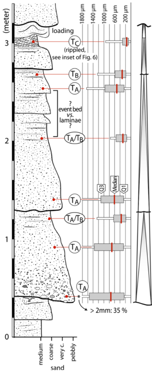
Fig. 10. Layout of eight sand samples collected in thick turbiditic beds (FA1; location in Fig. 6). Note that discriminating sand beds from thick laminae may be challenging (interval 2 to 2.6 m). A subdivision in three fining-up turbidites is proposed, which further shows an overall fining-up trend, culminating with a well-developed T c subdivision showing climbing-ripple cross-lamination (see inset in Fig. 6). Only the basal sample has a significant coarse fraction >2 mm (35 % in weight).
