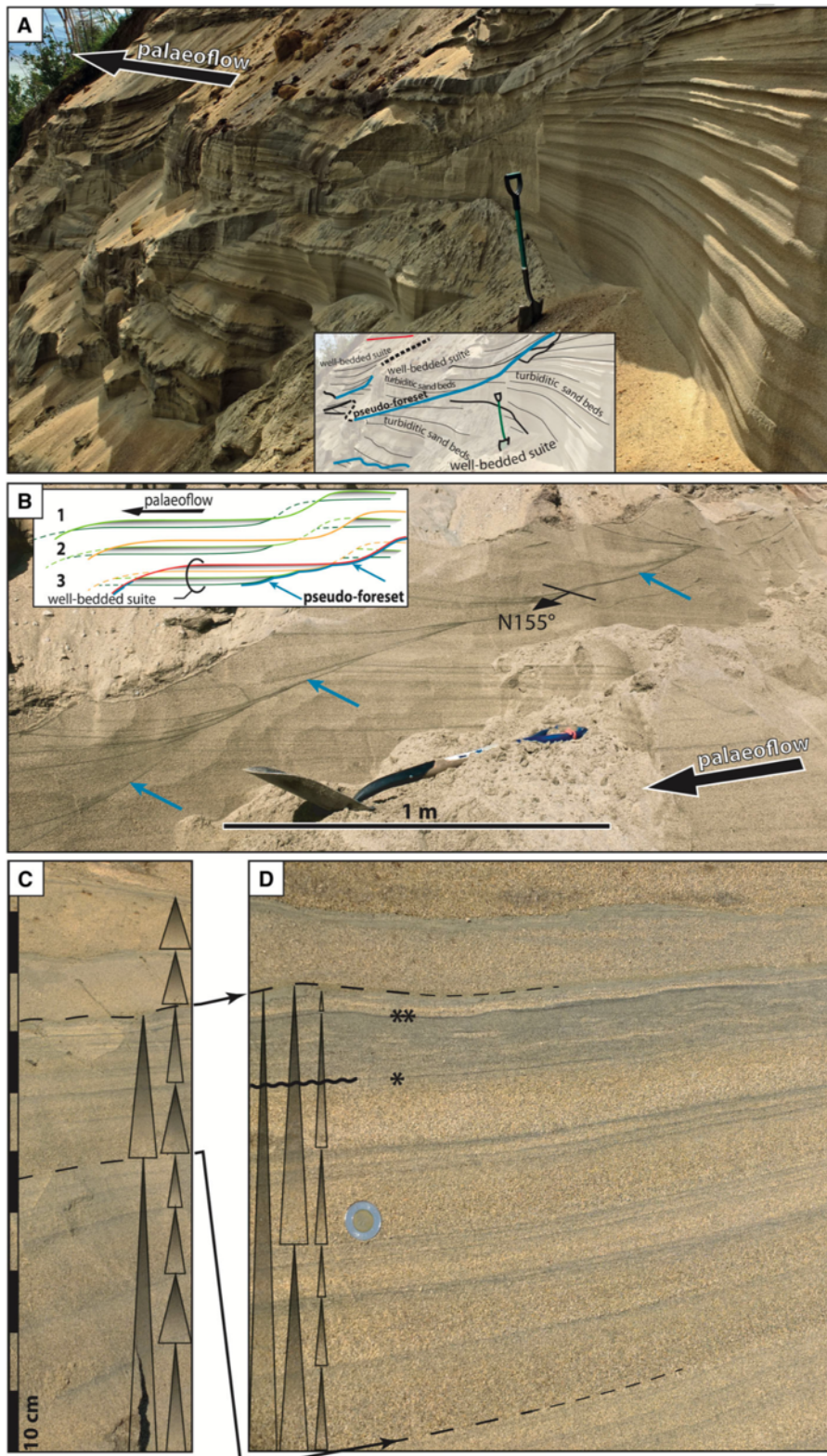
Fig. 7. Well-bedded suites and related depositional structures. (A) Oblique view of two adjacent well-bedded suites bounded by a pseudo-foreset (1 m long shovel for scale). Note that the laminae on the right-hand side of the photograph would appear on a cleaned outcrop akin to those illustrated in (D). (B) Detailed view on an upper segment of a pseudo-foreset (location in Fig. 5), corresponding to a superimposition of successive, spoon-shaped, small-scale scours highlighted by dark heavy mineral layers (inset shows time series detailing the formation scenario; see also Slotman and Cartigny, 2020). (C) and (D) the bed stacking pattern in well-bedded suites (FA3), consisting of elementary turbiditic cm- to dm-thick, fining-upward, sand beds (top-cut-out turbidites), which are themselves organized in a hierarchy of fining- and thinning-upward bed sets. T_A (massive) and T_B (planar lamination, T_{B-2} and/or T_{B-1} in the sense of Talling et al. , 2012) subdivisions are mainly evidenced, with subordinate rippled fine-grained to muddy sand ( T_C ). Note in (D) some dark heavy mineral layers suggesting lag processes at a within-bed grain-size break (*) or capping a T_C subdivision (**).
