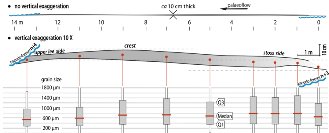
Fig. 11. Layout of nine sand samples collected along a single ca 10 cm thick turbidite from a well-bedded suite (FA4, essentially a T A subdivision) located between pseudo-foresets n+3 and n+4 of Fig. 3C (see also location in Fig. 5). Samples show a subtle downcurrent fining trend along the stoss side, which becomes clearer beyond the bedform crest along the upper lee side. Note the subhorizontal bed conformation, which appears as a backstepping bed only if a vertical exaggeration is applied (see also Fig. 12).
