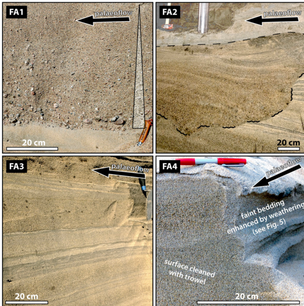
Fig. 9. Archetypal lithofacies and facies associations. FA1: Structureless sand and gravel (see also Figs. 8B and 10); FA2: Coarse sand with undulating lamination (see also Fig. 8C); FA3: Top-cut-out turbidites (see also Fig 7C and D); FA4: Amalgamated top-cut-out turbidites (see also Fig. 10). FA1 and FA2 characterize the pseudo-channel infills while FA3 and FA4 typify the well-bedded suites, which however also include in places subordinate FA1 and/or FA2 occurrences (Fig. 5; Table 2). FA1 and FA2 deposits are linked to cyclic-step instabilities in a stratified turbidity currents (peak- to waning-flow conditions); FA3 and FA4 deposits are interpreted as the result of expanded turbidity currents. See Discussion and Figs 15 and 16.
