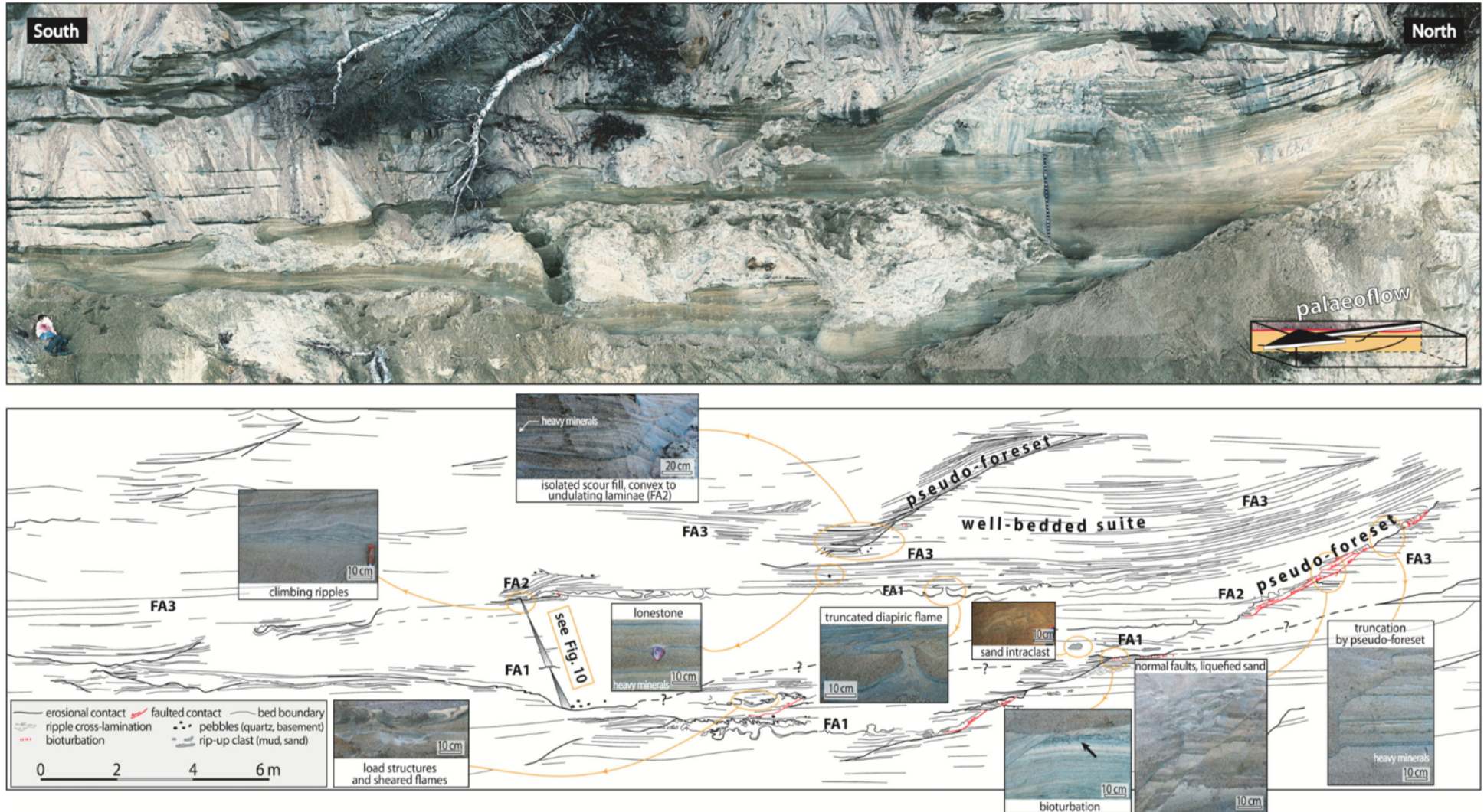
Fig 6. Orthophotomosaic of a southern portion of the study area (see location in Fig. 3B) and, below, its interpretation, differentiating the main bed boundaries and intervening erosion surfaces and showing relationships between pseudo-foresets, well-bedded suites and pseudo-channels. Contorted bed boundaries correspond to generalized load and flame structures associated with FA1 deposits. Note that the entire sand wedge including the fining-up succession of Fig. 10 onlaps toward the right some large scours and associated small-scale gravitational slides highlighted by red arrows. Insets offer a summary of sedimentary and deformation structures observed in the glaciofluvial delta-slope sands of the Portneuf-Forestville complex.
