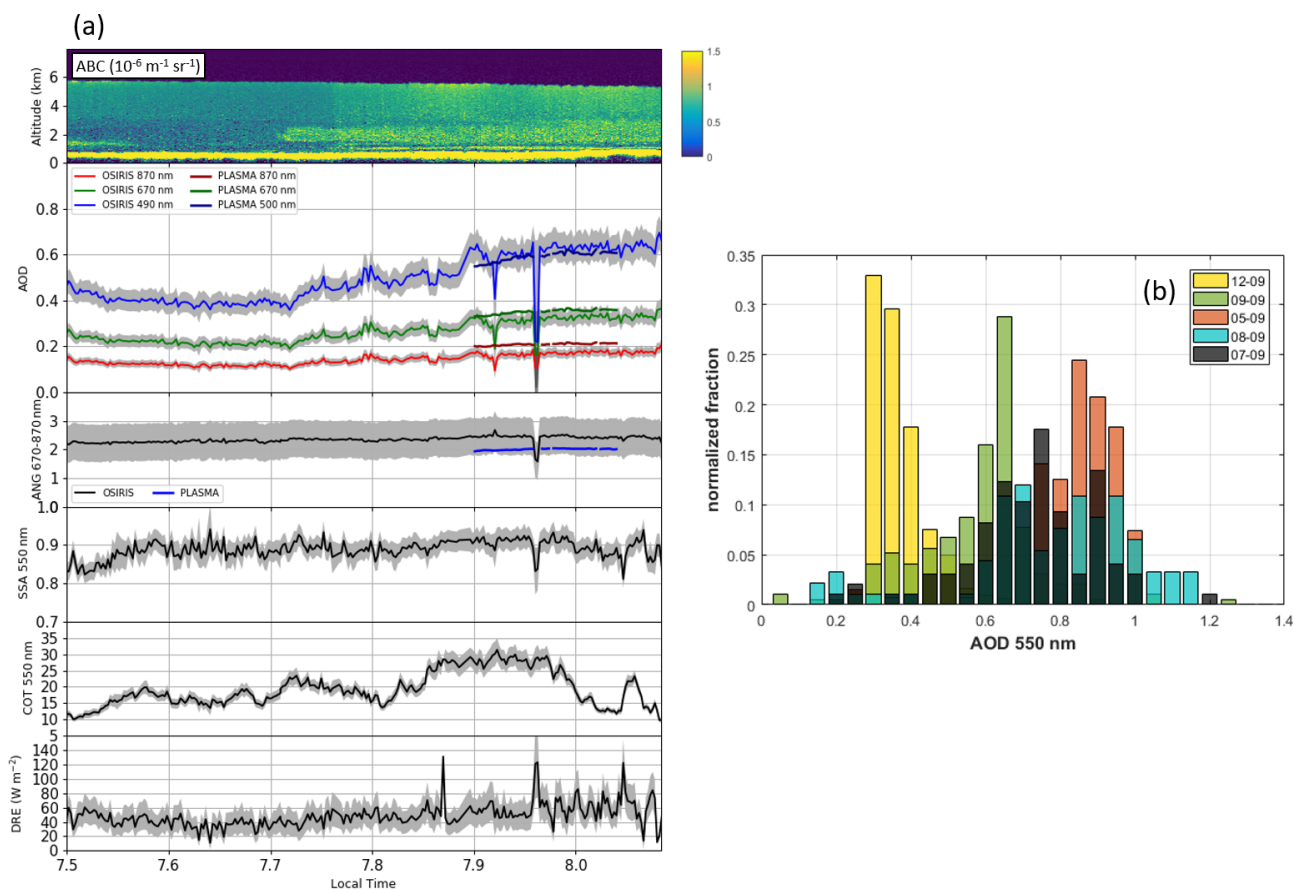
Figure 7. (a) Time series of the ABC profiles measured at 1064 nm by the lidar LNG, above-cloud AODs, Ångström exponents (670–870 nm), aerosol SSA, cloud optical depth and direct radiative effect estimated on 12 September 2017, and associated errors. (b) AOD histograms from OSIRIS measurements for the five selected flights.
