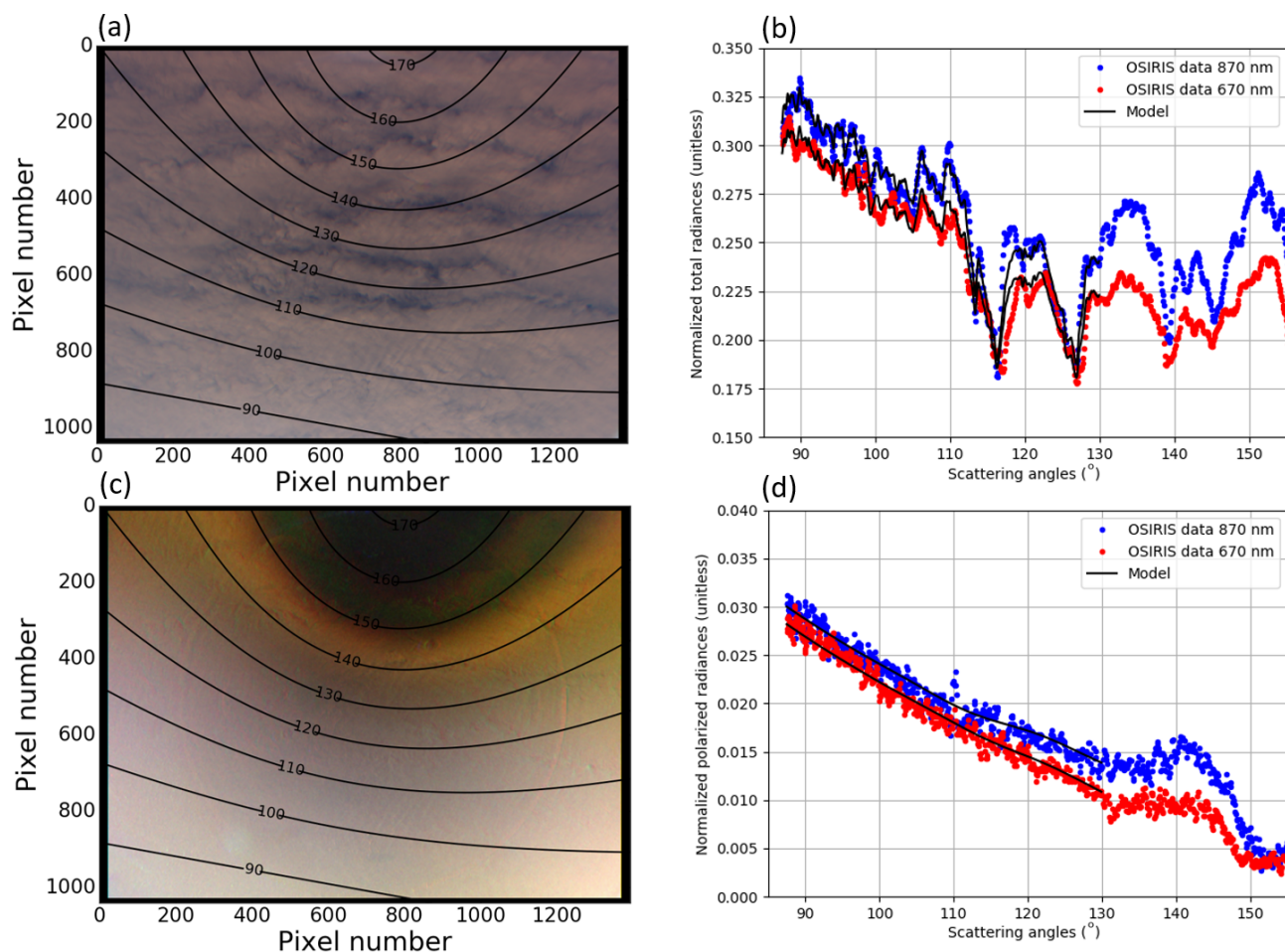
Figure 3. Total and polarized radiances measured by OSIRIS during 8 September 2017. Panels (a) and (c) represent the total, on the top, and the polarized, on the bottom, recomposed RGB radiances for the full OSIRIS image. Panels (b) and (d) represent the corresponding principle planes at 670 (red) and 870 nm (blue), respectively. OEM simulations, according Waquet et al. (2013a), of the total and polarized radiances for scattering angles below 130^\circ are represented with black lines in the panels (b) and (d). The main aerosol properties retrieved for this case are AOD equal to 0.74 at 670 nm, \alpha_{490-870} = 1.82 , and SSA equal to 0.87 at 670 nm.
