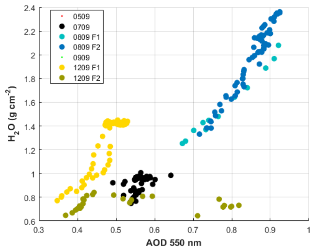
Figure 10. Column water vapour in a function of AOD at 550 nm, both measured by the PLASMA2 sun photometer during the AEROCLO-sA campaign.
