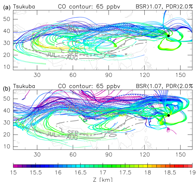
Figure 4. Kinematic backward trajectories for 10 d starting from Tsukuba in the 390–410 K potential temperature range at 100 m geopotential height intervals on all days during July–September 2018 on which measurements were made using ERA5 reanalysis data. Cases are sorted into two categories: (a) with and (b) without enhanced aerosol signals observed by lidar at the trajectory starting points. The conditions and number of trajectories for the former and the latter cases are respectively BSR > 1.07 and PDR > 2.0 % with 78 trajectories and BSR < 1.07 and PDR < 2.0 % with 136 trajectories. Colours indicate geopotential height ( Z ) values of the trajectories. Grey contours indicate 65 ppbv monthly mean CAMS CO levels at 400 K potential temperature, roughly indicating monthly mean boundaries of the ASM anticyclone (dotted for July, solid for August, and dash-dotted for September).
