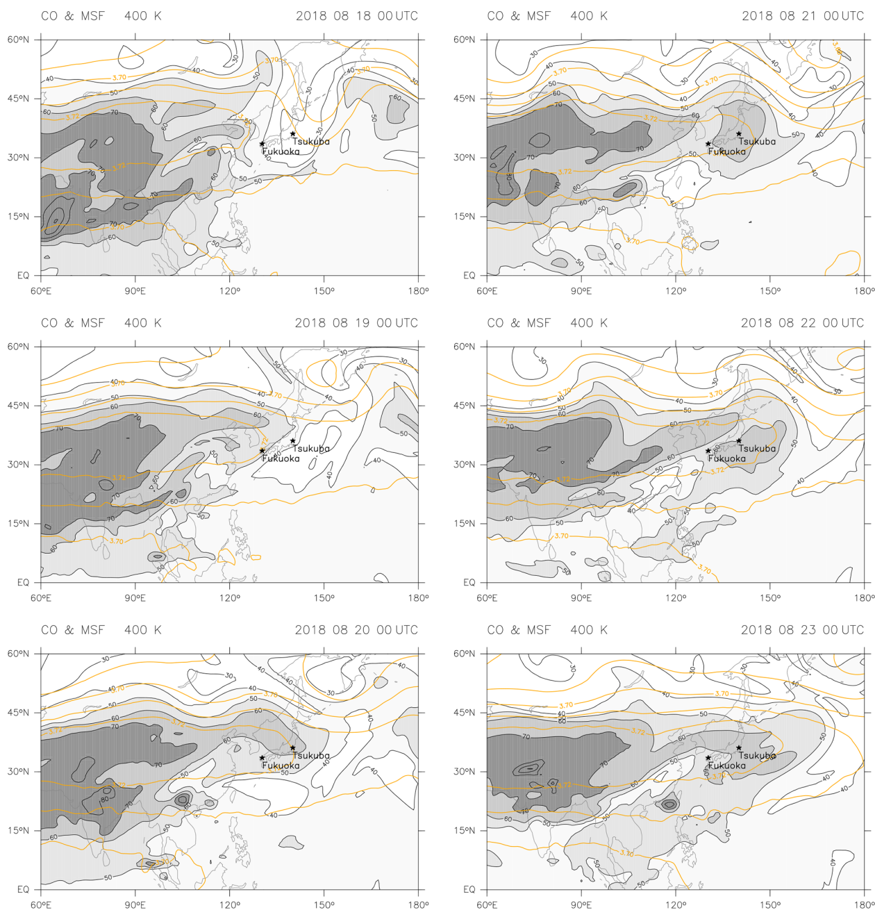
Figure 6. Horizontal distribution of daily instantaneous (00:00 UTC) CO (black contours with grey tone, with intervals of 10 ppbv) and the Montgomery streamfunction (MSF; coloured contours at intervals of 0.01 \times 10^5 \text{ m}^2 \text{ s}^{-2} ) at the 400 K potential temperature level during 18–23 August 2018 (dates indicated at the top right of each plot) using CAMS reanalysis data.
