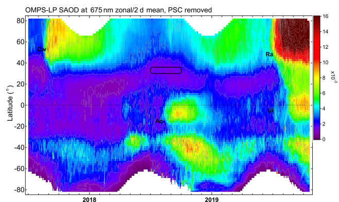
Figure 9. Time–latitude distribution of zonal-mean and 2 d mean lower-stratospheric aerosol optical depth at 675 nm between the tropopause and 21 km of altitude from July 2017 to October 2019, as calculated from OMPS LP satellite data. The tropopause altitude for each OMPS LP profile was provided within the OMPS LP dataset. Signals due to polar stratospheric clouds (PSCs) have been removed. Major events that significantly enhanced NH stratospheric aerosol loading are labelled: Cw, Canadian wildfires in the summer of 2017; Ao, Ambae (Aoba) eruption, Vanuatu (July 2018); Ra, Raikoke eruption, Kuril Islands, Russia (June 2019); Ul, Uluwatu eruption, Papua New Guinea (July, August, and October 2019) (GVP, 2013). The rectangular box indicates the period and location of the lidar measurements; white regions indicate missing measurements.
