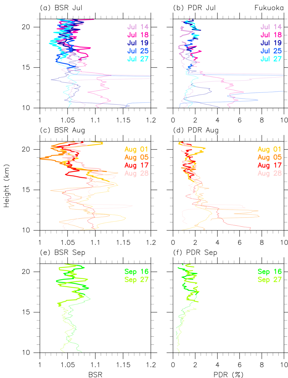
Figure 3. A total of 11 vertical profiles of (a, c, e) the backscattering ratio (BSR) and (b, d, f) particle depolarization ratio (PDR, in %) in (a, b) July, (c, d) August, and (e, f) September 2018 obtained using the lidar system at Fukuoka. Dates and colours are assigned in the legend where, for example, “Jul 14” refers to the night of 14–15 July. The stratospheric portion of the profiles has been thickened using the daily (first) lapse-rate tropopause location information provided by the JMA based on operational 21:00LT radiosonde data taken at the JMA Fukuoka site (at a \sim 4 km distance from the lidar site).
