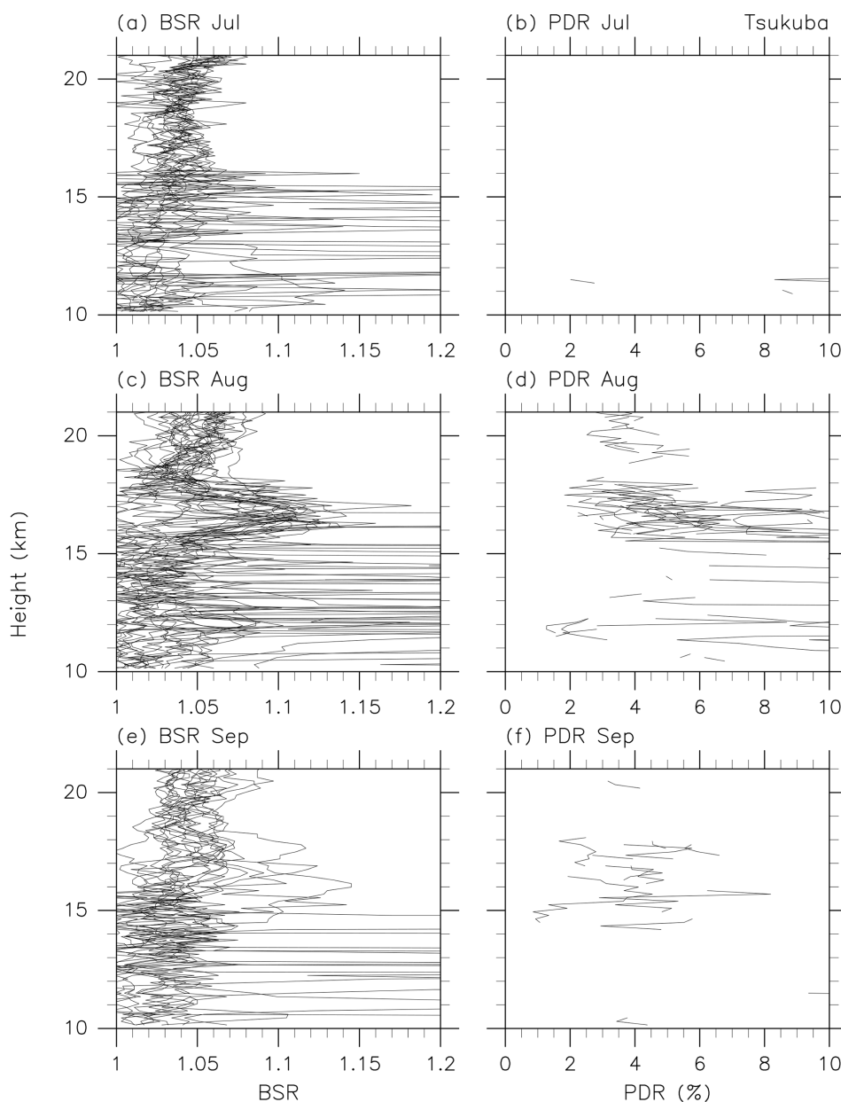
Figure 2. Vertical profiles of (a, c, e) the backscattering ratio (BSR) and (b, d, f) particle depolarization ratio (PDR, in %) in (a, b) July, (c, d) August, and (e, f) September 2018 obtained using the lidar system at MRI, Tsukuba. It is noted that strong and noisy signals in BSR below \sim 15.5 km are due to cirrus clouds.
