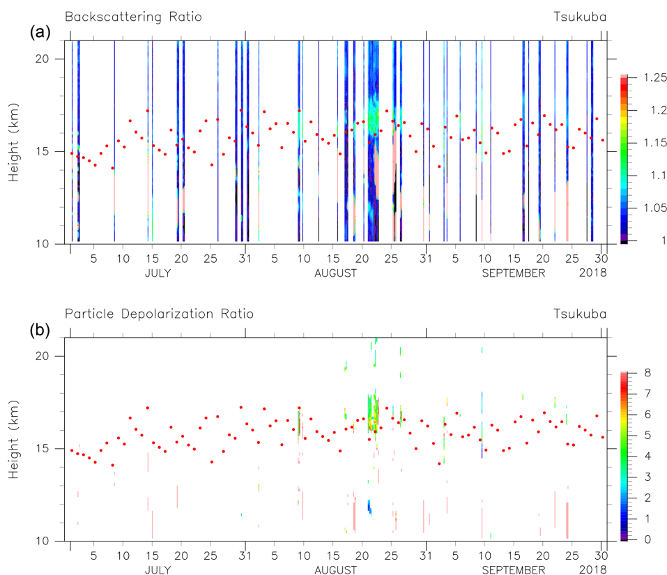
Figure 1. Time–height distributions of (a) the backscattering ratio and (b) particle depolarization ratio (%) during July–September 2018, as measured using the lidar system at MRI, Tsukuba. For each day, four time slots (i.e. 18:00–21:00, 21:00–00:00, 00:00–03:00, and 03:00–06:00 LT) are prepared, with 3 h averaged data filling the slots where thick lower to middle tropospheric clouds do not exist. Red dots indicate the daily (first) lapse-rate tropopause locations determined by the Japan Meteorological Agency (JMA) based on 21:00 LT radiosonde data taken at the JMA Tateno site (which shares the same site as the MRI).
