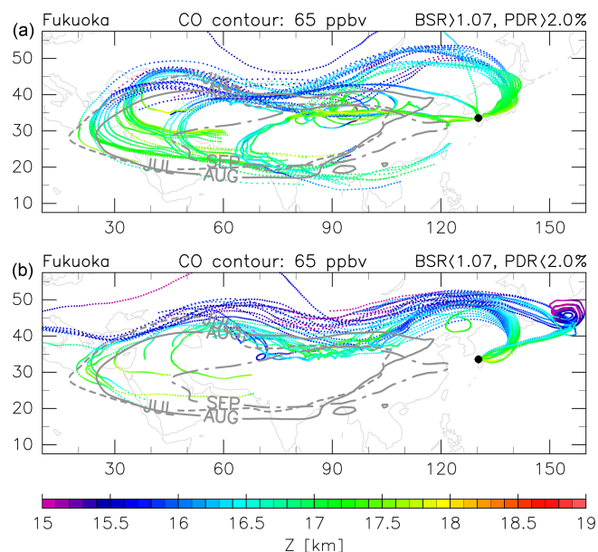
Figure 5. As for Fig. 4, but for trajectories from Fukuoka with (a) 44 and (b) 37 trajectories.
