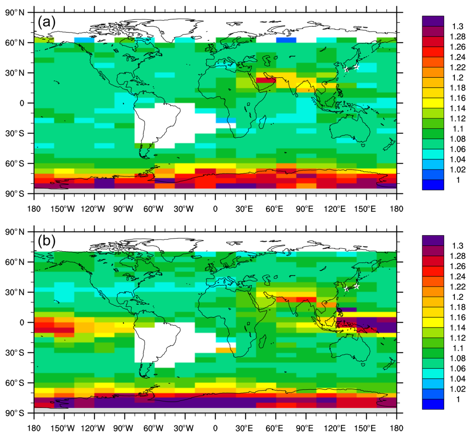
Figure 10. Monthly mean horizontal distribution of attenuated scattering ratio at 17.042 km observed with the CALIOP satellite instrument in (a) July 2018 and (b) August 2018. Spatial bins are 5° in latitude, 20° in longitude, and 900 m in altitude. Clouds and PSCs have been removed (Sect. 2.2). It is noted that the CALIOP attenuated scattering ratio is defined as the ratio of the measured attenuated backscatter coefficients and the attenuated backscatter coefficients calculated from the molecular model, and its valid range is from 0.60 to 25.00. The two lidar station locations are marked with white stars. White regions indicate missing measurements (see Noel et al., 2014, for the data missing over the South Atlantic region).
