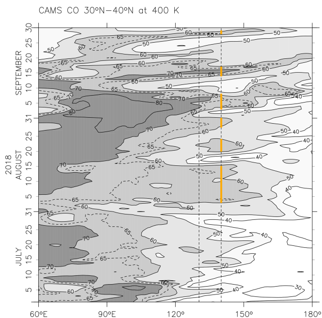
Figure 7. Longitude–time distribution of the daily averaged CO concentration at 400 K potential temperature averaged over 30–40° N using CAMS reanalysis data. The contour interval is 10 ppbv, with 65 ppbv contours added (dotted). Vertical dotted lines indicate the locations of the two lidar sites in Fukuoka (130.36° E) and Tsukuba (140.1° E); furthermore, the periods along the longitude of Tsukuba when the CO concentration was \geq 60 ppbv (i.e. 3–15, 20–24, and 28–31 August, as well as 3–8, 14–17, and 28–29 September) are shown as orange line segments.
