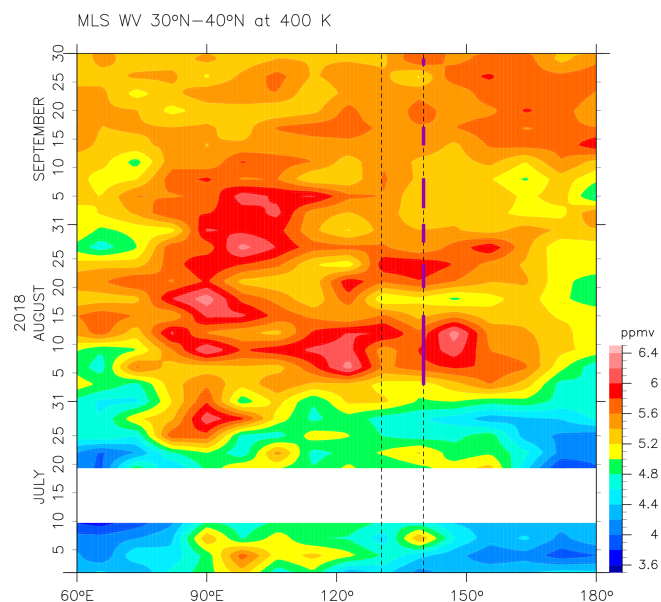
Figure 8. As for Fig. 7, but for water vapour (in ppmv) at 400 K measured with the satellite MLS instrument. Data for the 30–40° N region have been aggregated into 3 d and 8° longitude bins, each constituting about 10 individual data points. The white region indicates missing measurements. The purple line segments are the same as the orange ones in Fig. 7.
