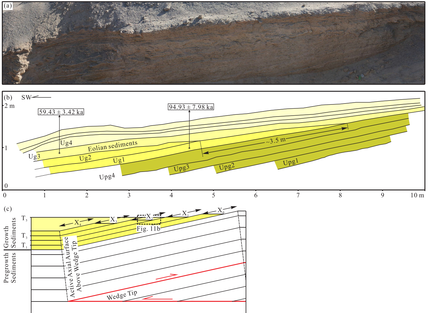
Figure 11. (a) A trench photo of the folded sediments produced by southwest-vergent thrusting of the lower SZG wedge structure. See location in Figure 8. (b) Reinterpretation of the trench. Folded Ugl and Ug2 represent two thrusting events. (c) A simplified model of a terraced hillslope formed on the front limb of a buried wedge thrust structure (modified from Mueller & Suppe, 1997). Folding events occur at times T n , defined by overlapped sediment packages. Terraces were developed above the sediments deposited above the strata that had already been folded through an active axial surface. Limb widening by each event is denoted by X n , which is measured parallel to bedding between outer terrace edges.
