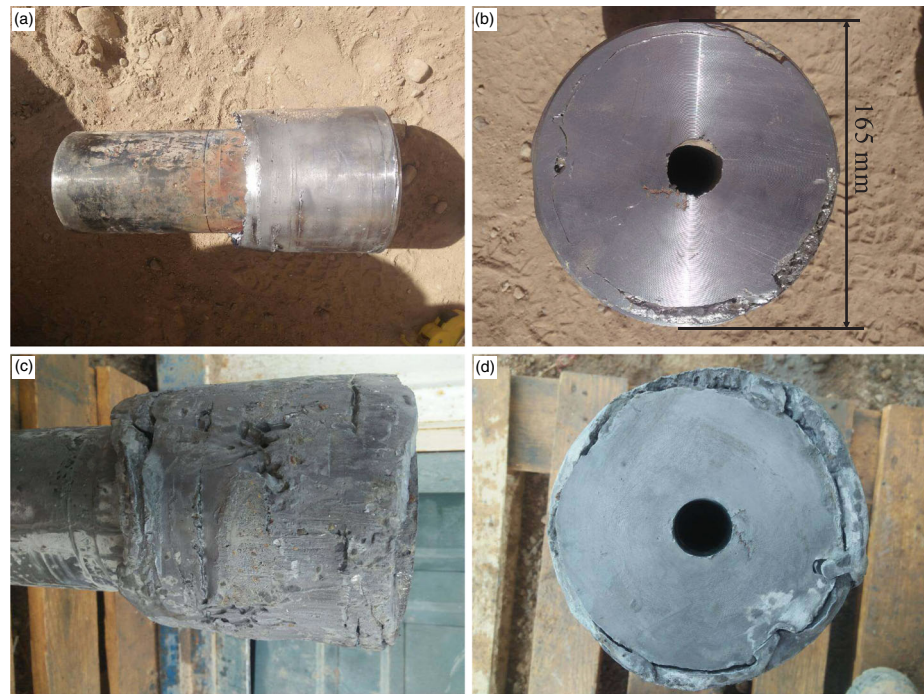
Figure 4. Photos of the lead seal before being put into (a and b) and after being pulled out (c and d) from borehole H4-3-414. The diameter of the lead seal bottom is 165 mm and the inner diameter of the casing pipe is 166.63 mm. The side face of the lead seal has scratches, but no imprint exists in its bottom surface, revealing that the coseismic slip at this borehole site is more than 196.85 mm, the outer diameter of the casing pipe.
