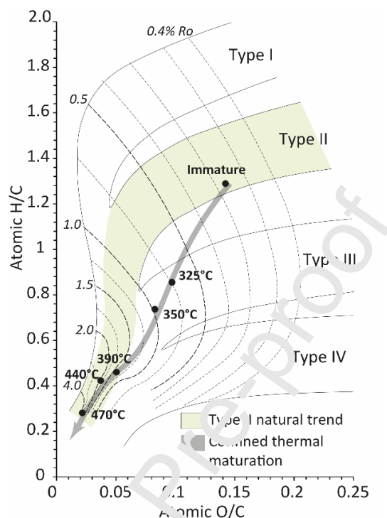
Figure 2. Evolution of H/C and O/C atomic ratios with increasing maturation temperature.
